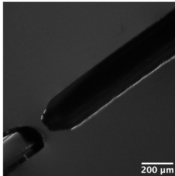
Supplementary Figure 1. Image of CSFOE (lower left) photoacoustic signal measurement using a needle hydrophone (upper right) by a microscope with 10X objective.
