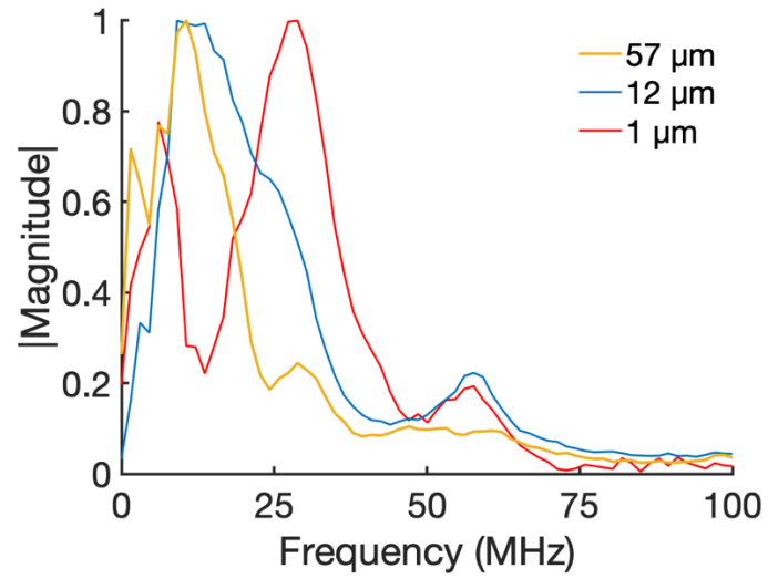
Supplementary Figure 2. Frequency analysis of optoacoustic signal generated by different CSFOEs with different candle soot layer thickness.
