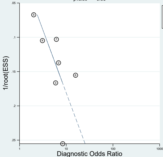
Fig. S3. Deeks' funnel plot asymmetry test of the diagnosis of quadriceps femoris thickness on ultrasound for sarcopenia
