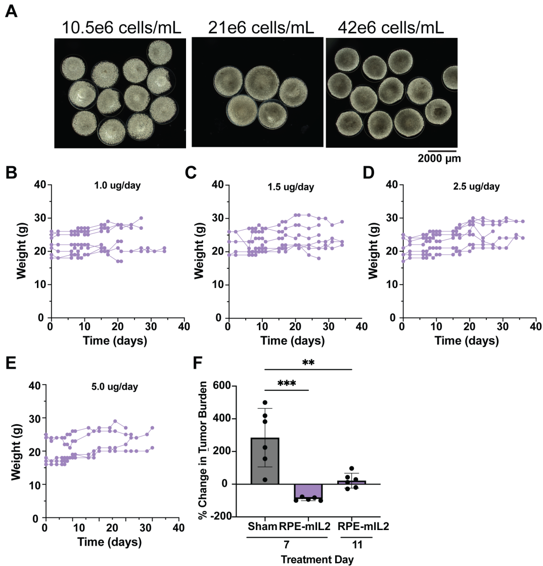
Supplemental Figure 1. Dose dependent anti-tumor effects of RPE-mIL2 administration. A , Darkfield images of RPE-mIL2 cells encapsulated at 10.5, 21, and 42e6 cells/mL of SLG20 alginate. Images acquired at 2X magnification; scale bar is 2000 \mu m. B-E , Plots tracking the weight of individual mice in each of the RPE-mIL2 treatment groups over the course of treatment. F , Percent change in tumor burden for sham and RPE-mIL2 groups treated at 7 days compared to mice treated at day 11.
