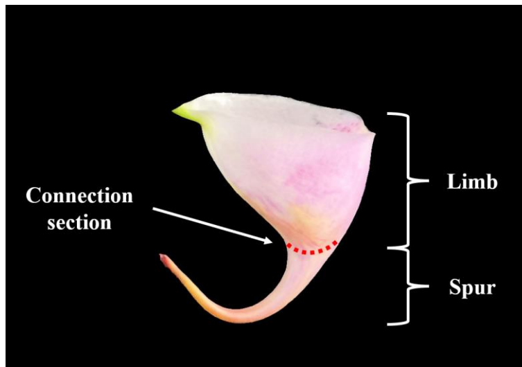
Figure S5 The labellum of I. uliginosa . The funnel-shaped part is the limb, and the curved tubular part is the spur, dashed red line indicates the connection section.
