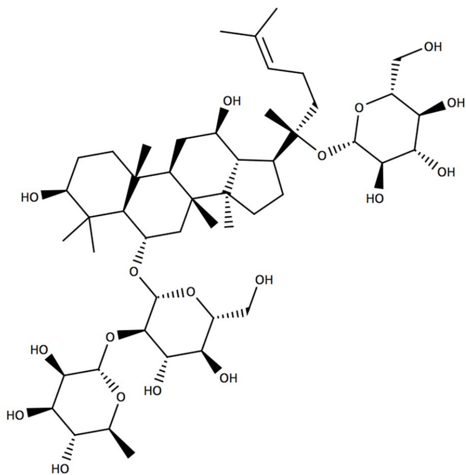
Figure 1f. Ginsenoside Re.
