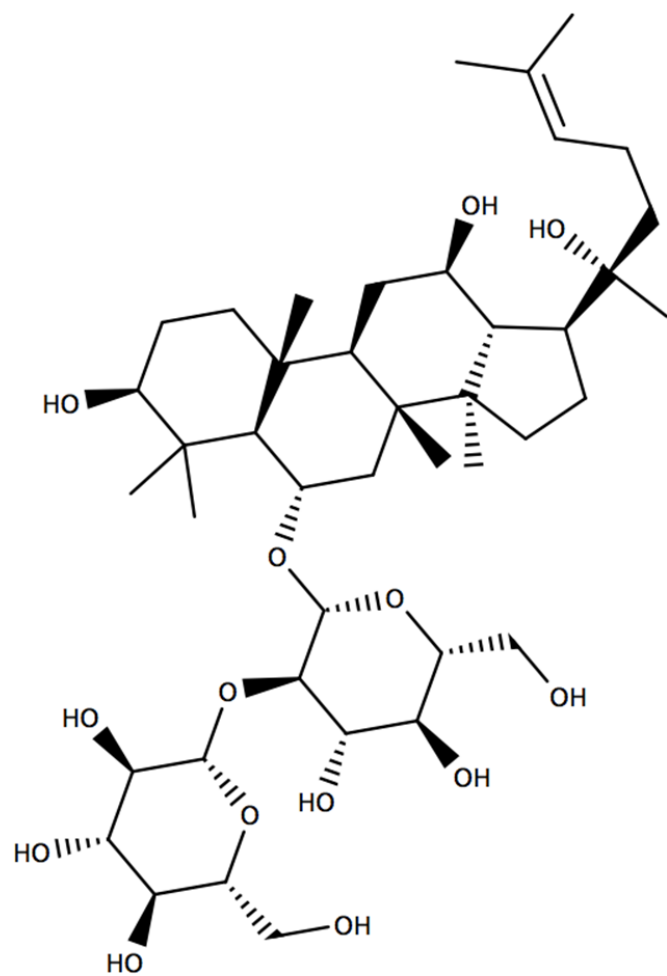
Figure 1g. Ginsenoside Rf.
