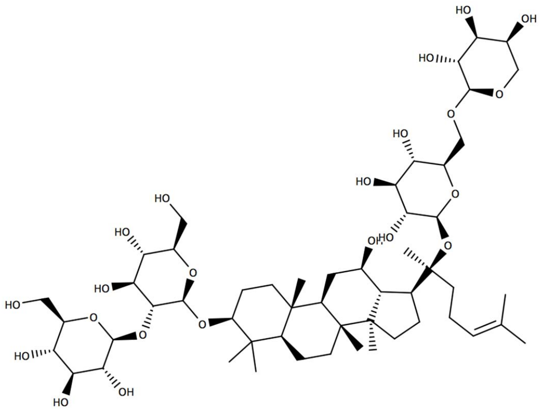
Figure 1b. Ginsenoside Rb2.
