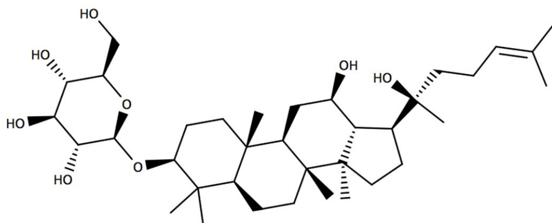
Figure 1n. 20(R)-Ginsenoside Rh2.
