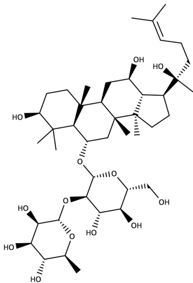
Figure 1j. 20(R)-Ginsenoside Rg2.
