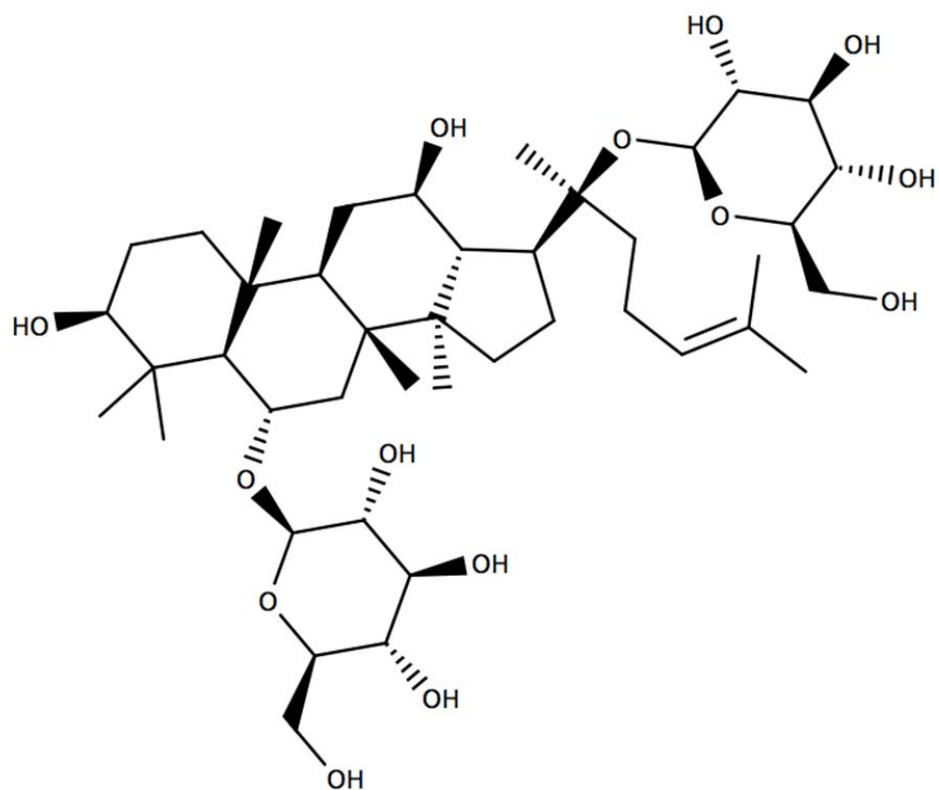
Figure 1h. Ginsenoside Rg1.
