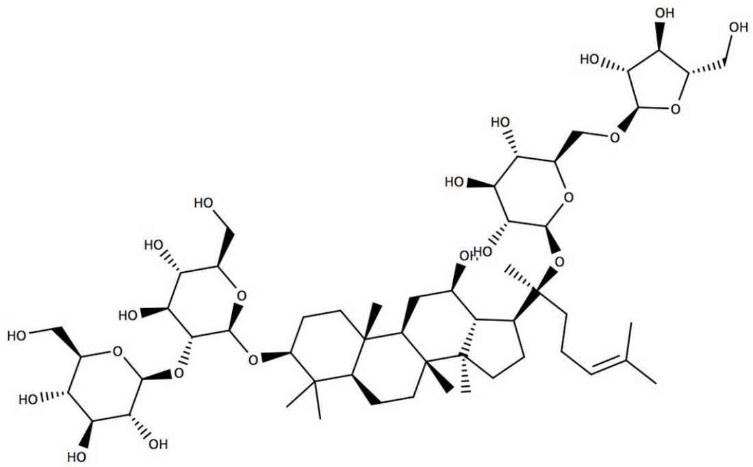
Figure 1d. Ginsenoside Rc.
