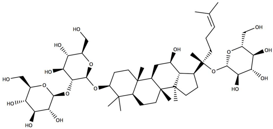
Figure 1e. Ginsenoside Rd.
