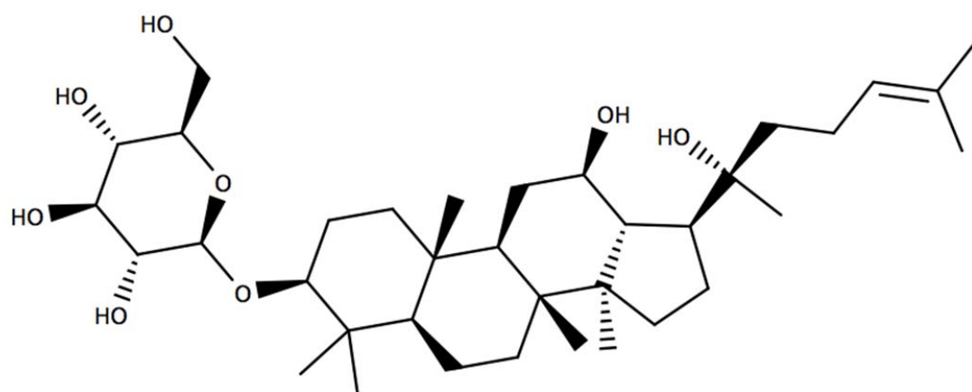
Figure 1m. 20(S)-Ginsenoside Rh2.
