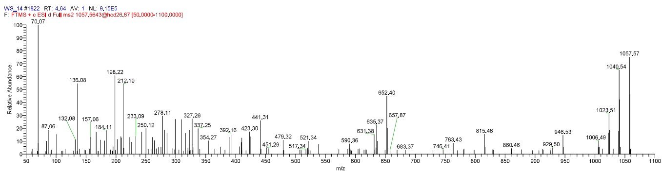
Figure S3 MS/MS spectra of compounds 4 and 5
