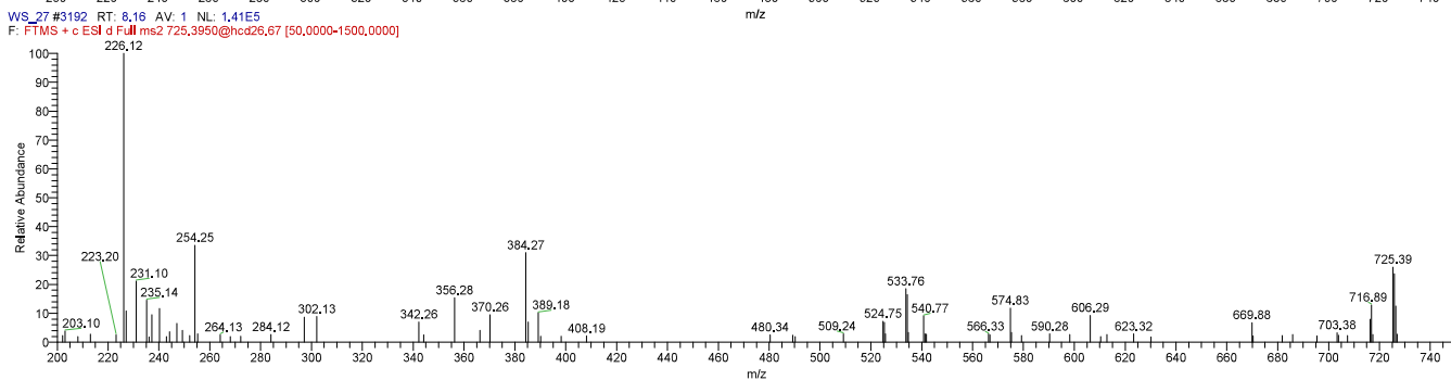
Figure S5 MS/MS spectra of compounds 7, 9 and 10
