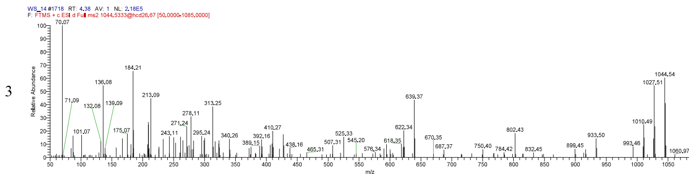
Figure S2 MS/MS spectra of compounds 2 and 3
