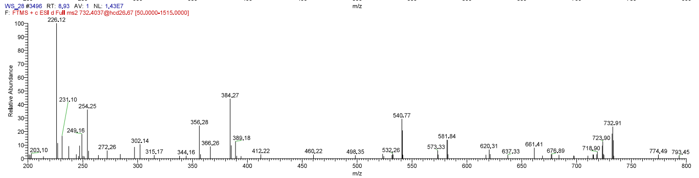
Figure S6 MS/MS spectra of compounds 8, 12 and 13
