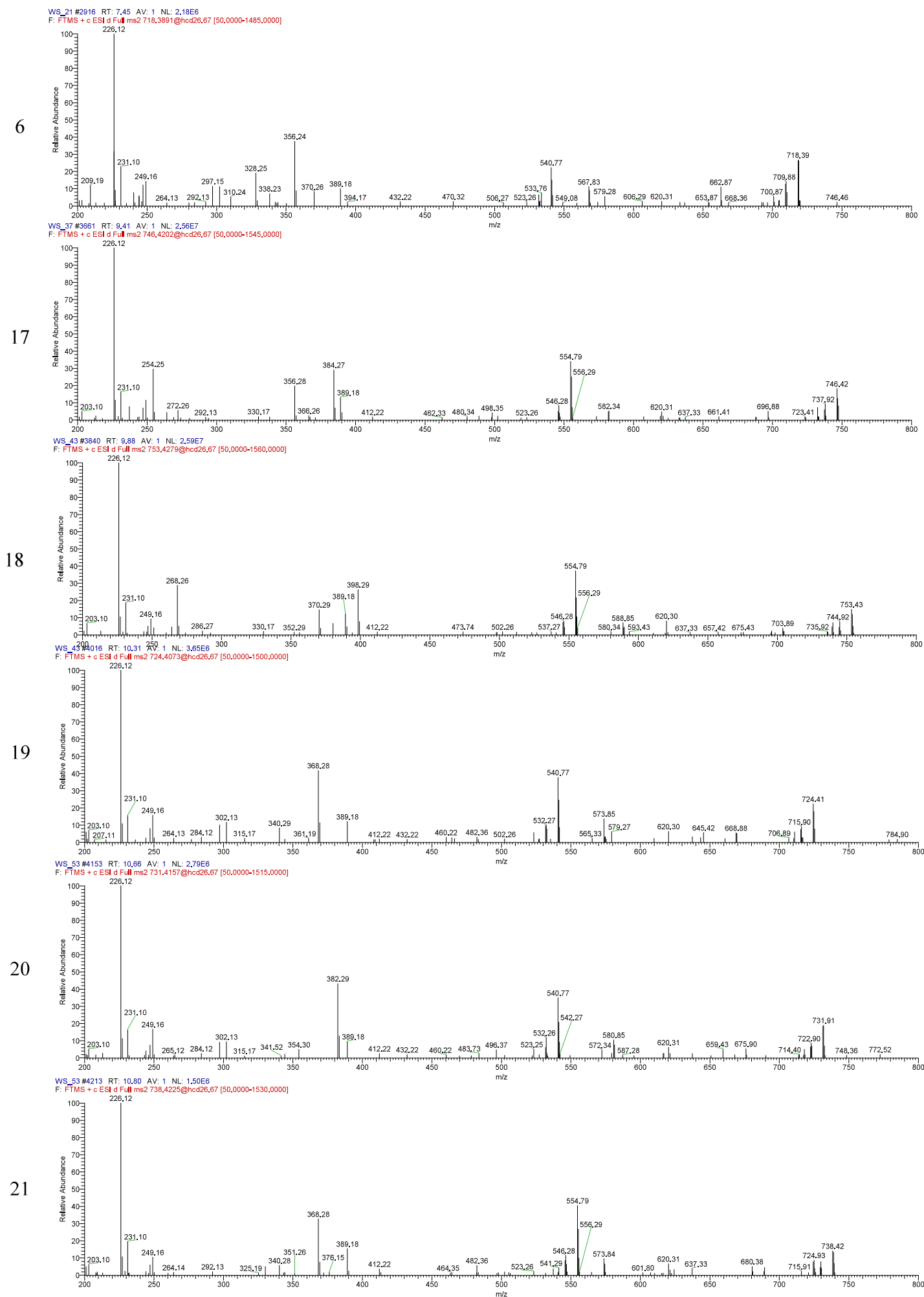
Figure S4 MS/MS spectra of compounds 6, 17, 18, 19, 20 and 21
