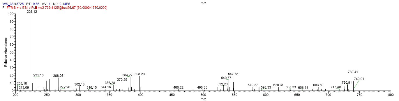
Figure S7 MS/MS spectra of compounds 11, 14, 15 and 16
