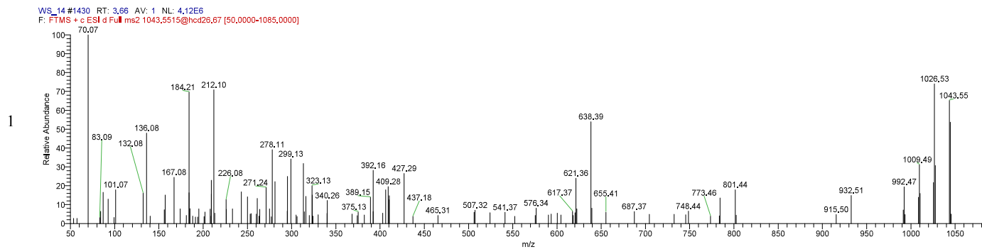
Figure S1 MS/MS spectra of compounds 1
