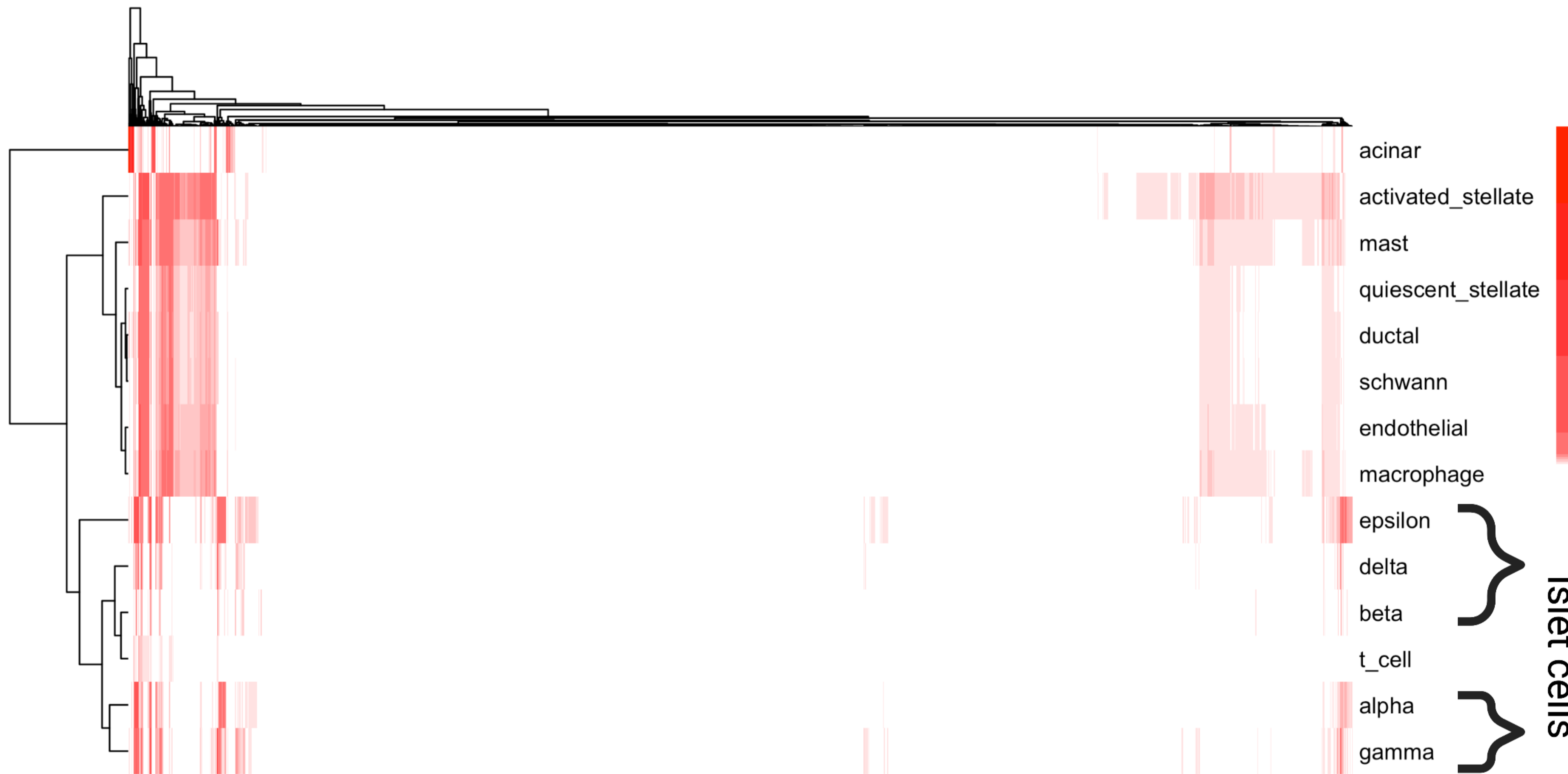
nn-PRRR coefficients
