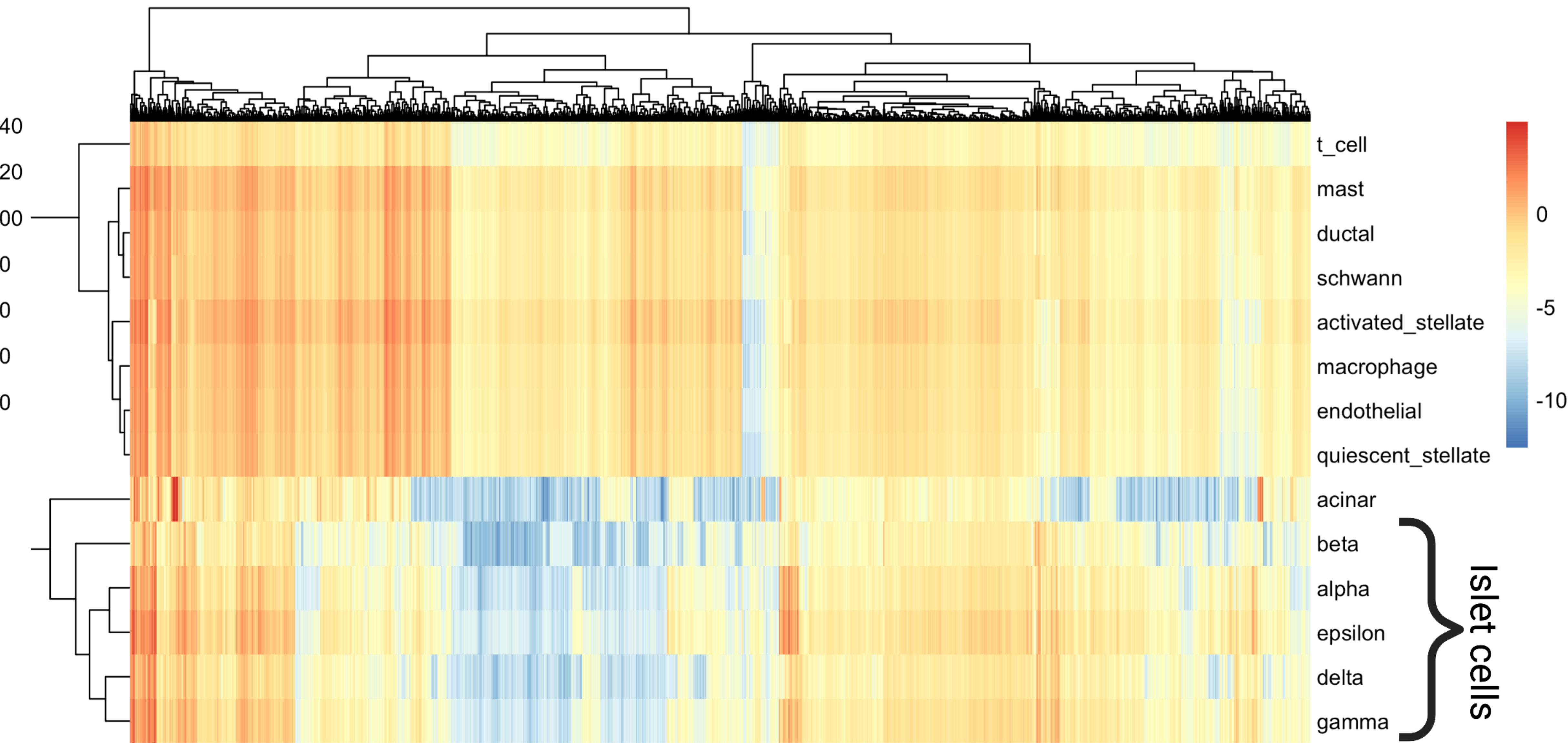
nn-PRRR coefficients
