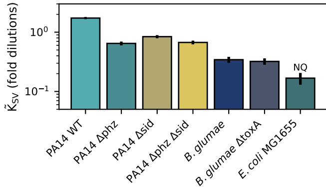
Supernatants + RTDP
