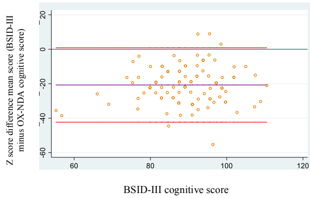
Figure S4 Bland-Altman Plots
