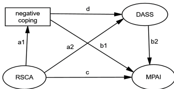
Figure 1 Hypothesized model
