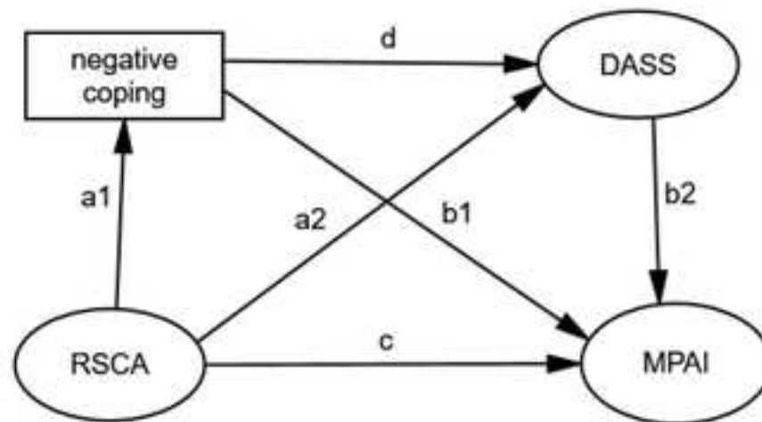
Figure 1 Hypothesized model
