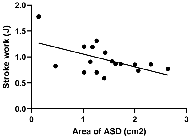
Stoke work
