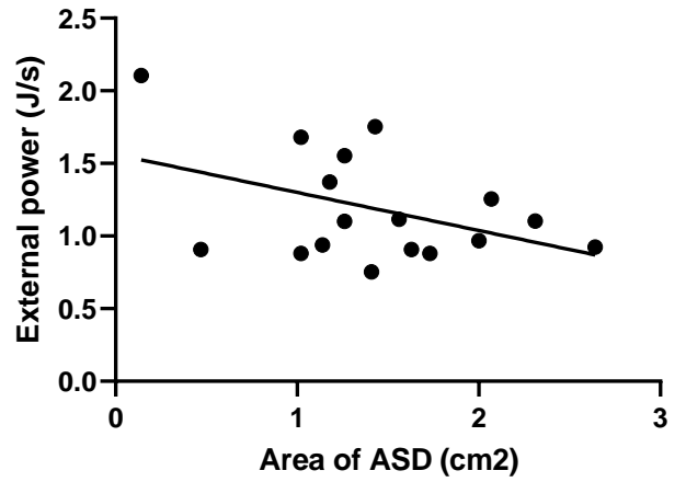
External power
