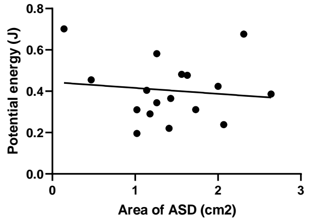
Potential energy
