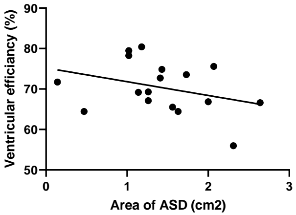
Ventricular efficiency
