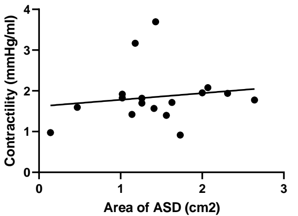
Contractility
