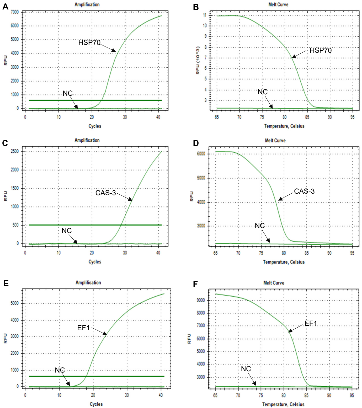
Supplementary Fig. 1. Amplification and melting curves from qRT-PCR of heat shock protein-70 (HSP70) (A, B), caspase-3 (CAS-3) (C, D), and elongation factor-1 (EF1) (E, F) genes. NC, negative control.
