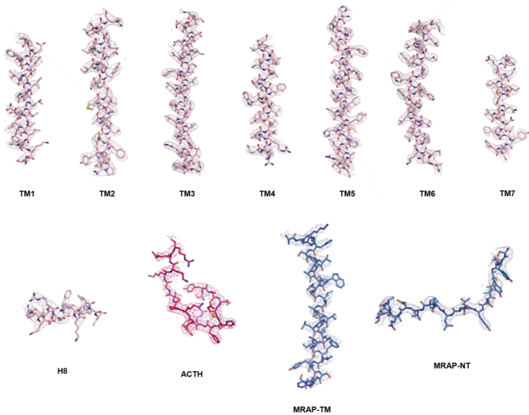
Supplementary information, Fig. S2 Representative segments of model and cryo-EM density. Model segments with corresponding map density of transmembrane helices and helix 8 of MC2R; ACTH and calcium ion; transmembrane helix and N-terminus of MRAP1. All the cryo-EM densities are shown in PyMOL and contoured at 6 sigma.
