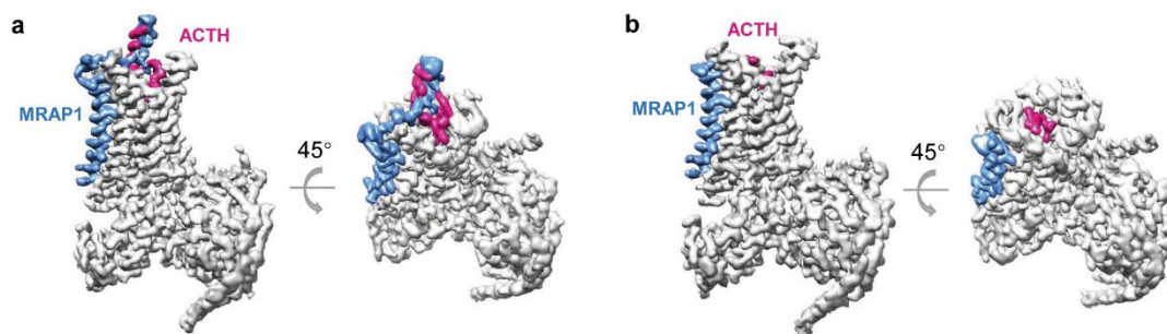
Supplementary information, Fig. S8 Representation of densities of two states after focused 3D classification. a. Density of the integrated ACTH-MC2R-G s -MRAP1 structure in two different views. b. Density of the loose ACTH-MC2R-G s -MRAP1 structure in two different views. Deep pink color shows the ACTH density in (a) or presumable ACTH density in (b), blue color shows the MRAP1 density in both maps.
