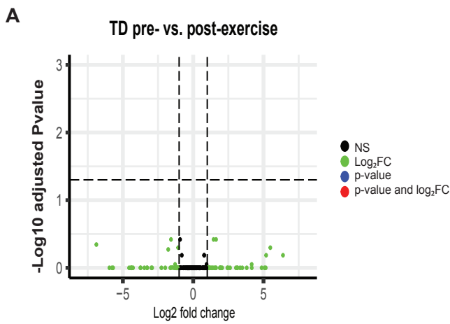
Supplementary Figure 2 – Volcano plots illustrating differences in EV cargo after exercise in (A) typically developed (TD) and (B) cerebral palsy (CP) individuals. Each point on the scatter plot represents a microRNA where its position on the x-axis corresponds to the average log 2 -fold change after exercise. The position on the y-axis corresponds to log 10 P value of its differential expression after adjustment for false discovery rate.
