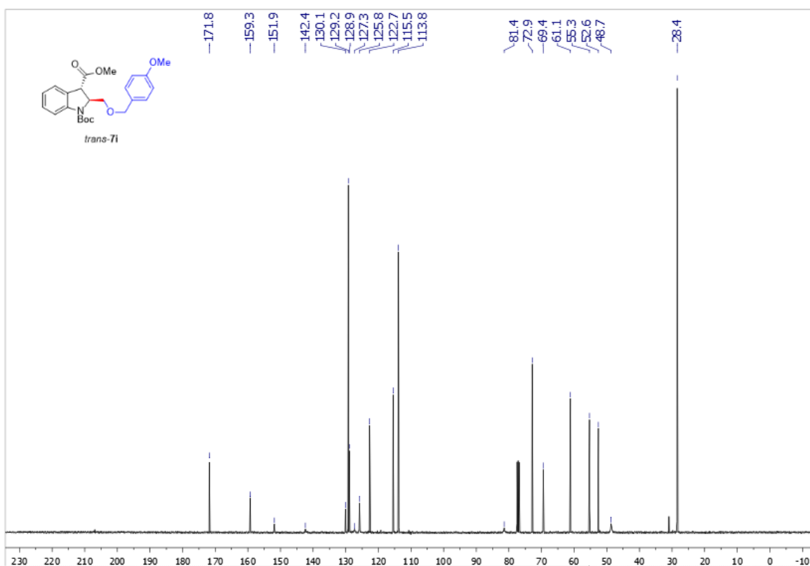
Supplementary Figure 163. 13 C NMR spectra of trans -7i
