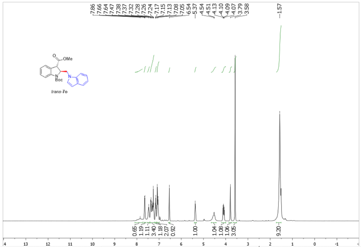
Supplementary Figure 174. 1 H NMR spectra of trans -7o
