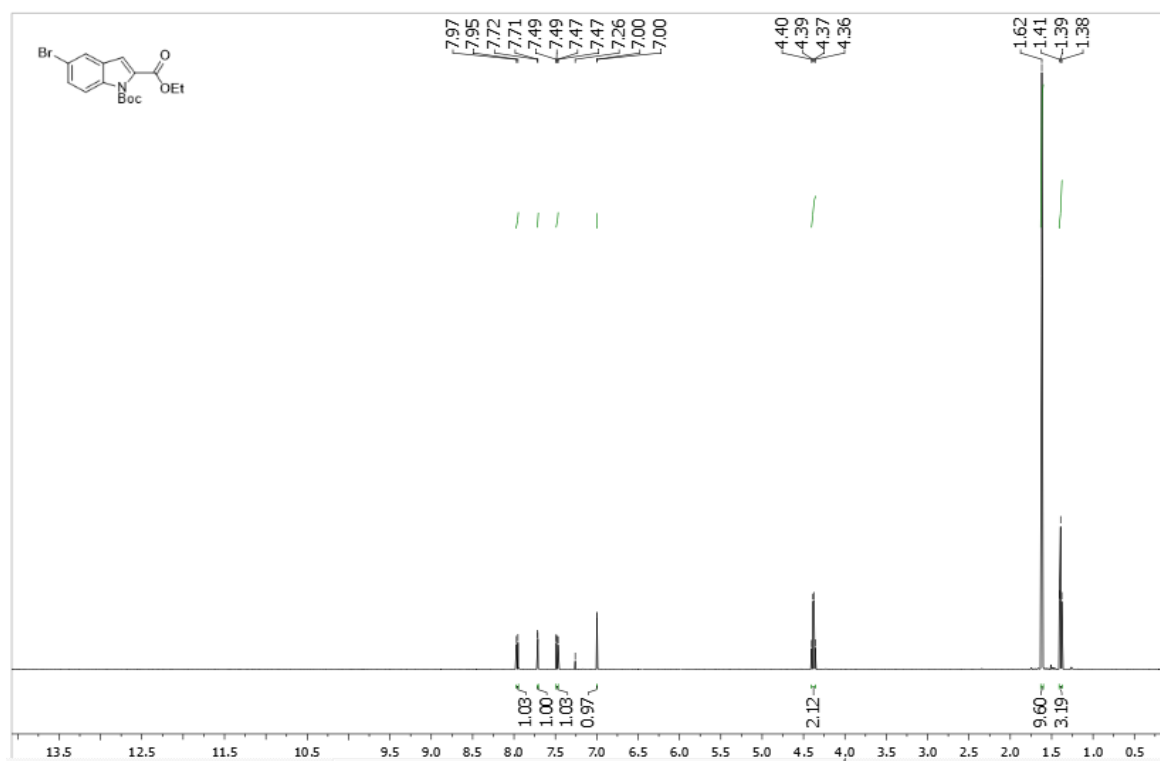
Supplementary Figure 21. ^1\text{H} NMR spectra of 1r
