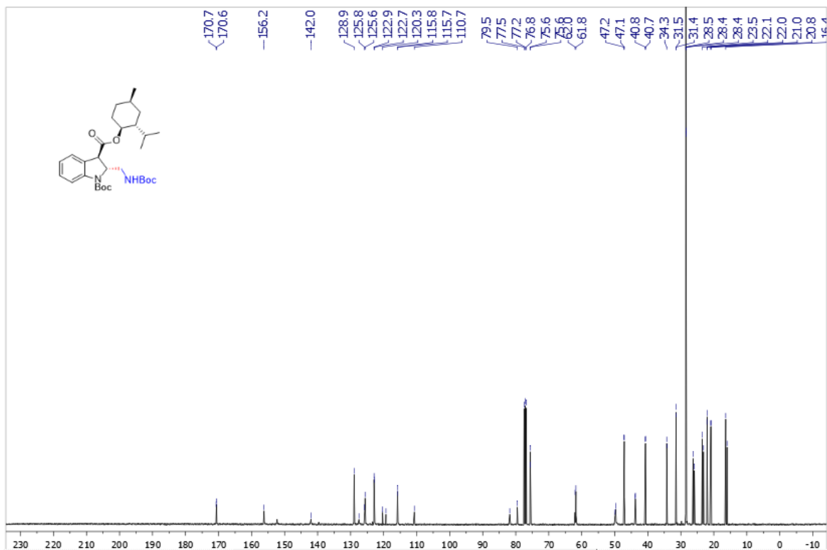
Supplementary Figure 136. ^{13}\text{C} NMR spectra of trans -3as
