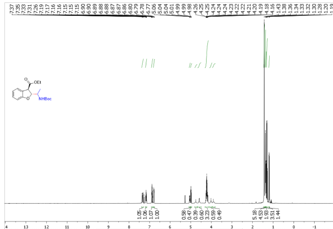
Supplementary Figure 85. ^1\text{H} NMR spectra of trans -3t
