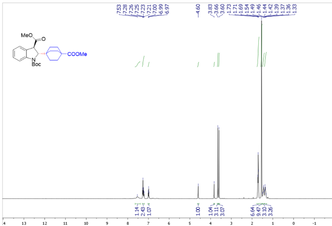
Supplementary Figure 125. ^1\text{H} NMR spectra of trans -3an
