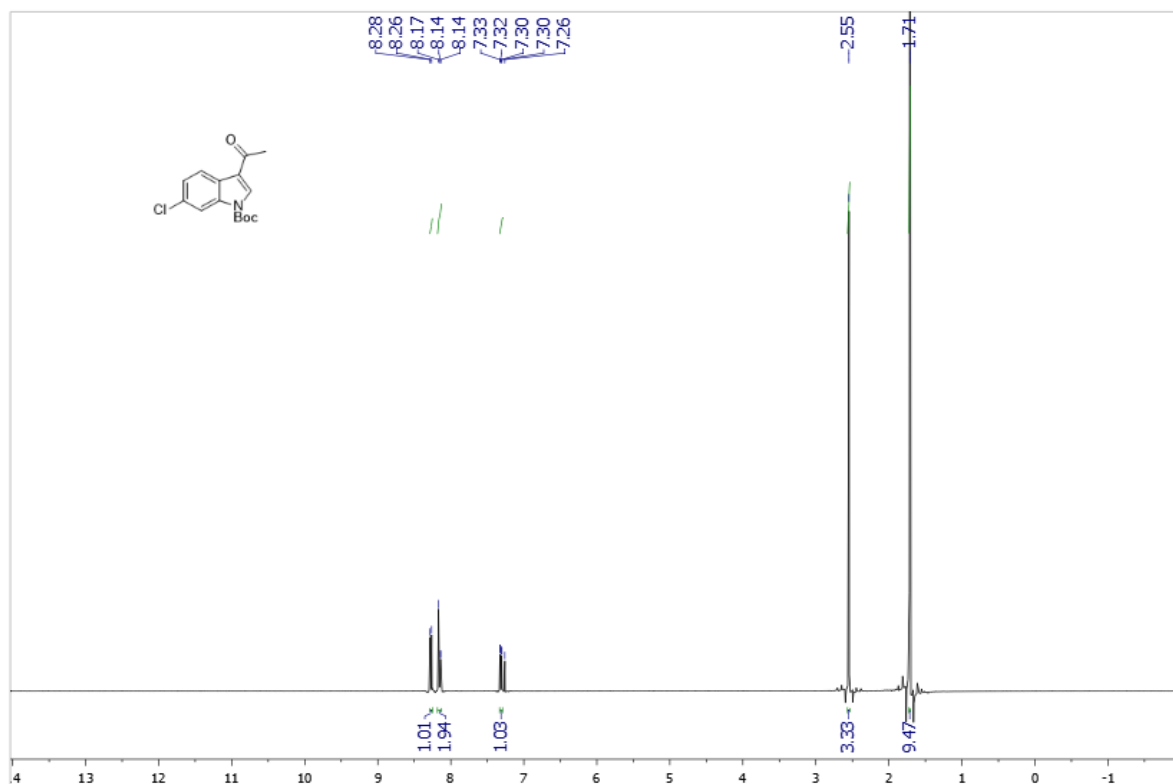
Supplementary Figure 15. ^1\text{H} NMR spectra of 1l
