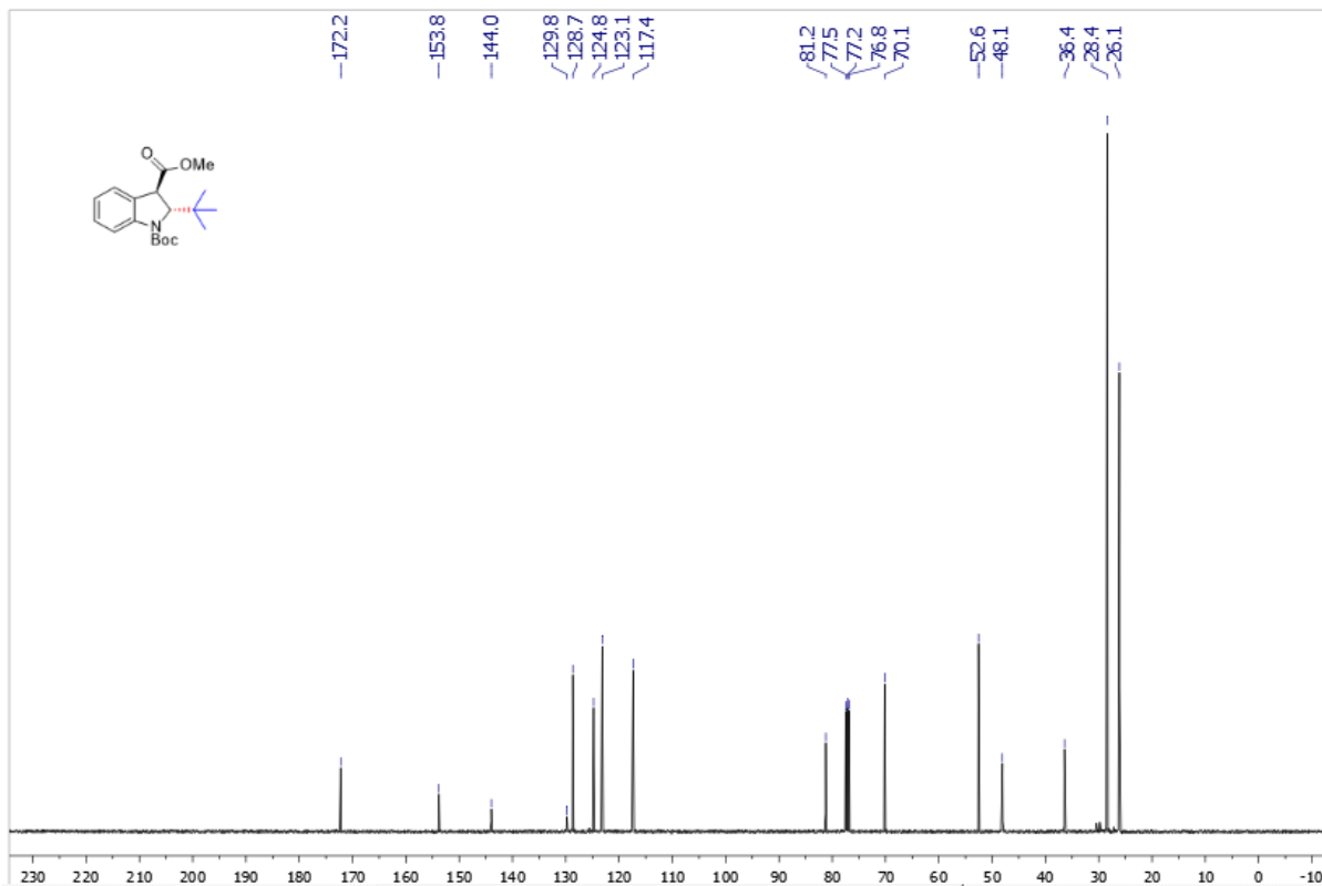
Supplementary Figure 122. ^{13}\text{C} NMR spectra of trans -3al
