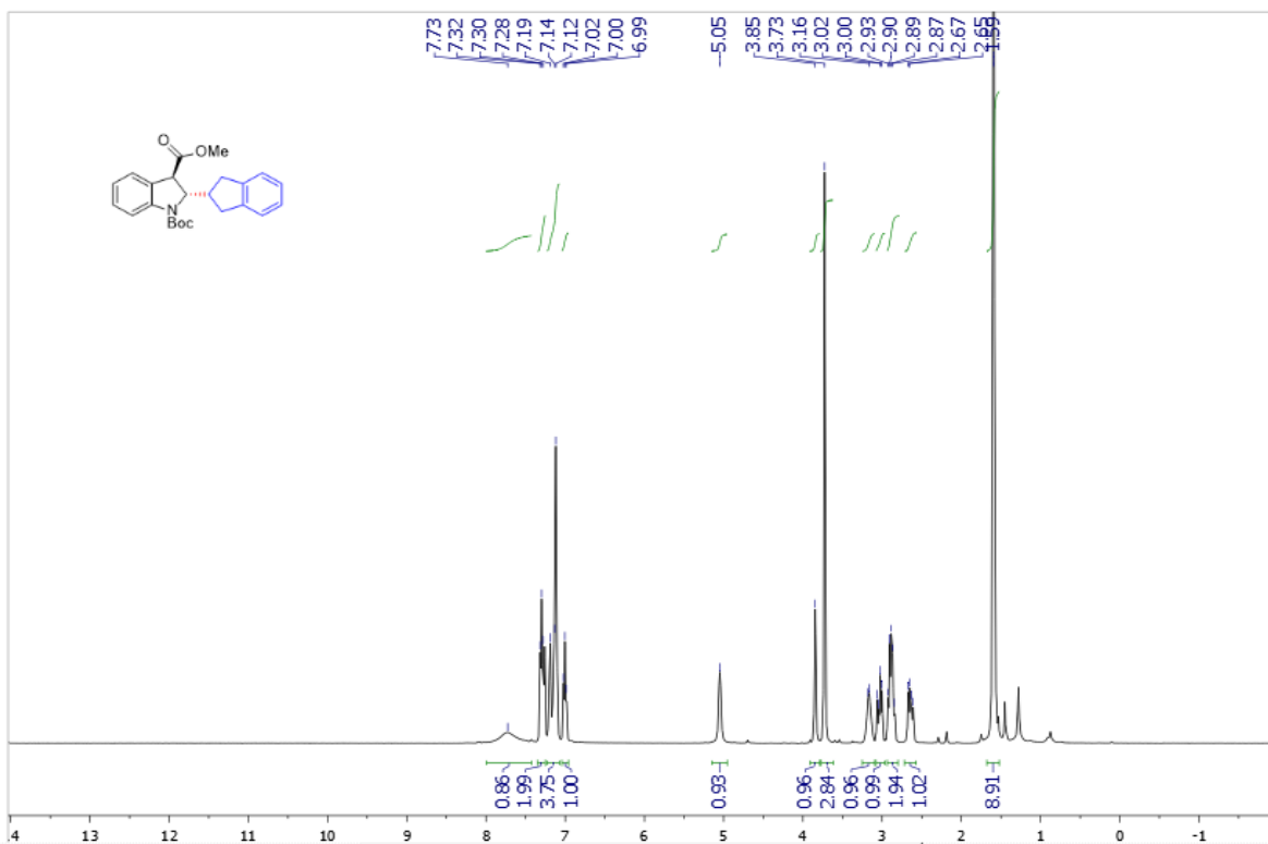
Supplementary Figure 119. ^1\text{H} NMR spectra of trans -3ak
