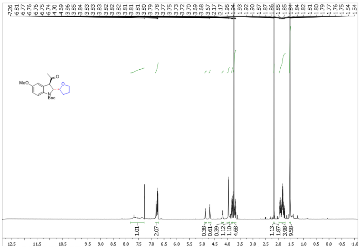
Supplementary Figure 71. ^1\text{H} NMR spectra of trans -3n
