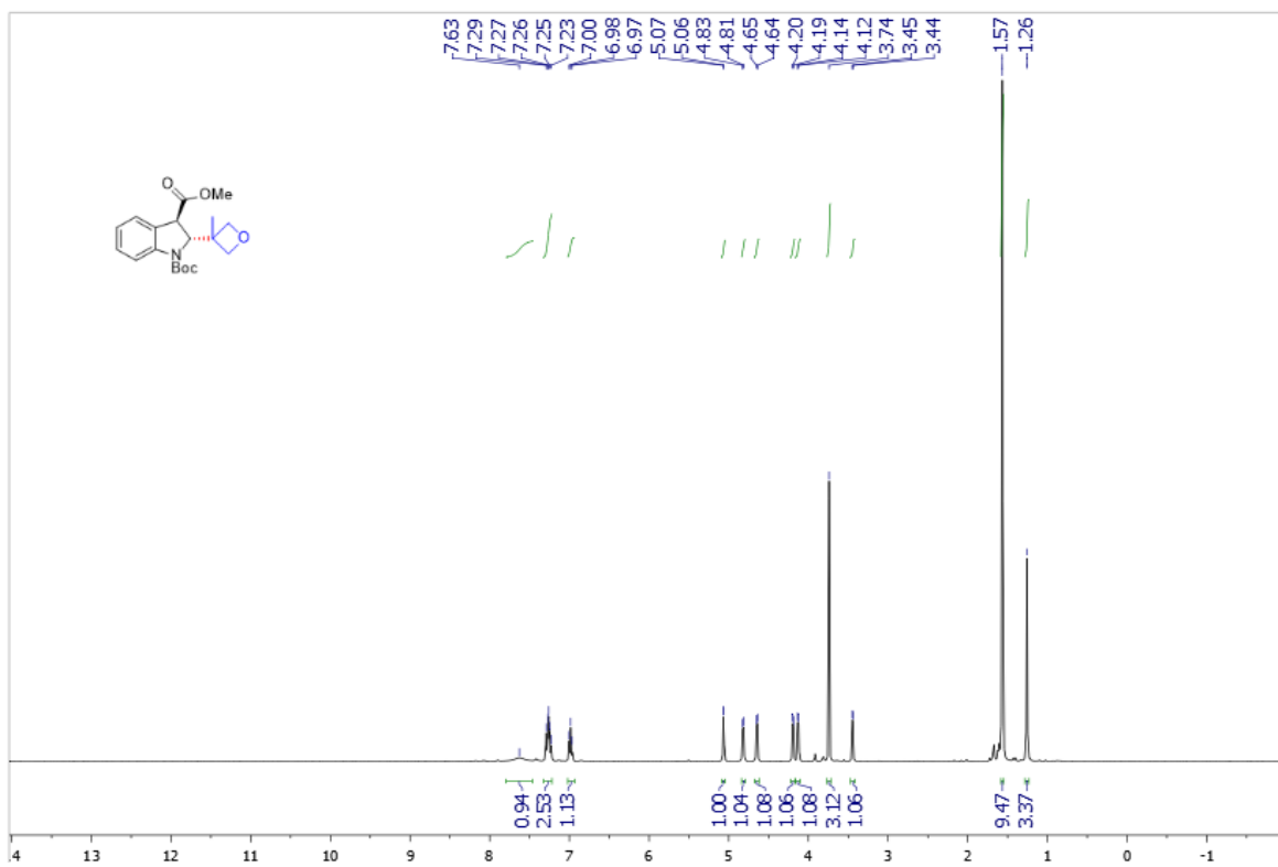
Supplementary Figure 127. 1 H NMR spectra of trans -3ao
