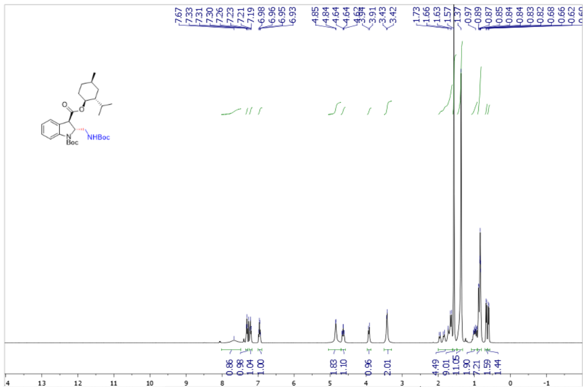
Supplementary Figure 135. ^1\text{H} NMR spectra of trans -3as
