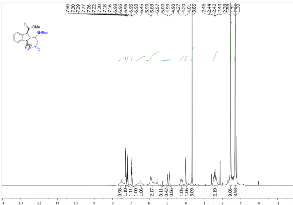
Supplementary Figure 99. 1 H NMR spectra of trans -3aa
