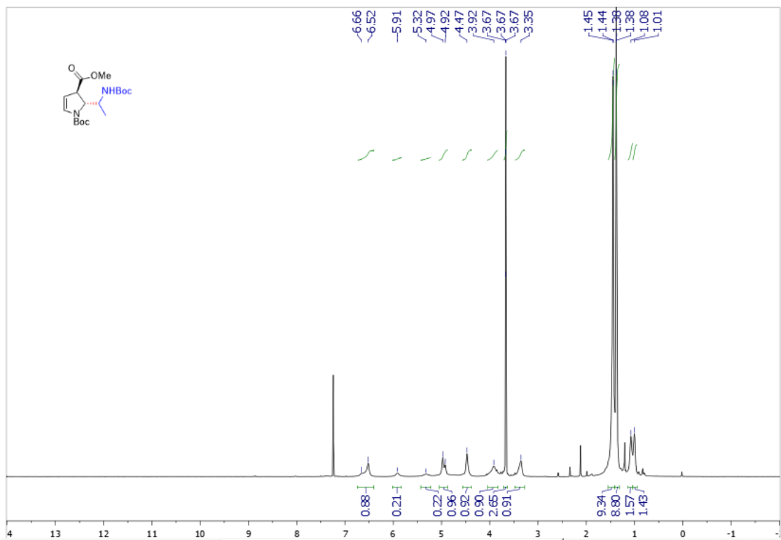
Supplementary Figure 83. ^1\text{H} NMR spectra of trans -3s
