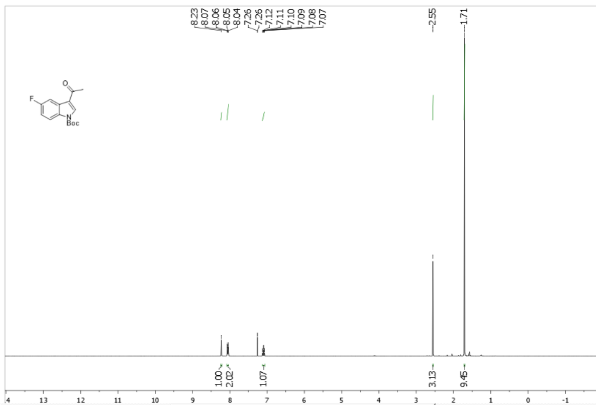
Supplementary Figure 17. ^1\text{H} NMR spectra of 1m
