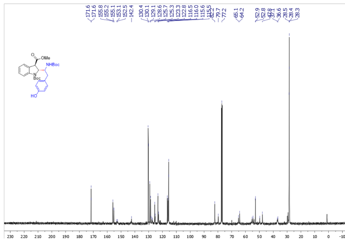
Supplementary Figure 96. 13 C NMR spectra of trans -3y
