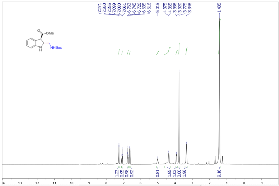
Supplementary Figure 148. ^1\text{H} NMR spectra of trans -4k
