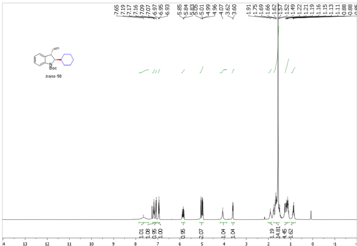
Supplementary Figure 189. ^1\text{H} NMR spectra of trans -10
