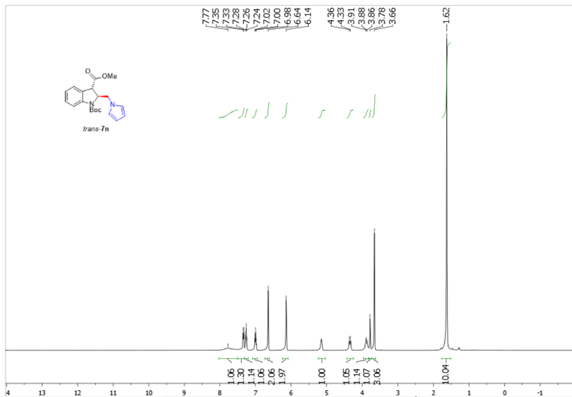
Supplementary Figure 172. ^1\text{H} NMR spectra of trans-7n
