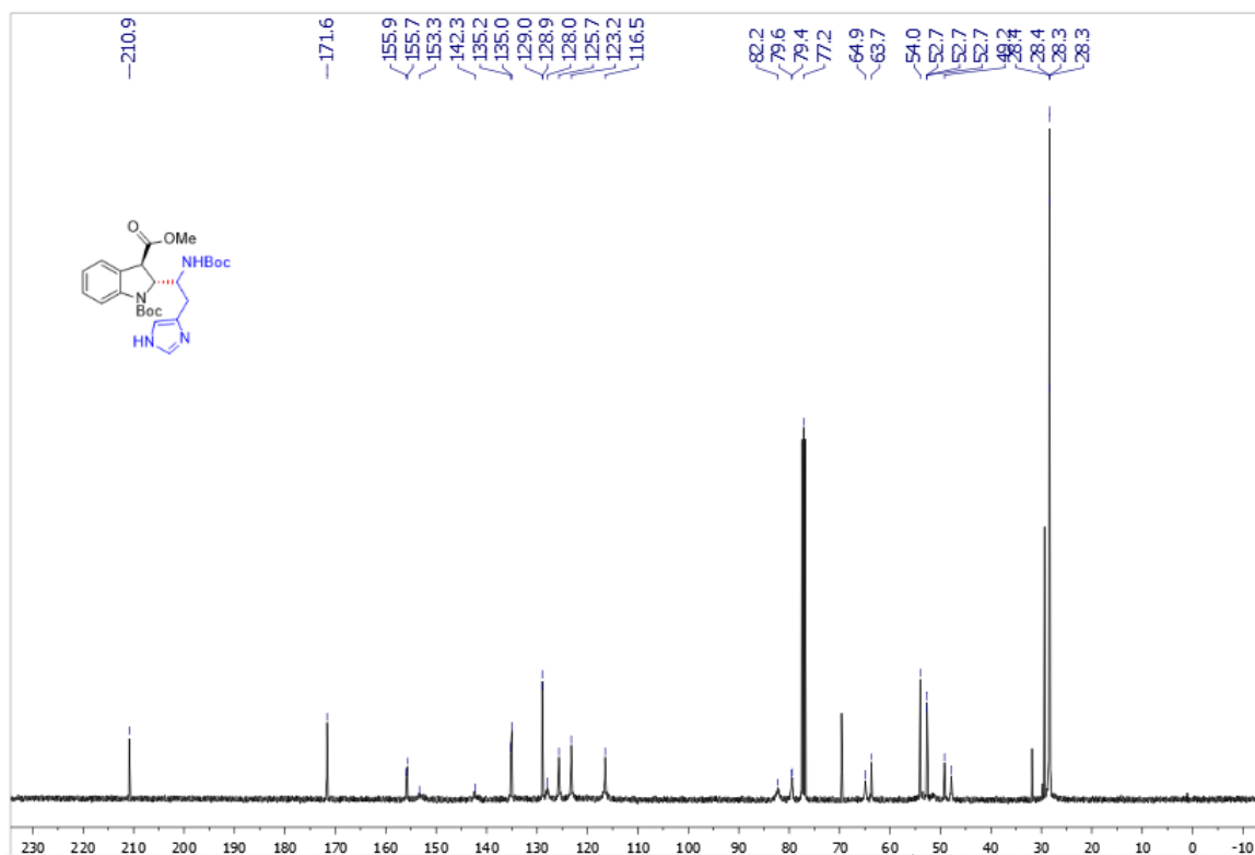
Supplementary Figure 98. 13 C NMR spectra of trans -3z
