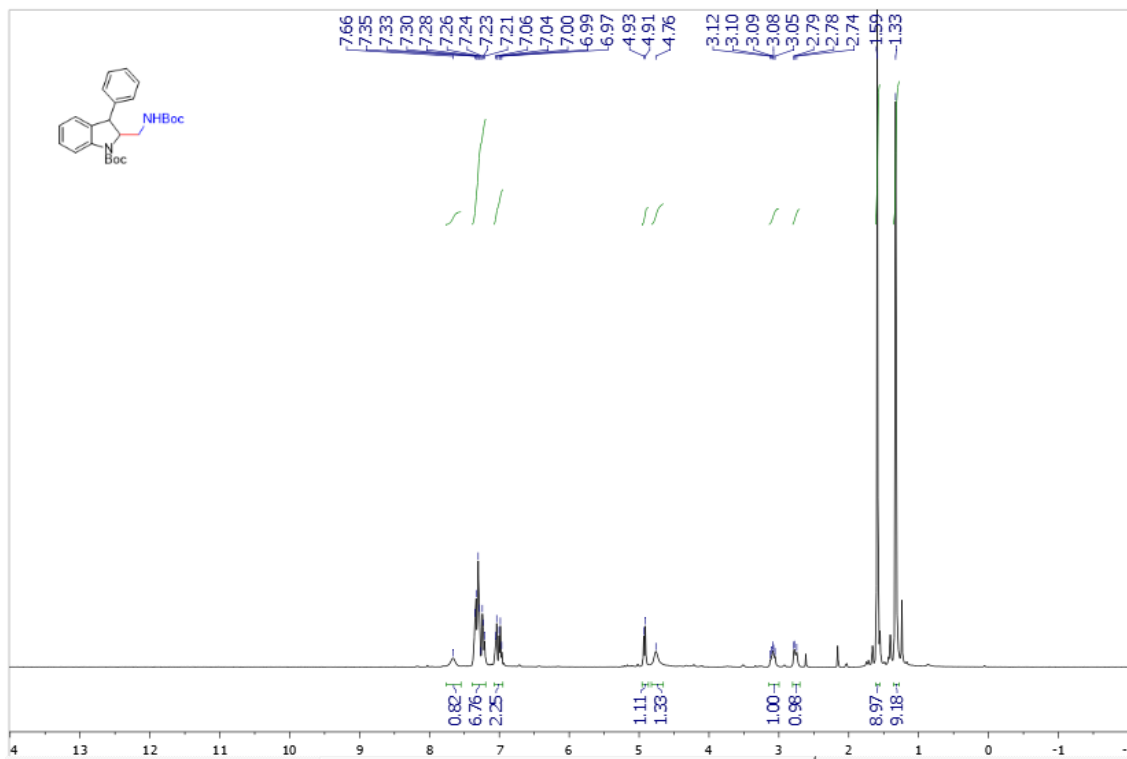
Supplementary Figure 75. 1 H NMR spectra of 3p-isomer-a
