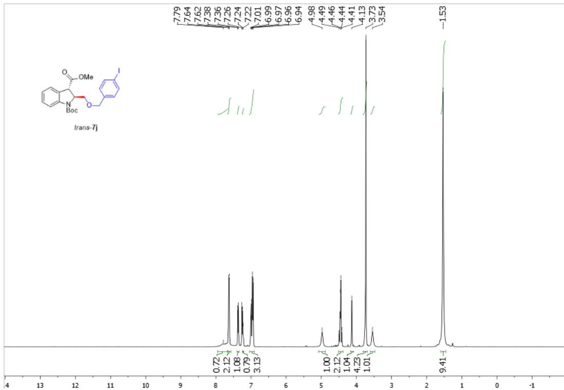
Supplementary Figure 164. 1 H NMR spectra of trans -7j
