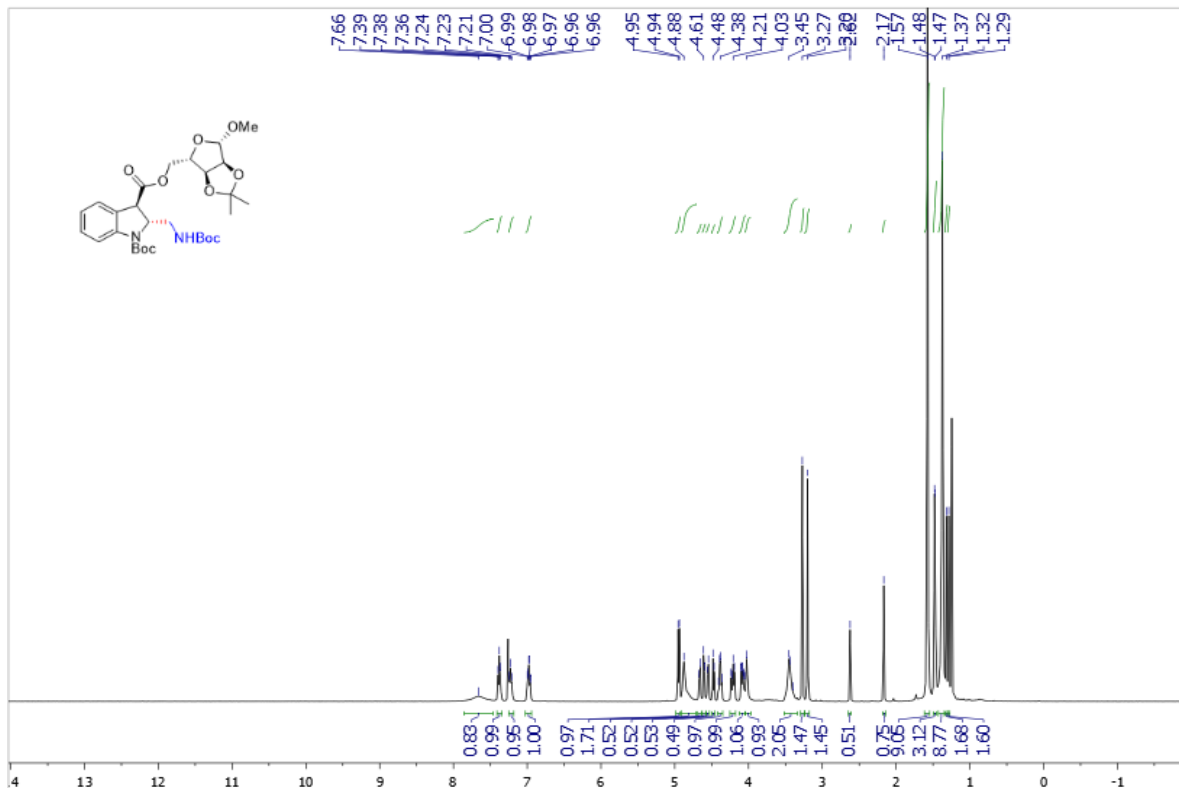
Supplementary Figure 137. 1 H NMR spectra of trans -3at
