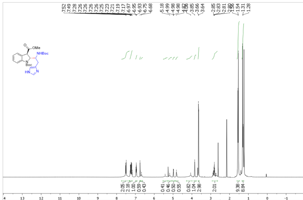
Supplementary Figure 97. 1 H NMR spectra of trans -3z
