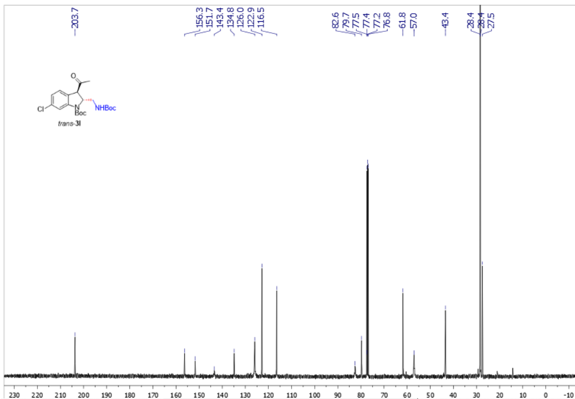
Supplementary Figure 68. 13 C NMR spectra of trans -31
