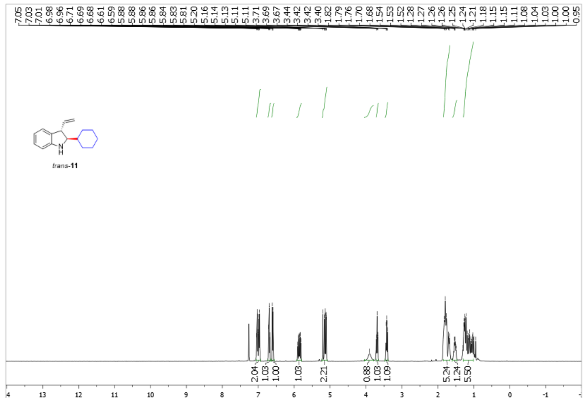
Supplementary Figure 191. 1 H NMR spectra of trans -11
