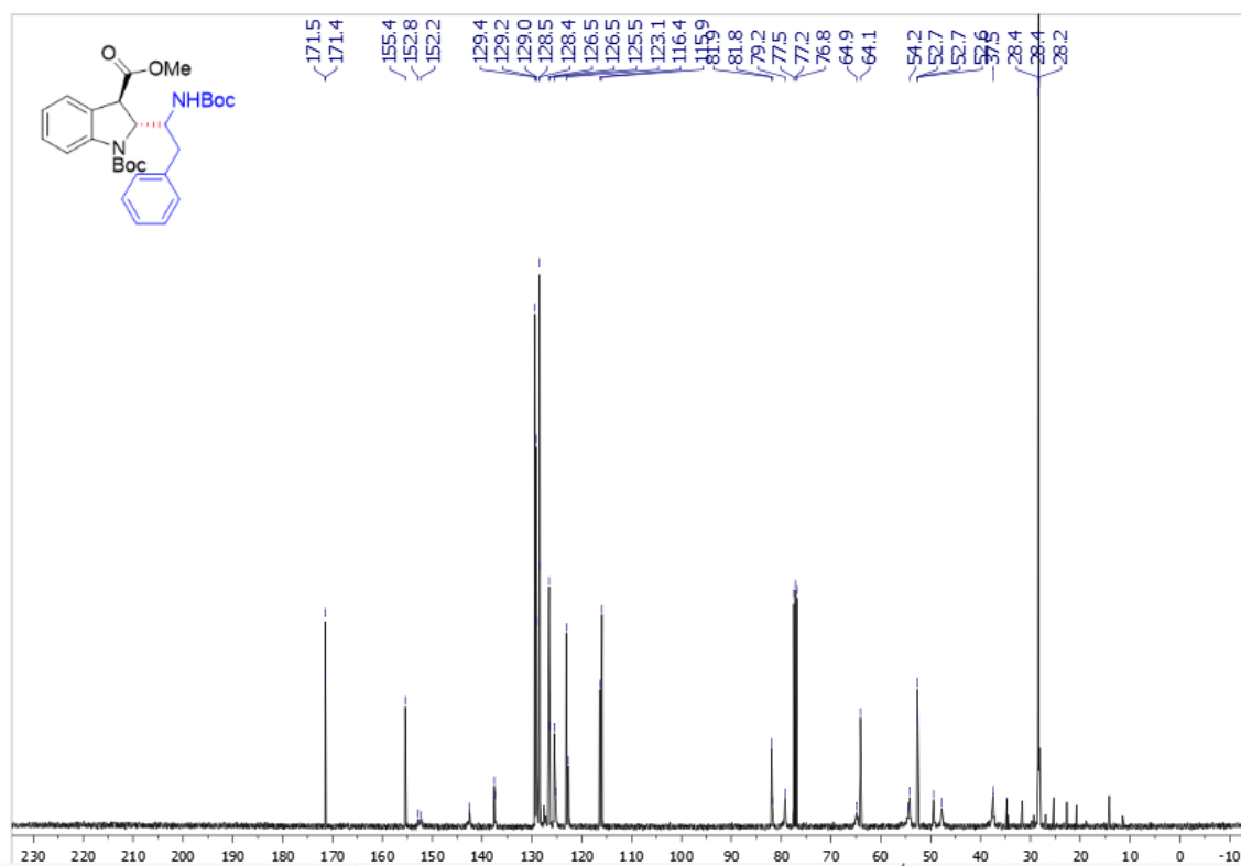
Supplementary Figure 92. 13 C NMR spectra of trans -3w
