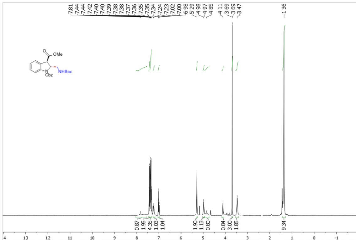
Supplementary Figure 65. ^1\text{H} NMR spectra of trans -3k
