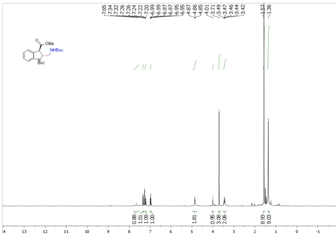
Supplementary Figure 89. ^1\text{H} NMR spectra of trans -3v
