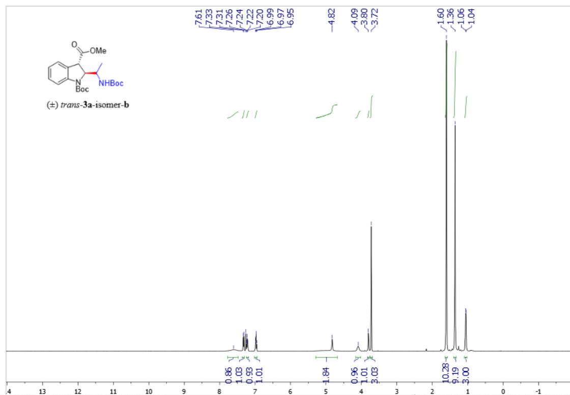
Supplementary Figure 43. ^1\text{H} NMR spectra of trans -3a-isomer-b
