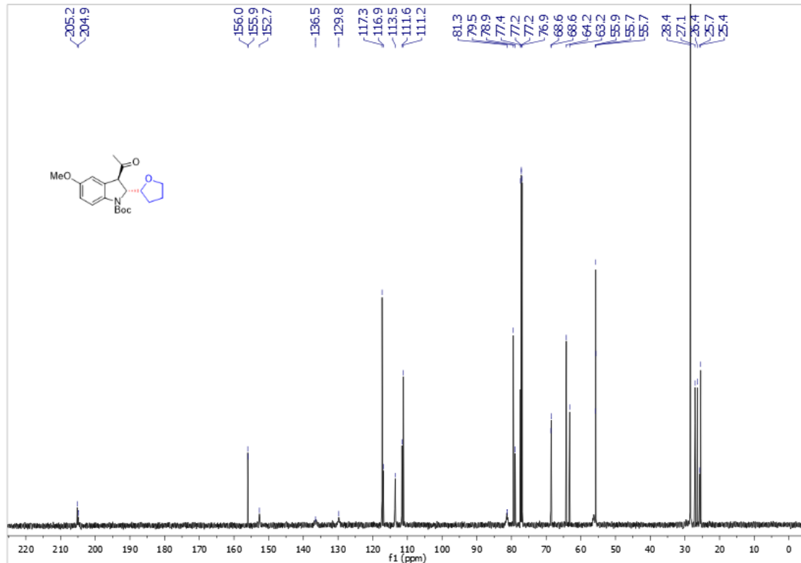
Supplementary Figure 72. ^{13}\text{C} NMR spectra of trans -3n
