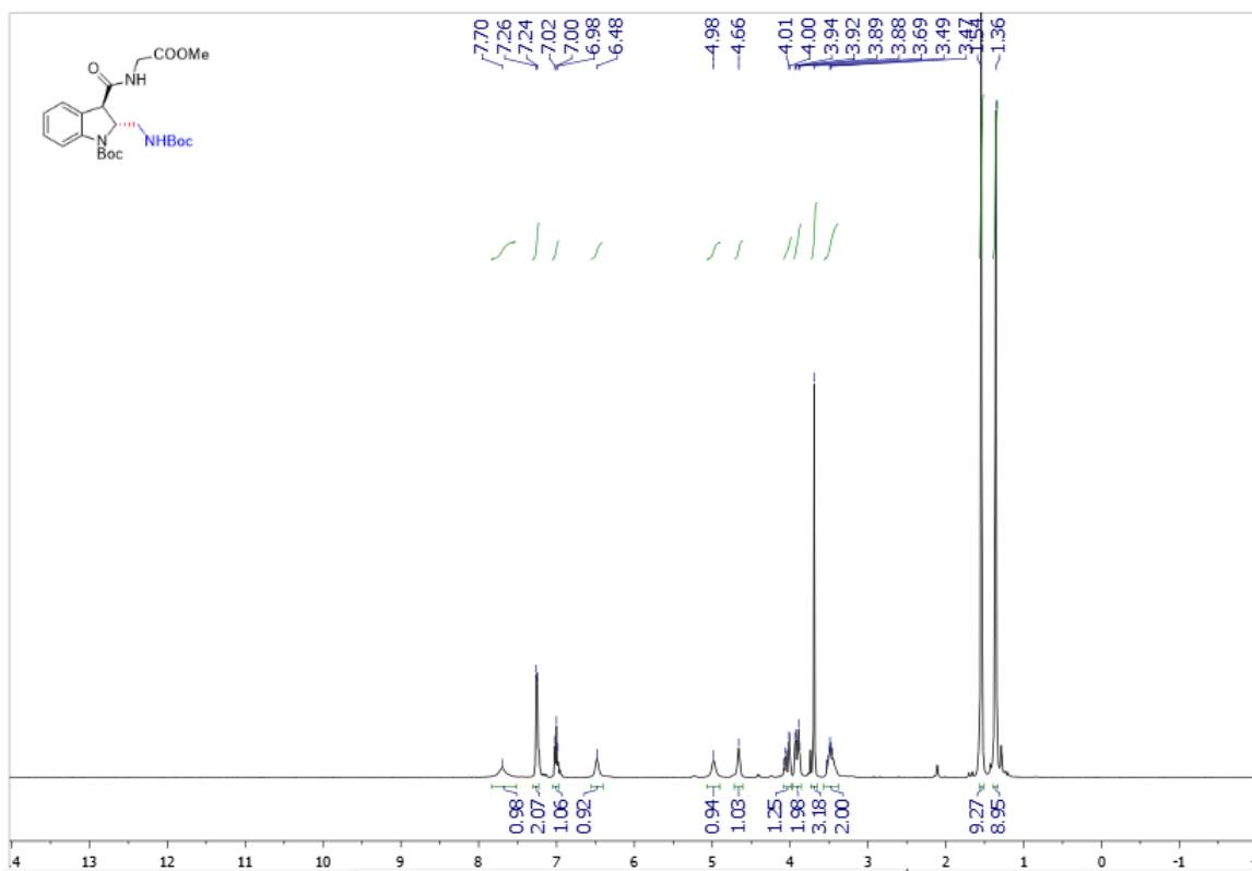
Supplementary Figure 57. ^1\text{H} NMR spectra of trans -3g
