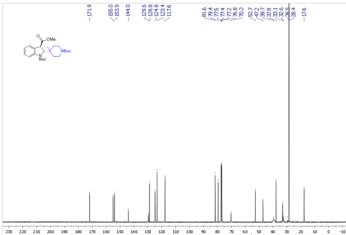
Supplementary Figure 132. ^{13}\text{C} NMR spectra of trans -3aq
