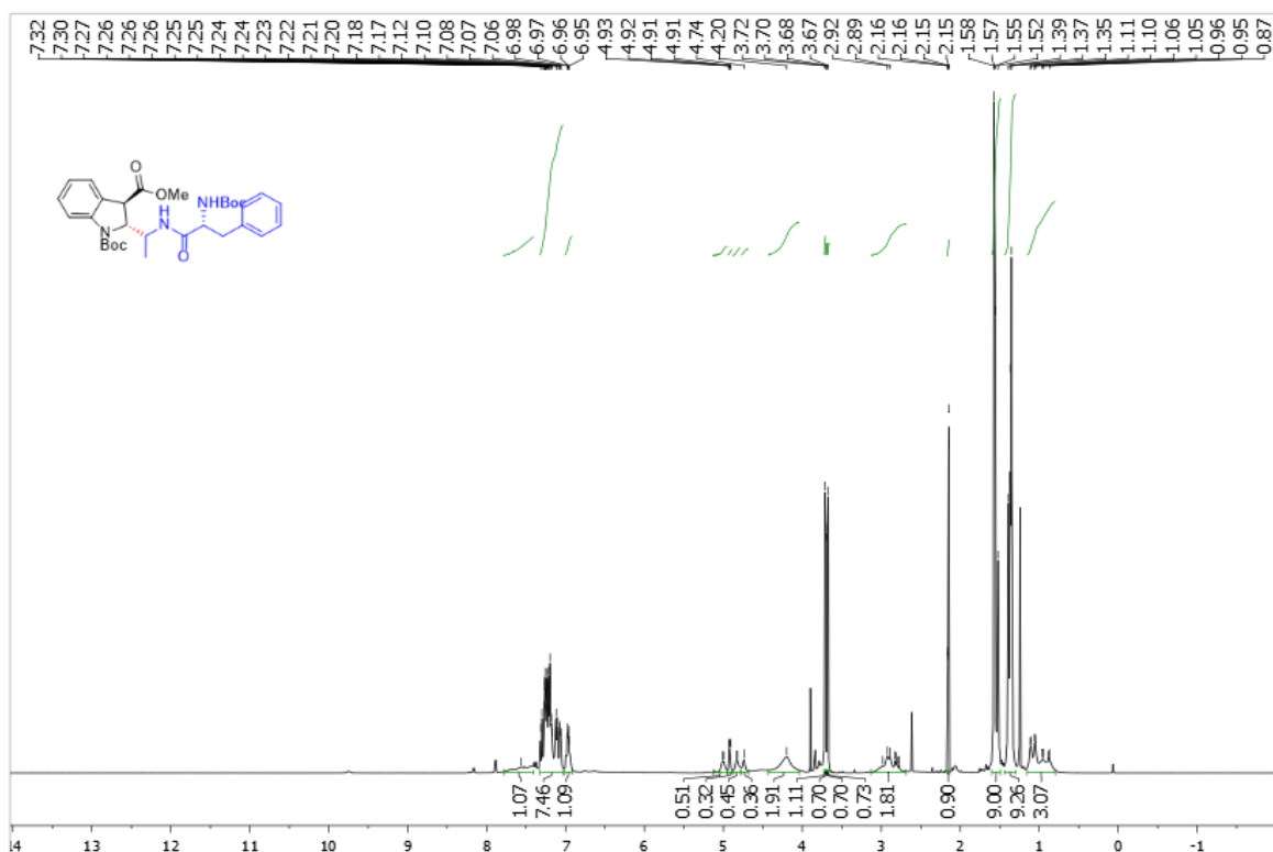
Supplementary Figure 133. ^1\text{H} NMR spectra of trans -3ar
