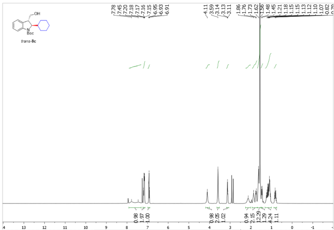
Supplementary Figure 185. 1 H NMR spectra of trans-8c
