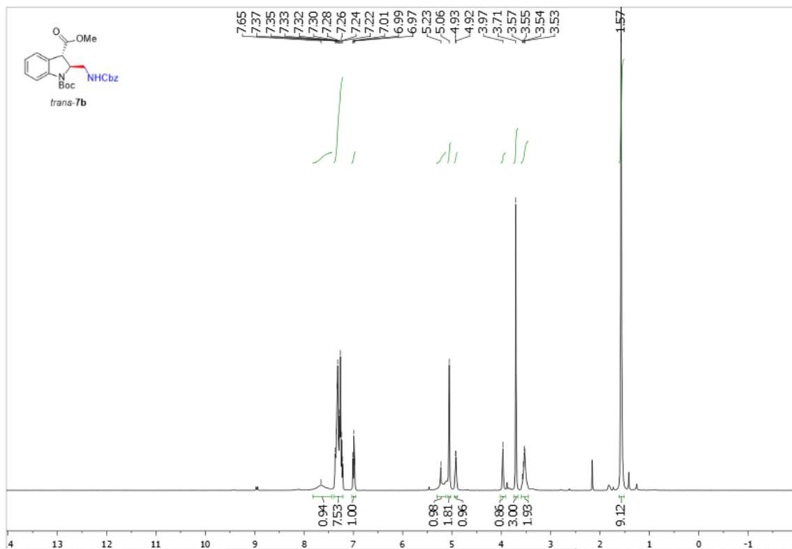
Supplementary Figure 152. 1 H NMR spectra of trans -7b
