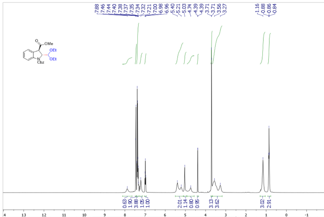
Supplementary Figure 115. ^1\text{H} NMR spectra of trans -3ai
