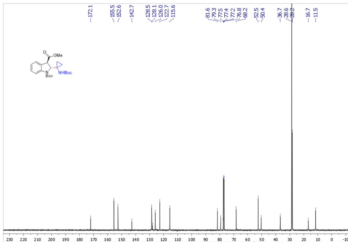
Supplementary Figure 108. ^{13}\text{C} NMR spectra of trans -3ae
