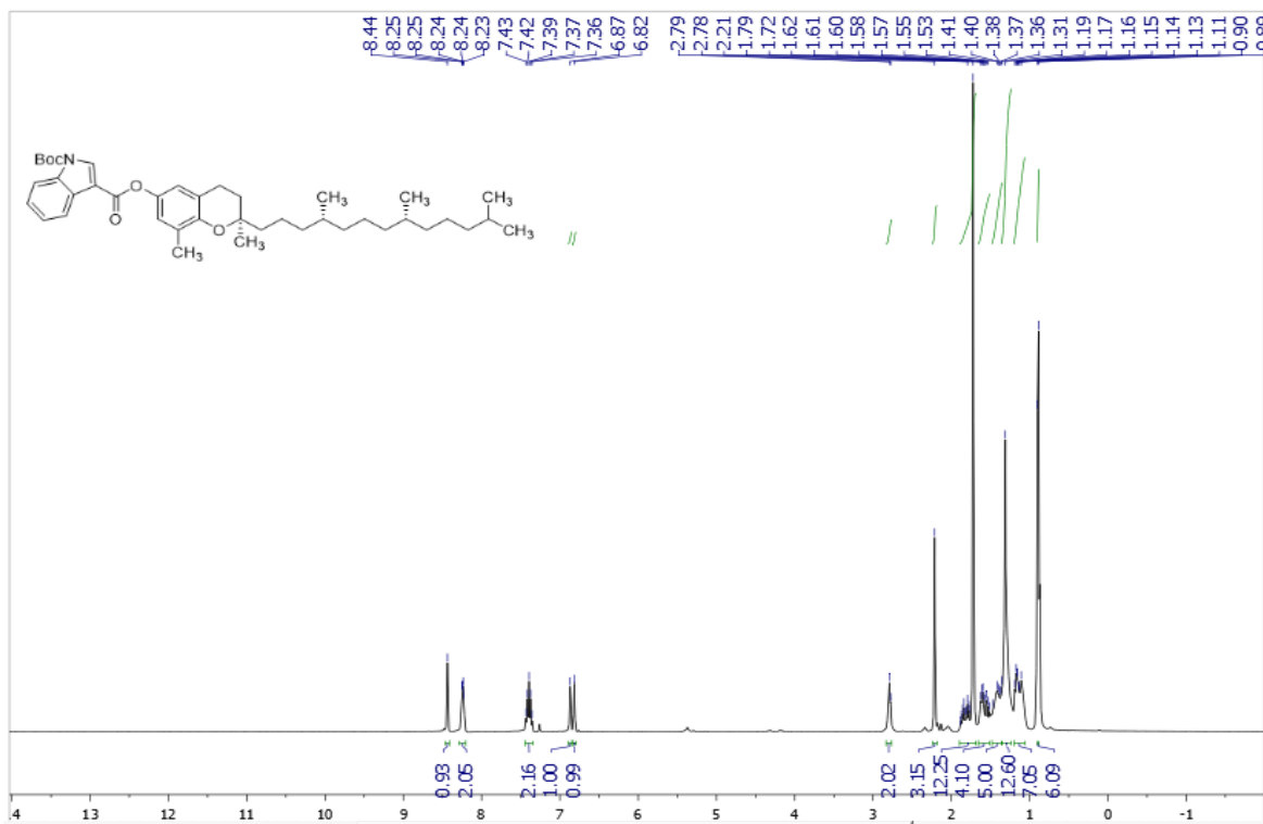
Supplementary Figure 35. ^1\text{H} NMR spectra of 1ax
