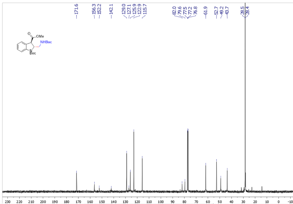
Supplementary Figure 90. ^{13}\text{C} NMR spectra of trans -3v
