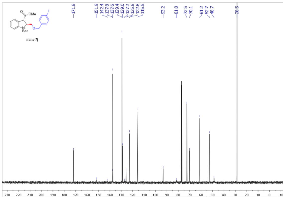
Supplementary Figure 165. 13 C NMR spectra of trans -7j
