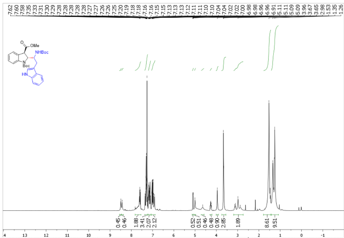
Supplementary Figure 93. ^1\text{H} NMR spectra of trans -3x
