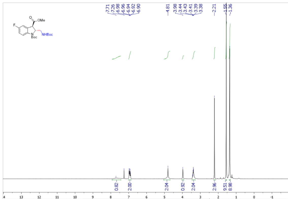
Supplementary Figure 69. ^1\text{H} NMR spectra of trans -3m
