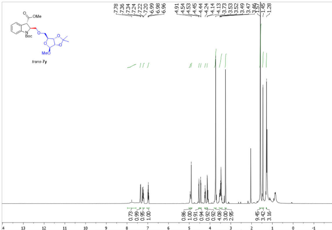
Supplementary Figure 178. 1 H NMR spectra of trans -7y
