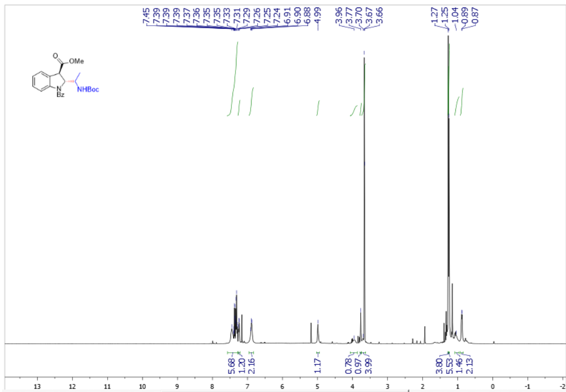
Supplementary Figure 61. ^1\text{H} NMR spectra of trans -3i
