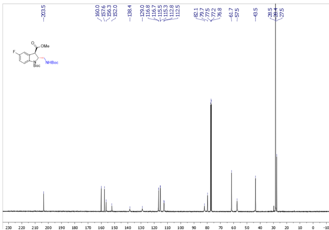
Supplementary Figure 70. ^{13}\text{C} NMR spectra of trans -3m
