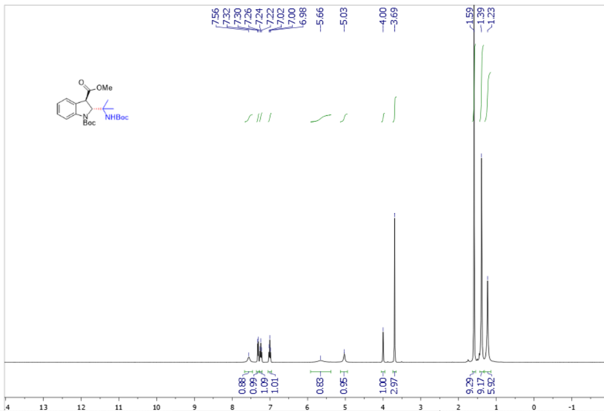
Supplementary Figure 105. ^1\text{H} NMR spectra of trans -3ad
