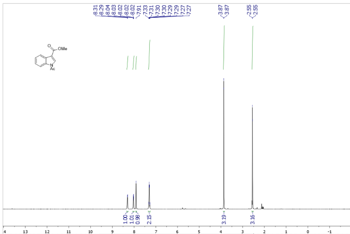
Supplementary Figure 11. ^1\text{H} NMR spectra of 1j
