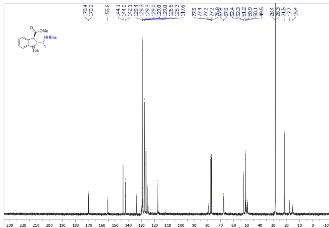
Supplementary Figure 60. ^{13}\text{C} NMR spectra of trans -3h
