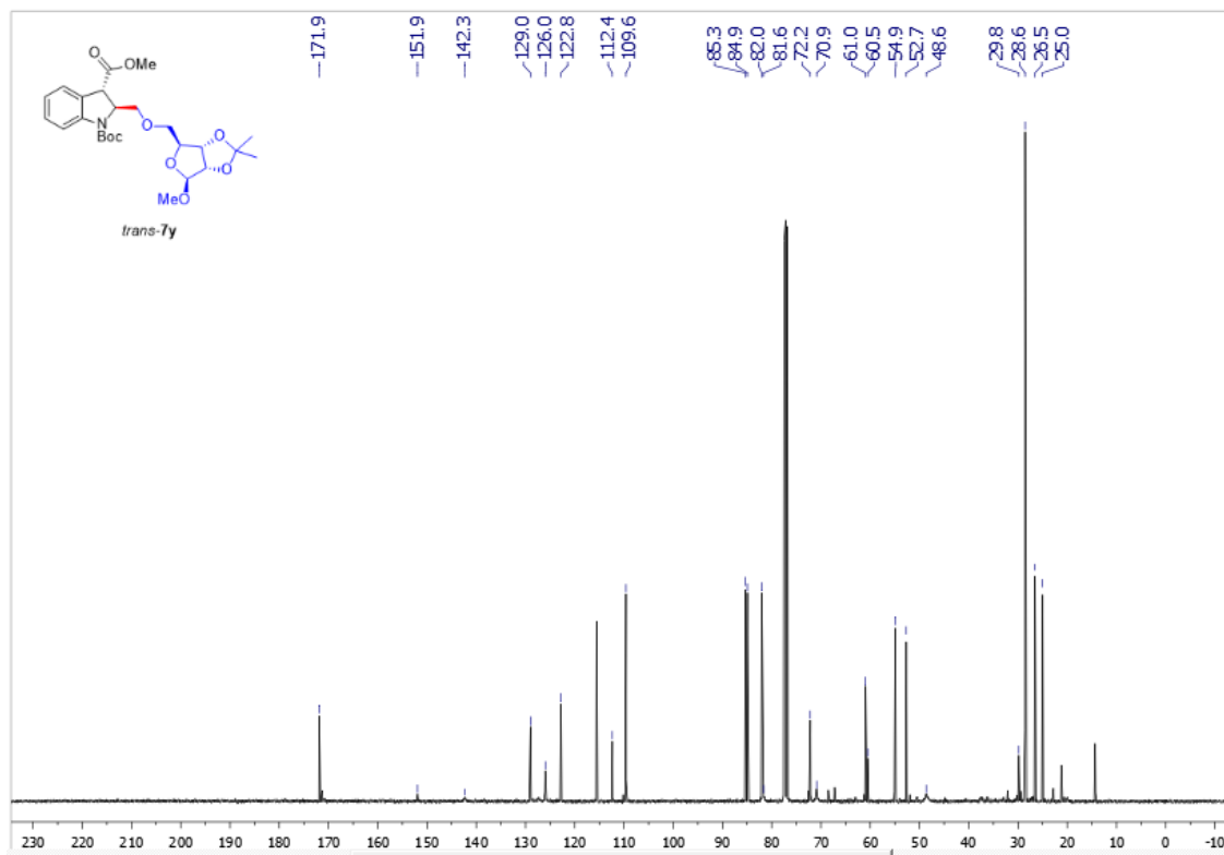
Supplementary Figure 179. 13 C NMR spectra of trans -7y
