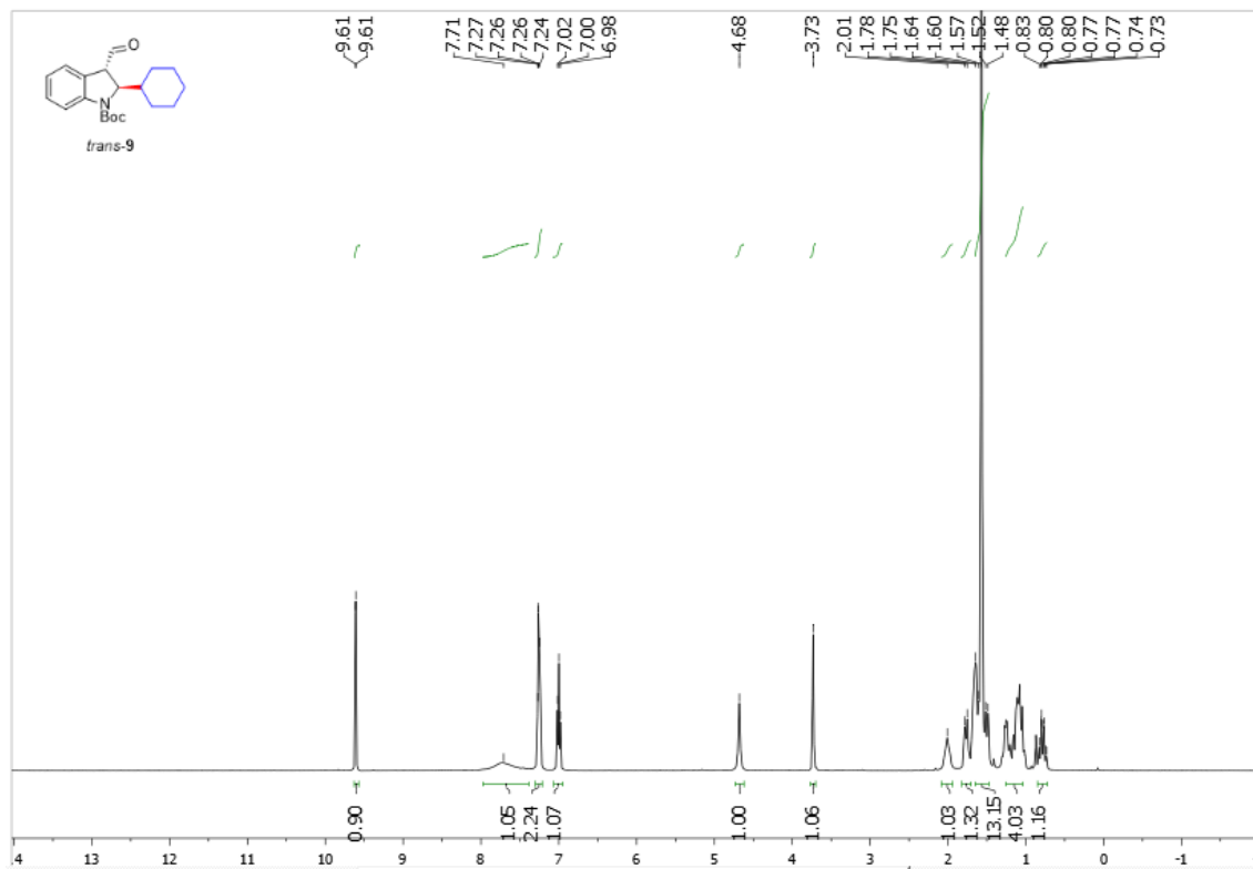
Supplementary Figure 187. 1 H NMR spectra of trans-9
