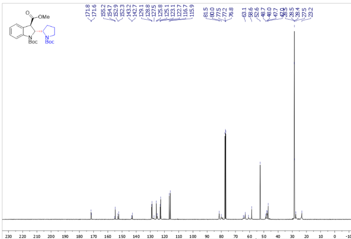
Supplementary Figure 104. ^{13}\text{C} NMR spectra of trans -3ac
