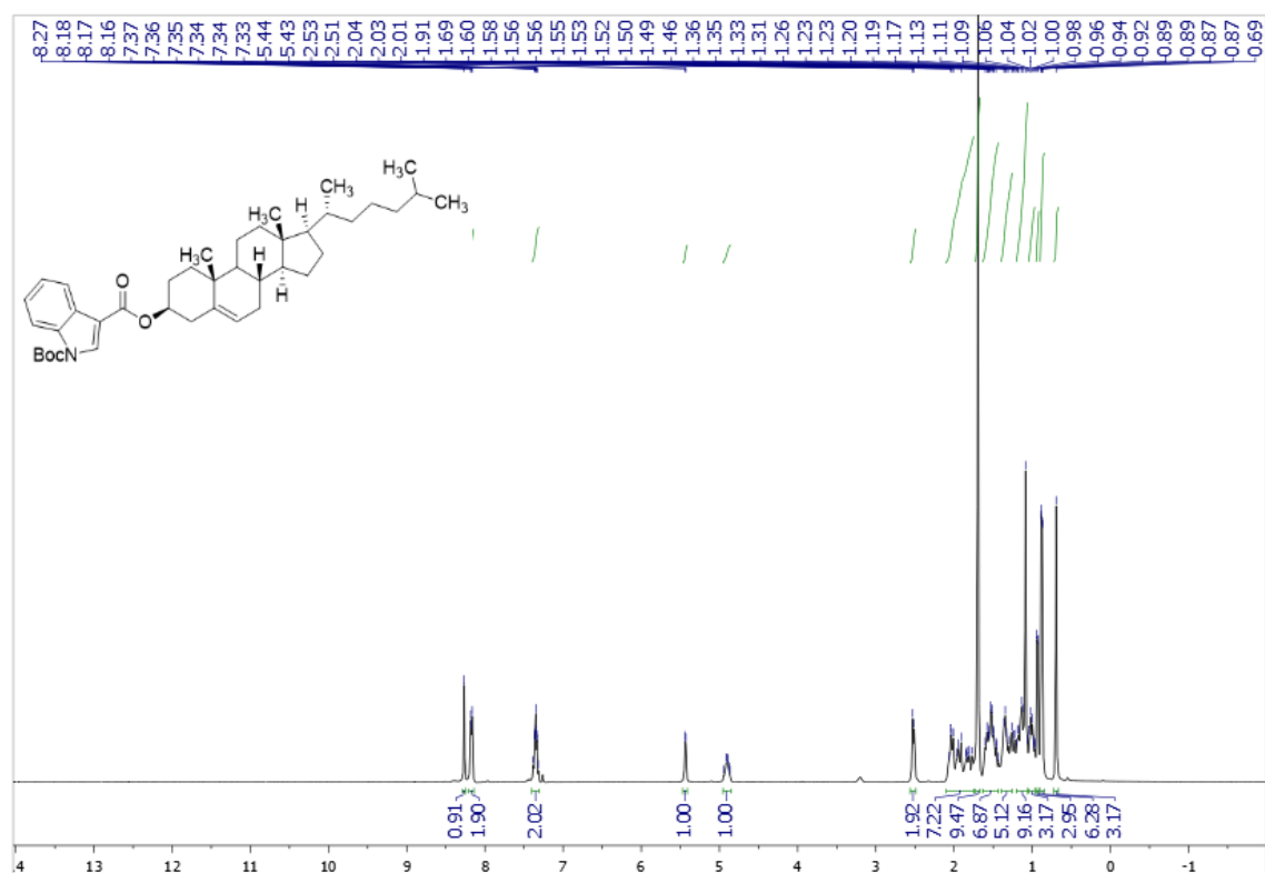
Supplementary Figure 33. ^1\text{H} NMR spectra of 1av
