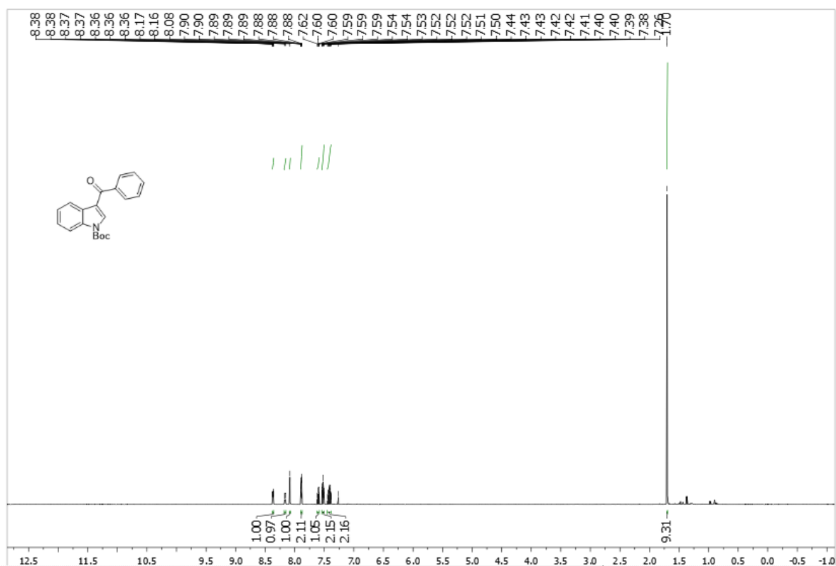
Supplementary Figure 5. ^1\text{H} NMR spectra of 1e
