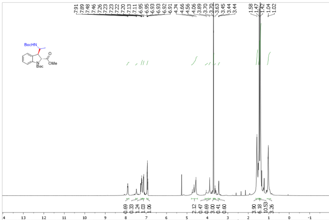
Supplementary Figure 79. ^1\text{H} NMR spectra of trans -3q
