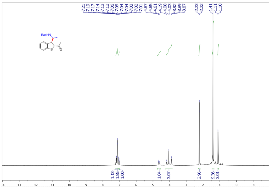
Supplementary Figure 87. ^1\text{H} NMR spectra of trans -3u
