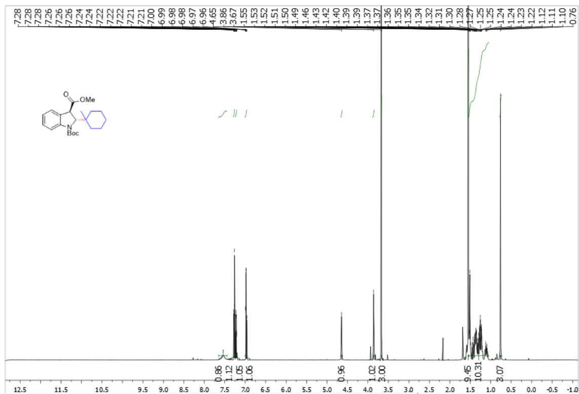
Supplementary Figure 123. ^1\text{H} NMR spectra of trans -3am
