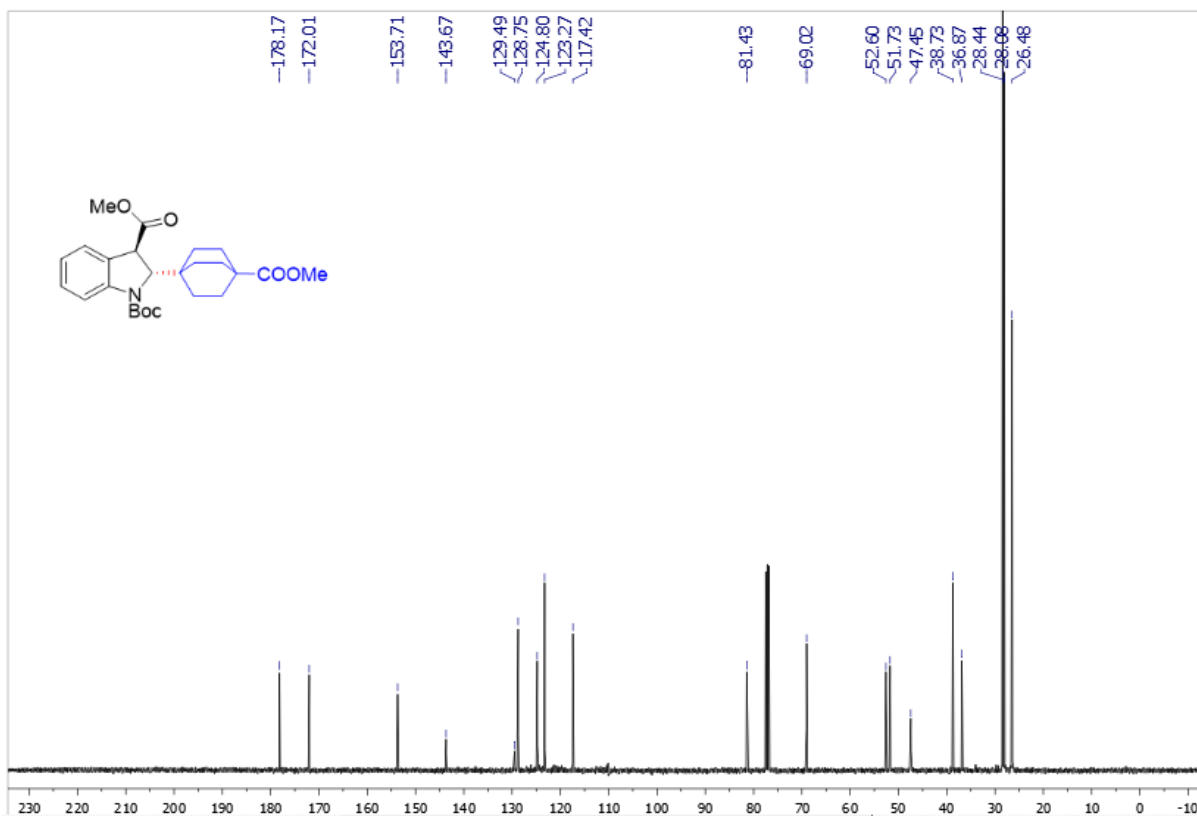
Supplementary Figure 126. ^{13}\text{C} NMR spectra of trans -3an
