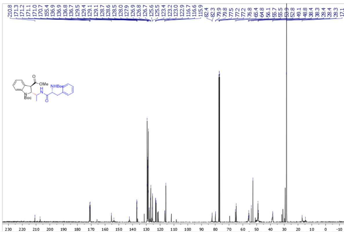
Supplementary Figure 134. ^{13}\text{C} NMR spectra of trans -3ar
