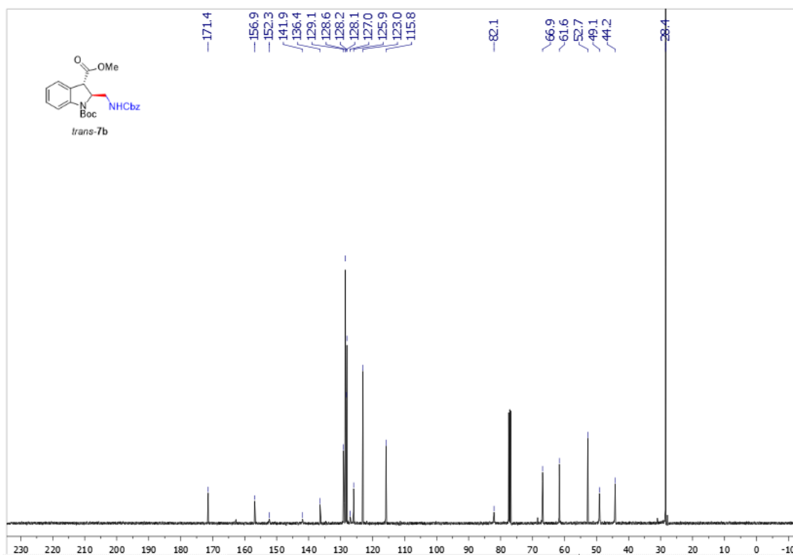
Supplementary Figure 153. 13 C NMR spectra of trans -7b
