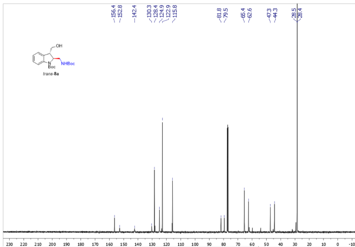
Supplementary Figure 182. 13 C NMR spectra of trans -8a
