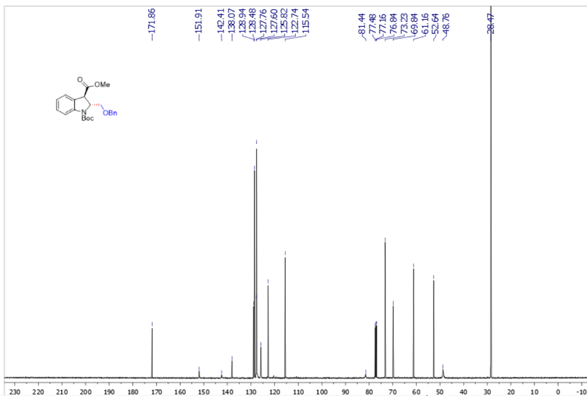
Supplementary Figure 112. ^{13}\text{C} NMR spectra of trans -3ag
