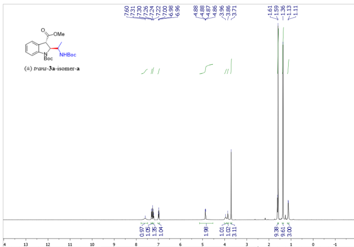
Supplementary Figure 41. ^1\text{H} NMR spectra of trans -3a-isomer-a
