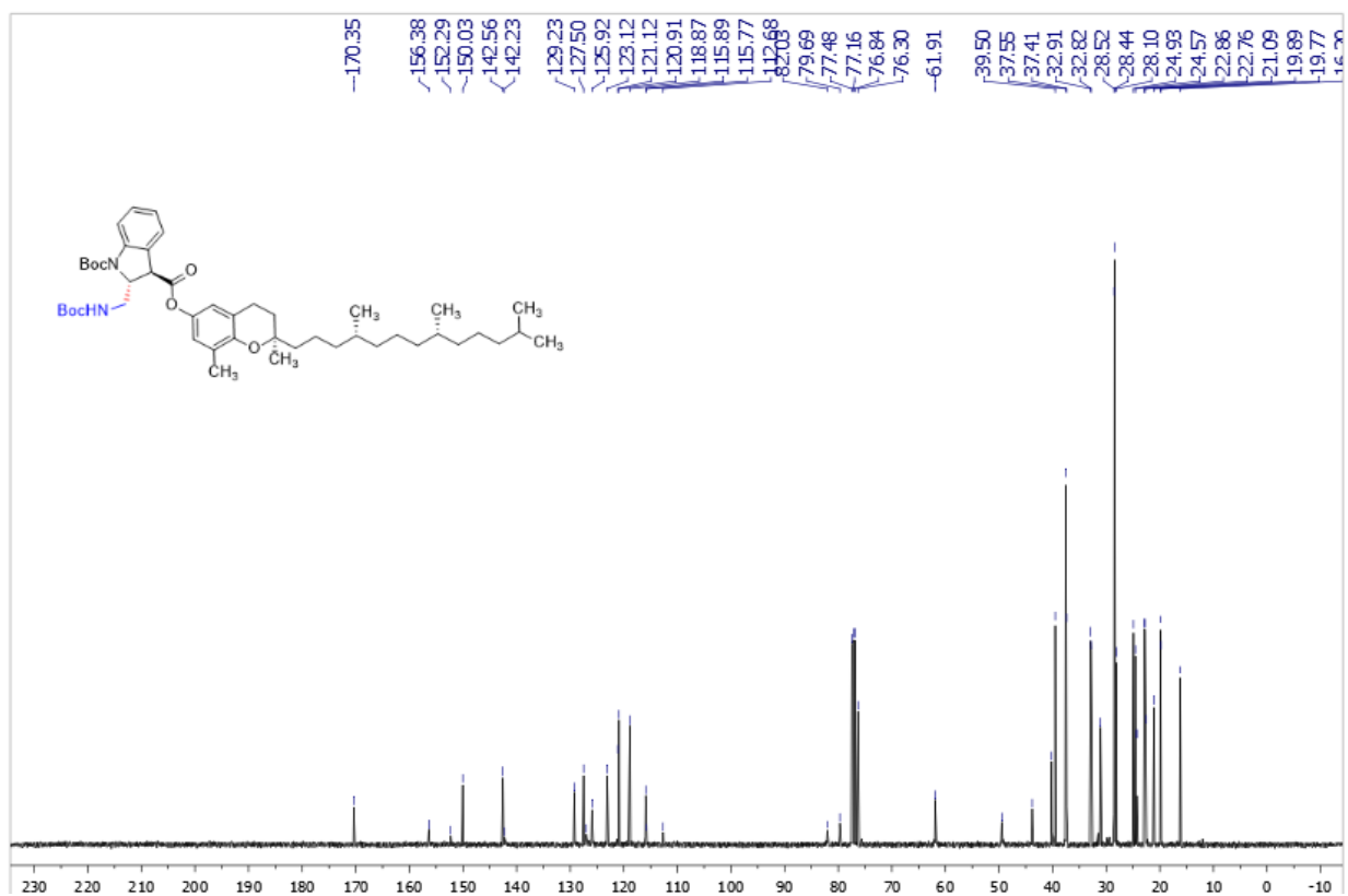
Supplementary Figure 146. 13 C NMR spectra of trans -3ax
