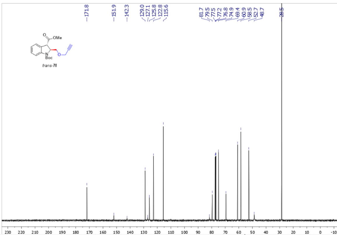
Supplementary Figure 161. ^{13}\text{C} NMR spectra of trans -7f
