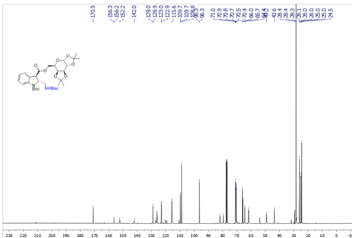
Supplementary Figure 140. 13 C NMR spectra of trans -3au
