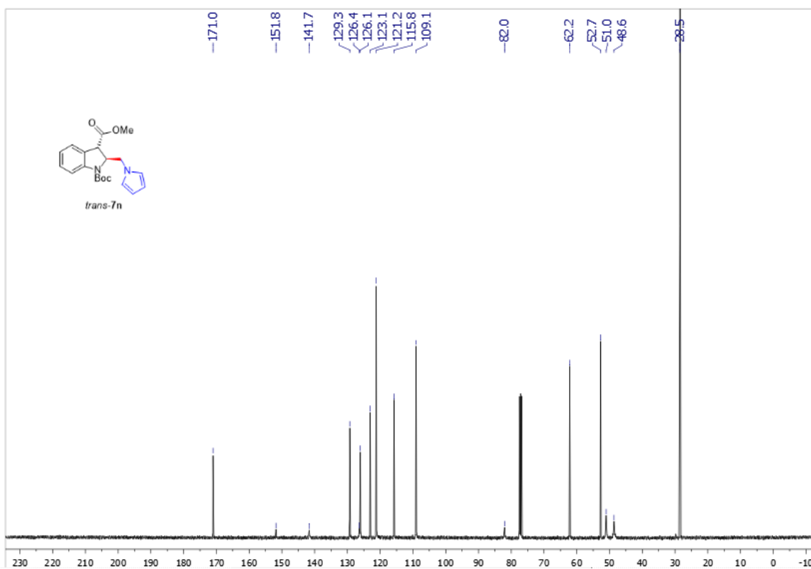
Supplementary Figure 173. ^{13}\text{C} NMR spectra of trans-7n
