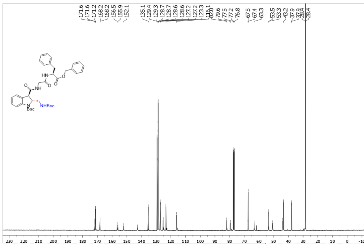
Supplementary Figure 142. 13 C NMR spectra of trans -3av
