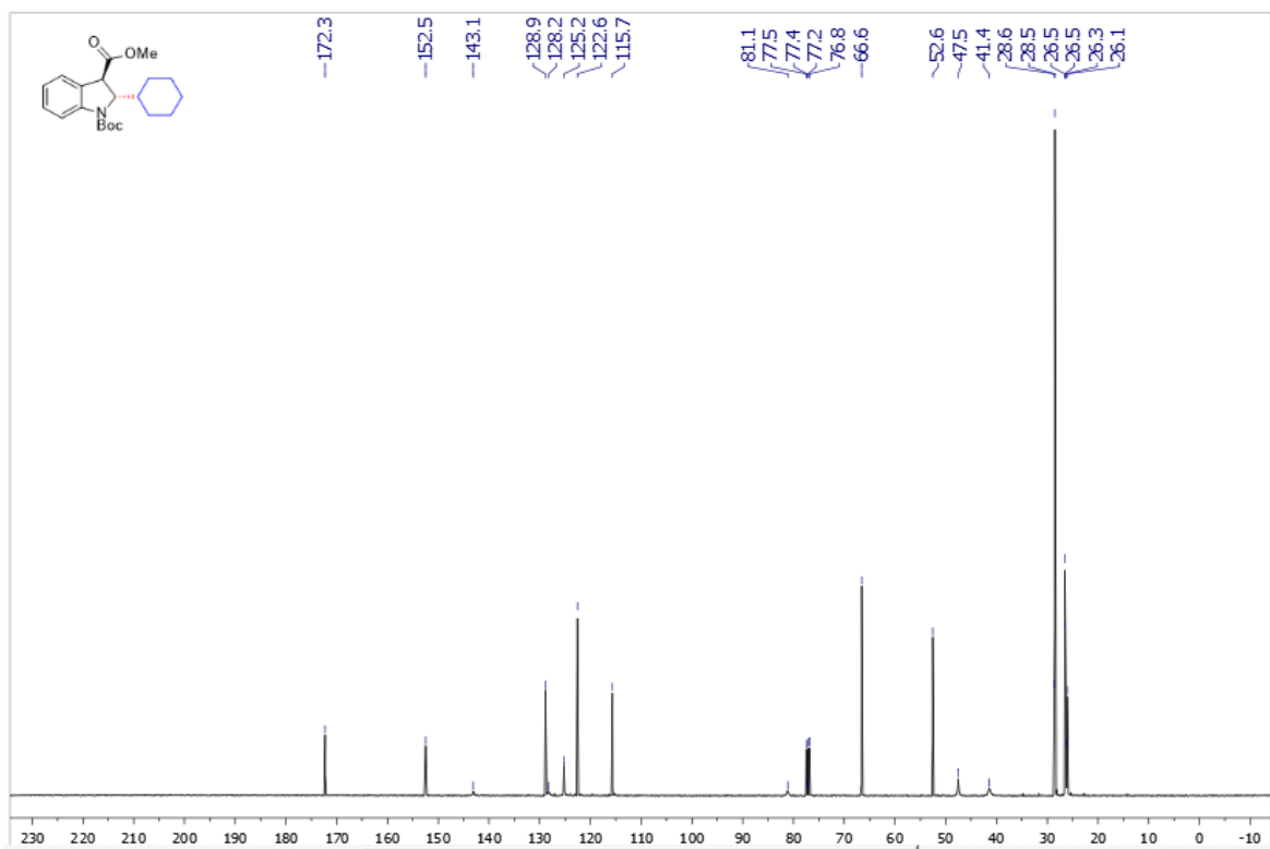
Supplementary Figure 118. ^{13}\text{C} NMR spectra of trans -3aj
