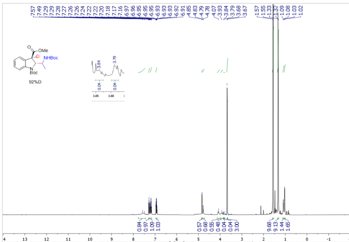
Supplementary Figure 147. ^1\text{H} NMR spectra of trans -3a-d
