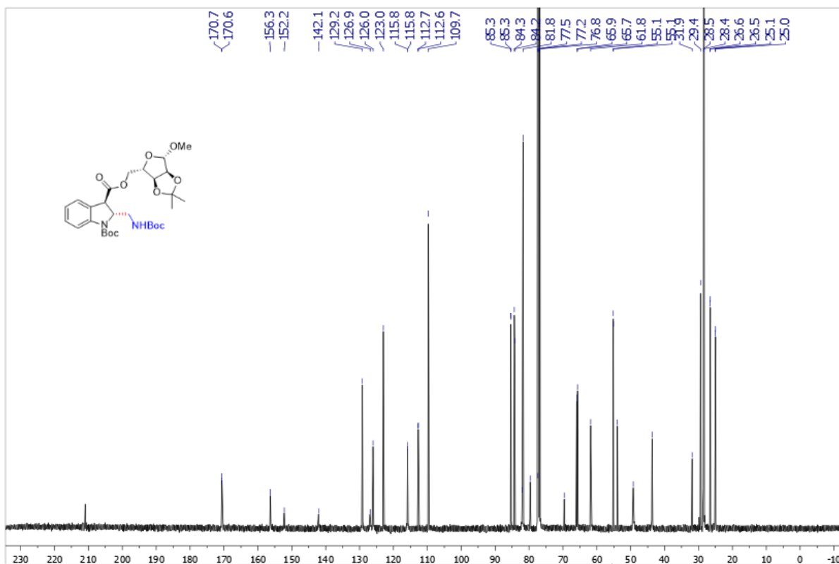
Supplementary Figure 138. 13 C NMR spectra of trans -3at
