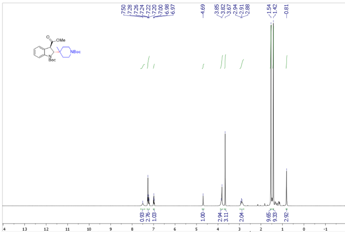
Supplementary Figure 131. ^1\text{H} NMR spectra of trans -3aq
