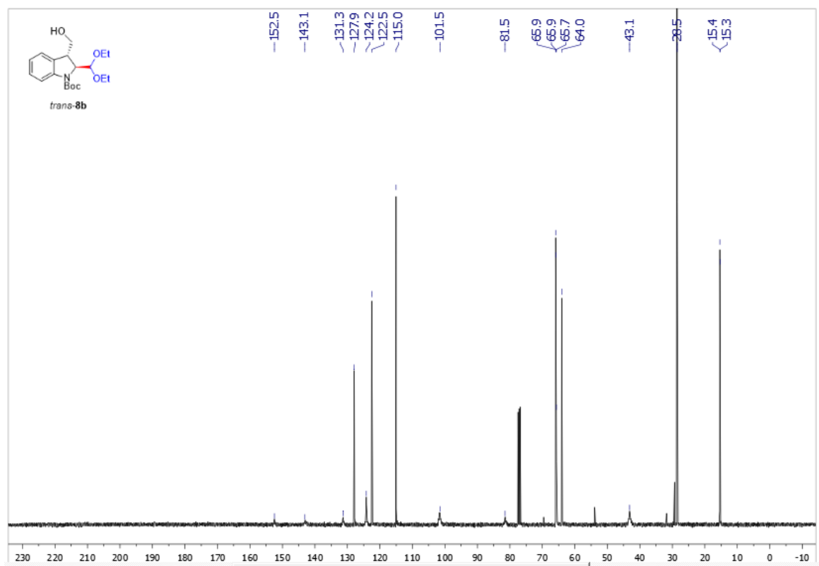
Supplementary Figure 184. 13 C NMR spectra of trans-8b
