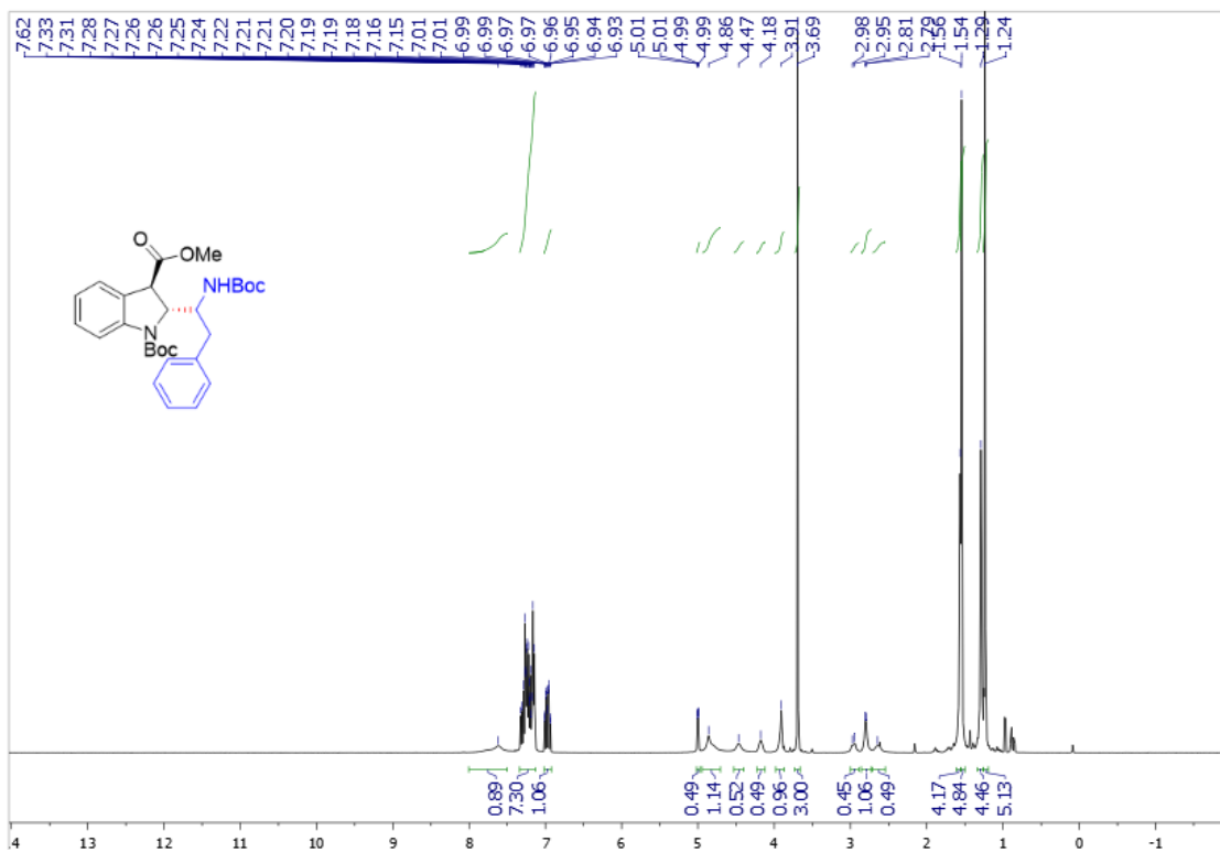
Supplementary Figure 91. 1 H NMR spectra of trans -3w
