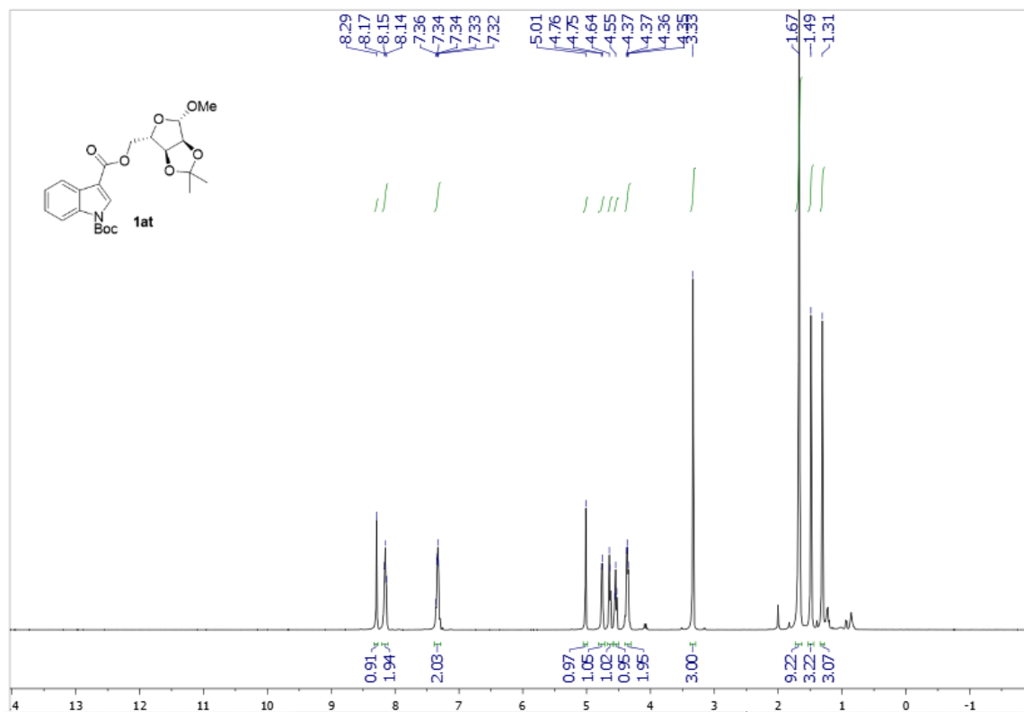
Supplementary Figure 27. ^1\text{H} NMR spectra of 1a t
