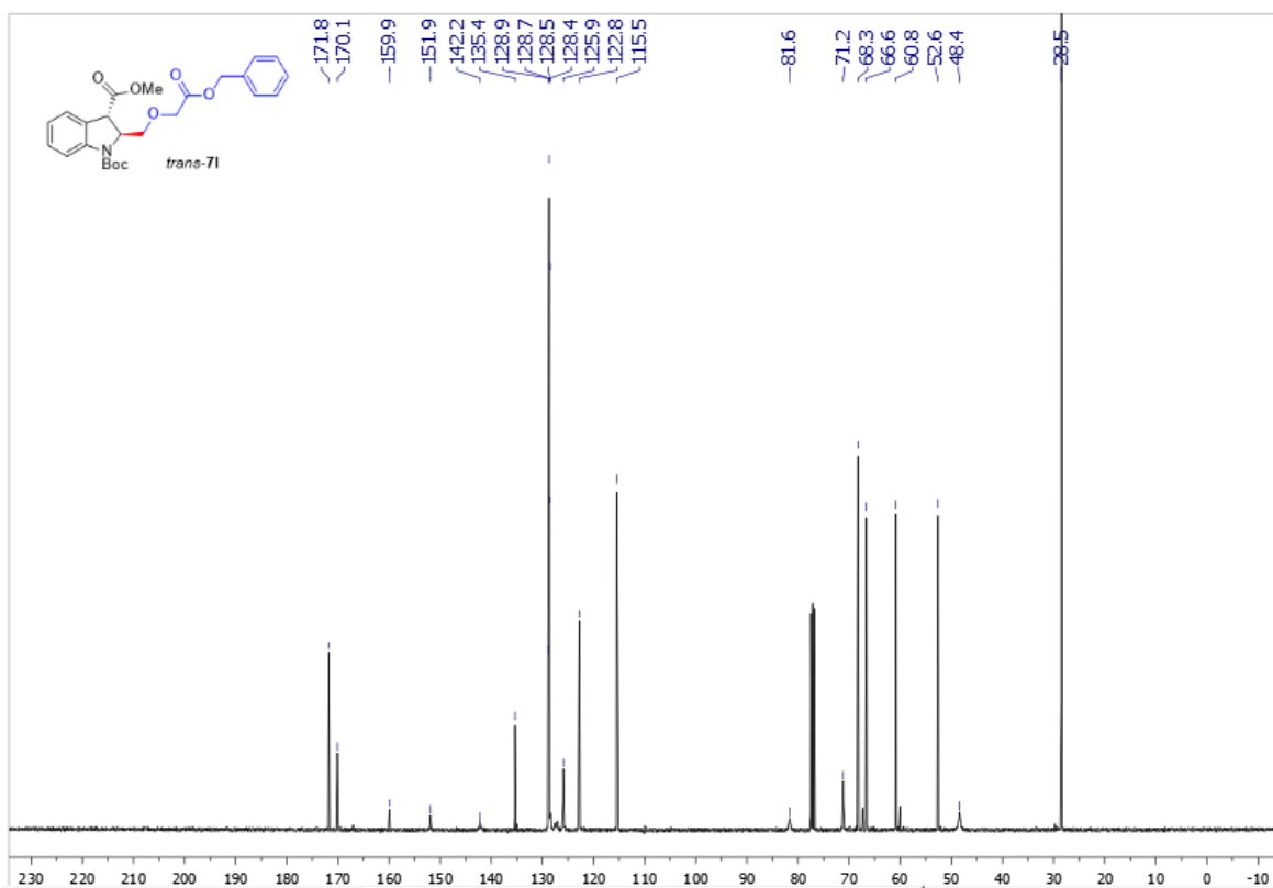
Supplementary Figure 169. 13 C NMR spectra of trans -71
