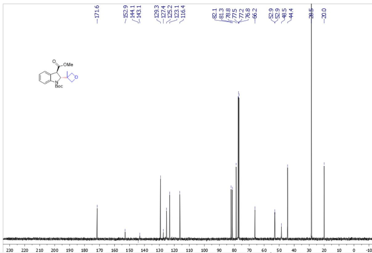
Supplementary Figure 128. 13 C NMR spectra of trans -3ao
