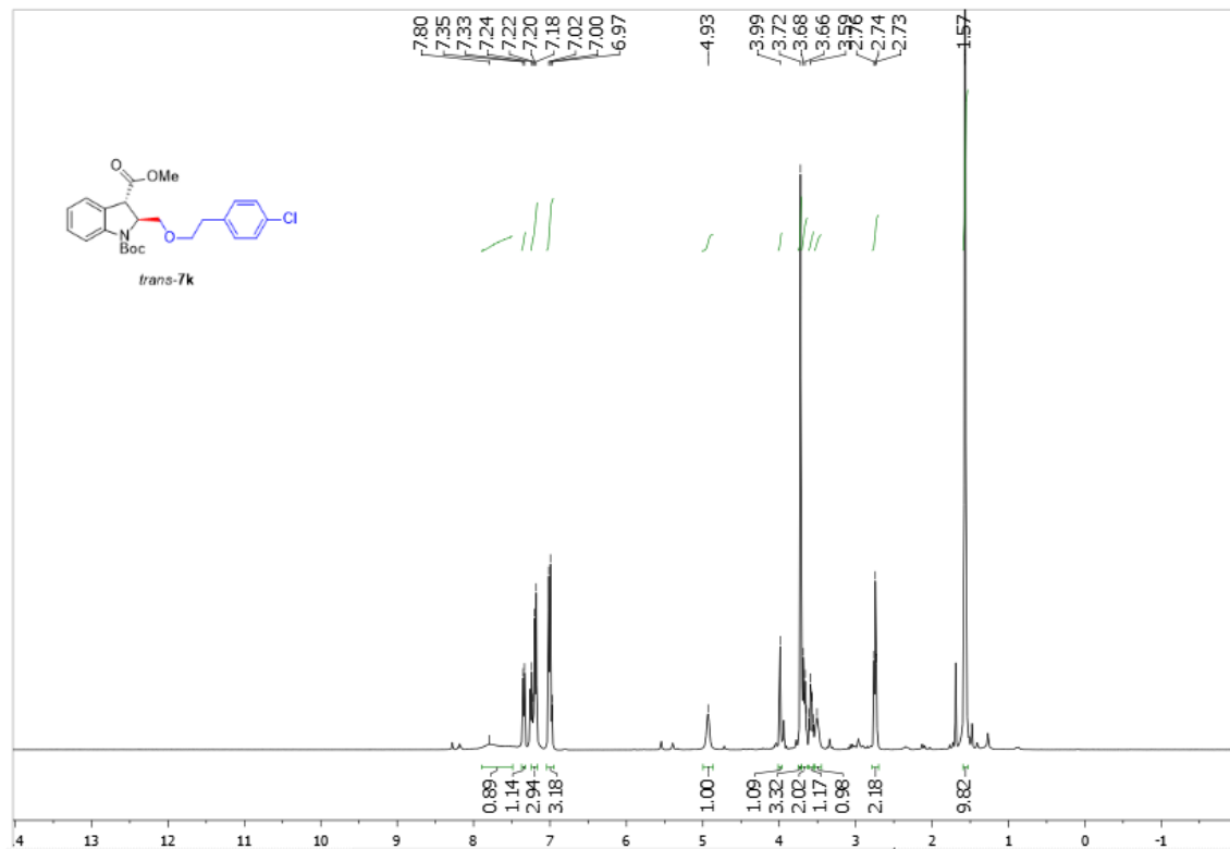
Supplementary Figure 166. 1 H NMR spectra of trans -7k
