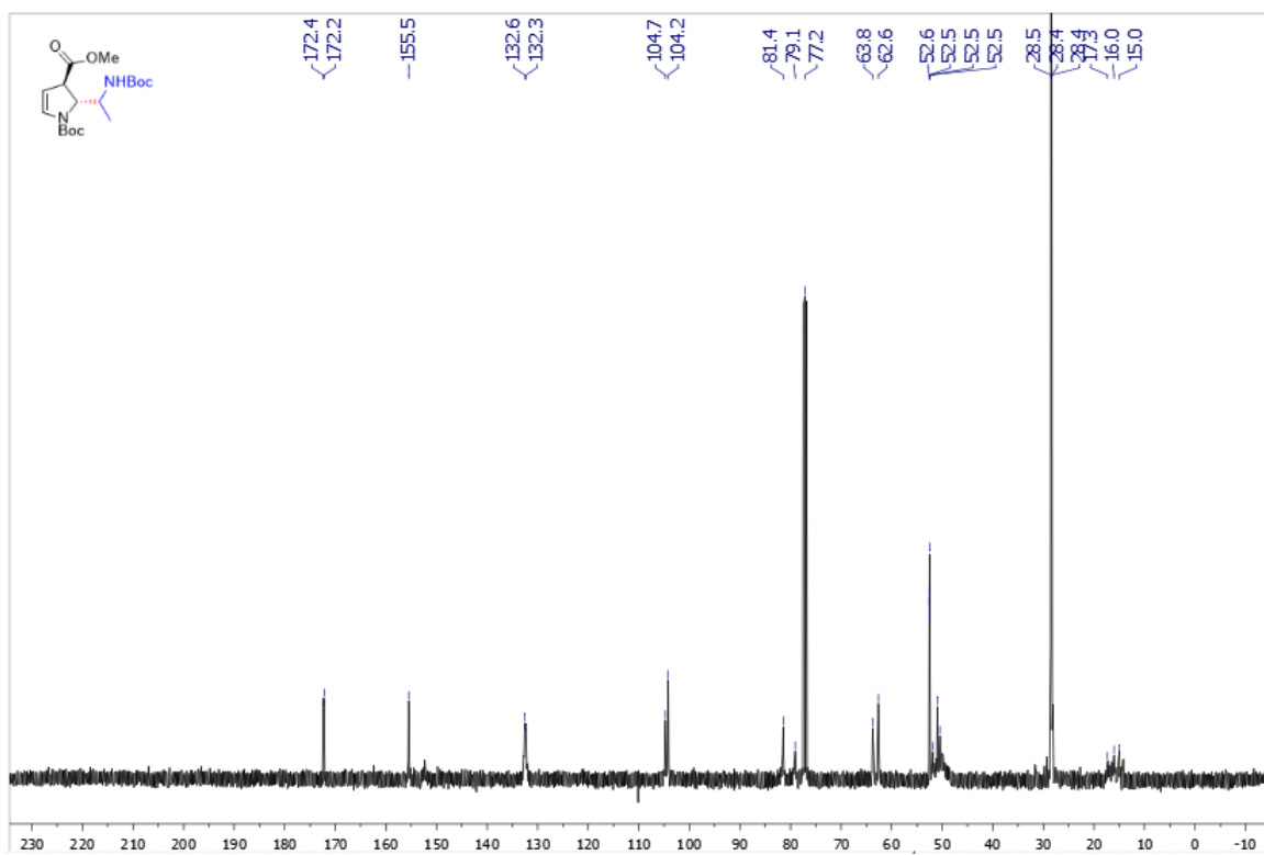
Supplementary Figure 84. ^{13}\text{C} NMR spectra of trans -3s
