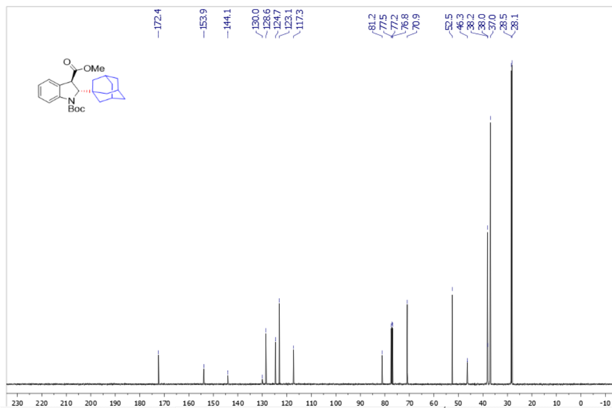
Supplementary Figure 130. 13 C NMR spectra of trans -3ap
