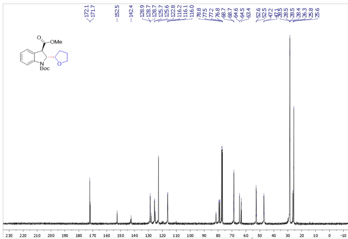
Supplementary Figure 110. ^{13}\text{C} NMR spectra of trans -3af
