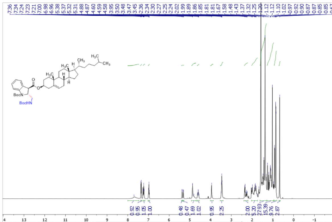
Supplementary Figure 143. 1 H NMR spectra of trans -3aw
