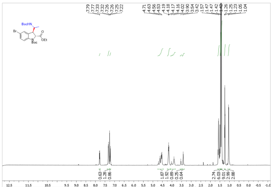
Supplementary Figure 81. 1 H NMR spectra of trans -3r
