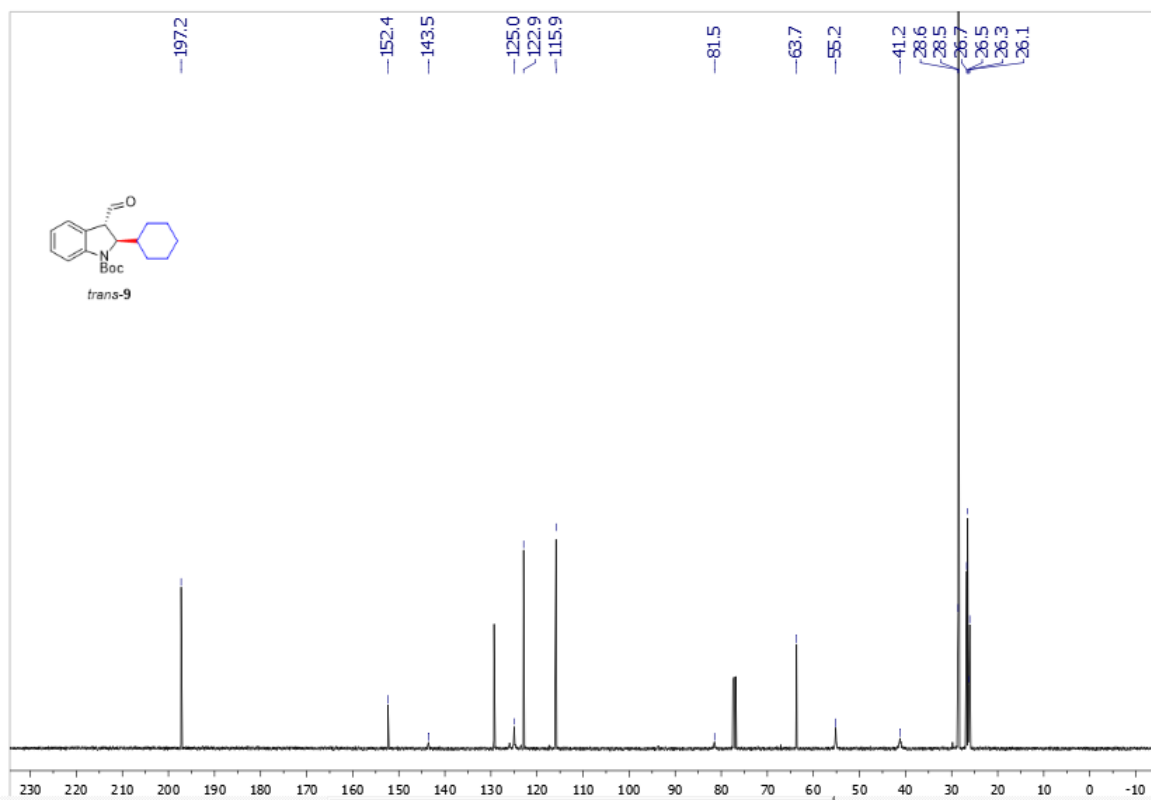
Supplementary Figure 188. 13 C NMR spectra of trans-9
