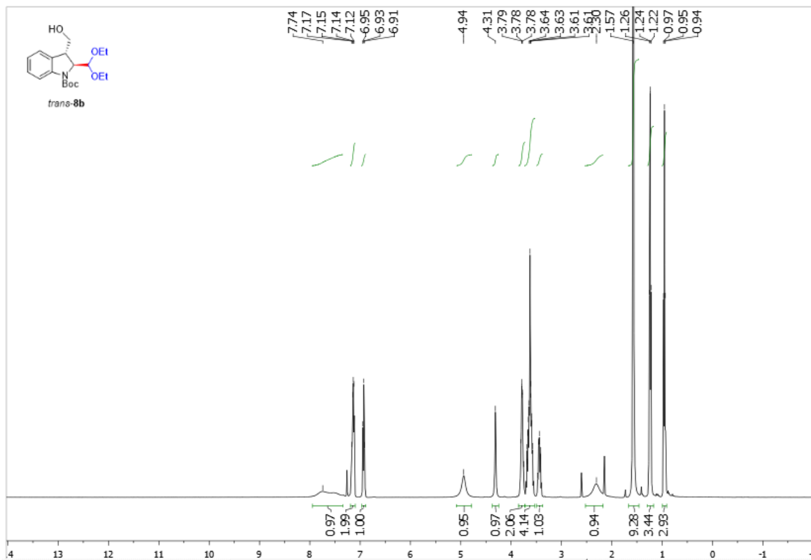
Supplementary Figure 183. 1 H NMR spectra of trans-8b
