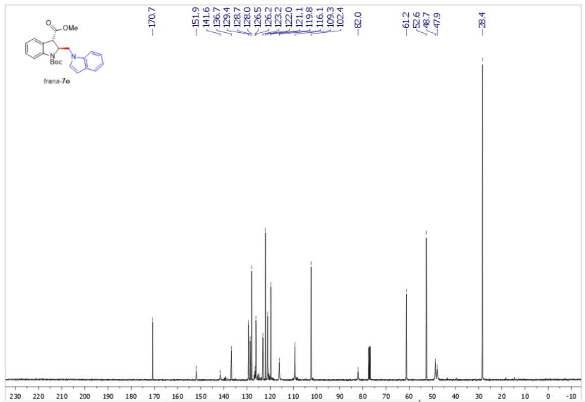
Supplementary Figure 175. 13 C NMR spectra of trans -7o
