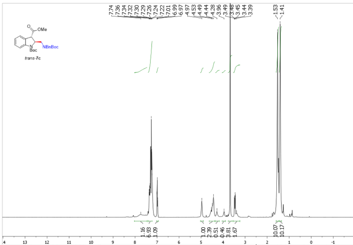
Supplementary Figure 154. 1 H NMR spectra of trans -7c
