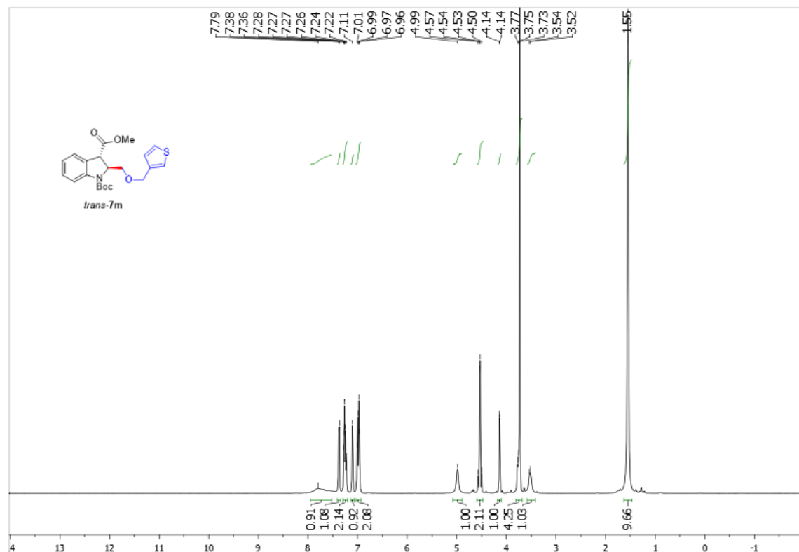
Supplementary Figure 170. 1 H NMR spectra of trans -7m
