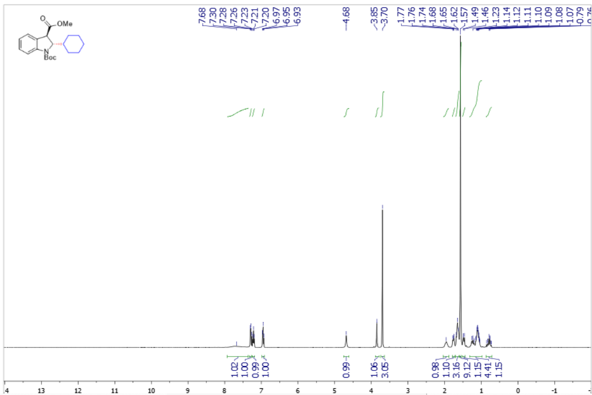
Supplementary Figure 117. ^1\text{H} NMR spectra of trans -3aj
