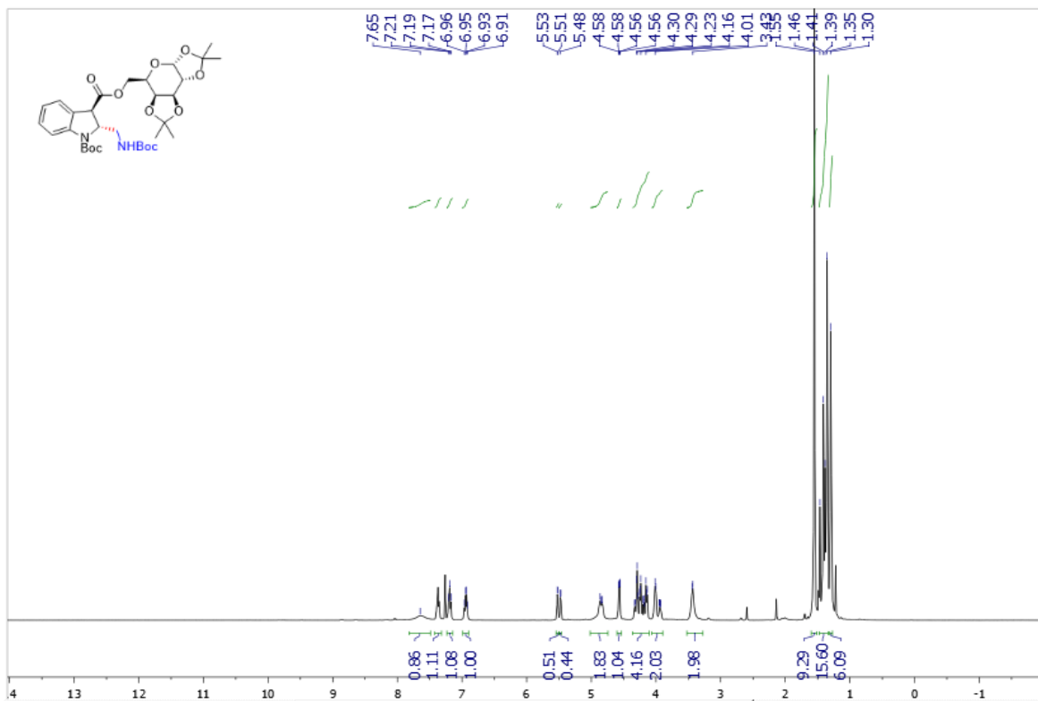
Supplementary Figure 139. 1 H NMR spectra of trans -3au
