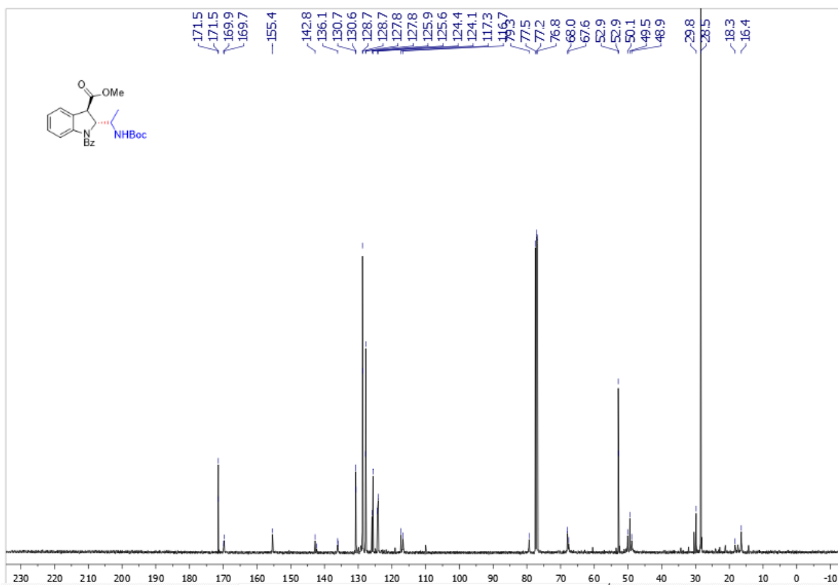
Supplementary Figure 62. ^{13}\text{C} NMR spectra of trans -3i
