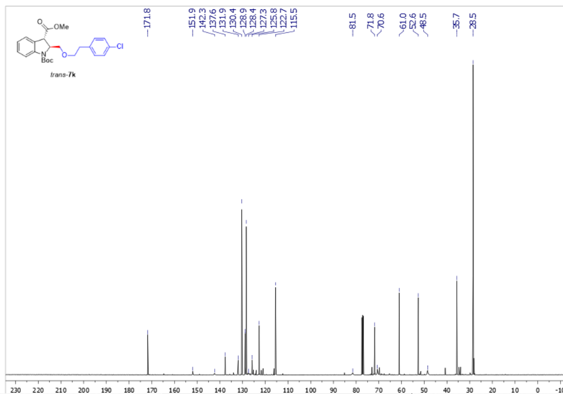
Supplementary Figure 167. 13 C NMR spectra of trans -7k
