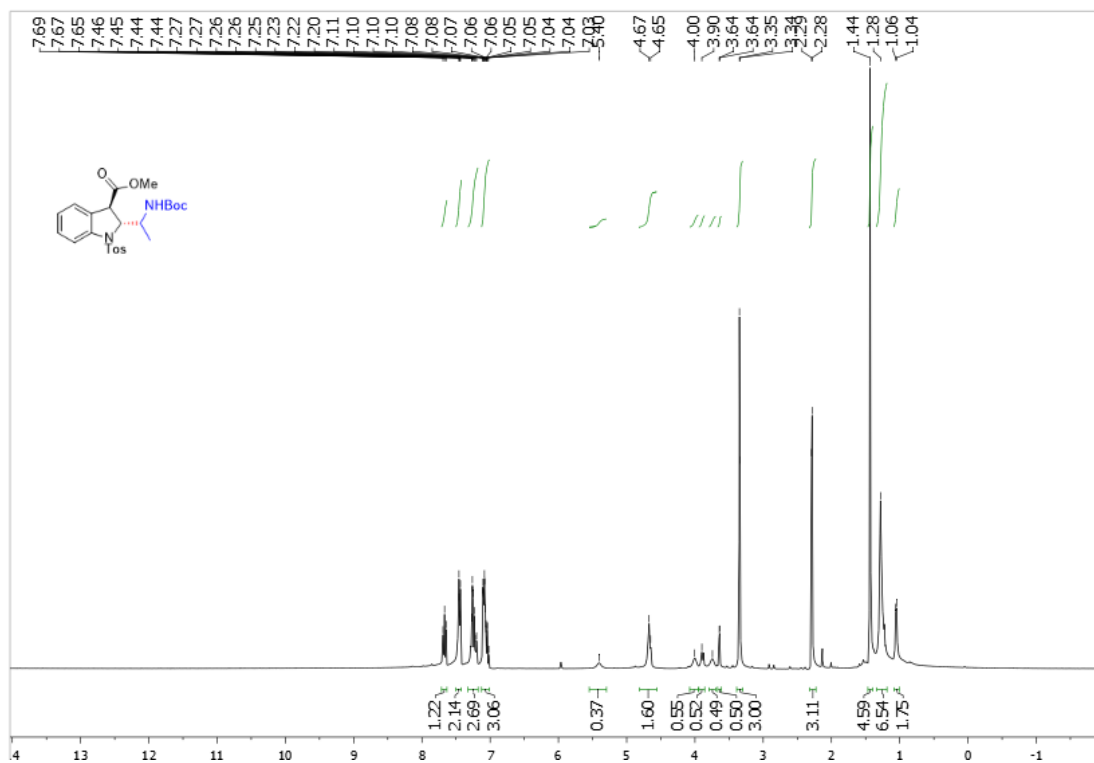
Supplementary Figure 59. ^1\text{H} NMR spectra of trans -3h
