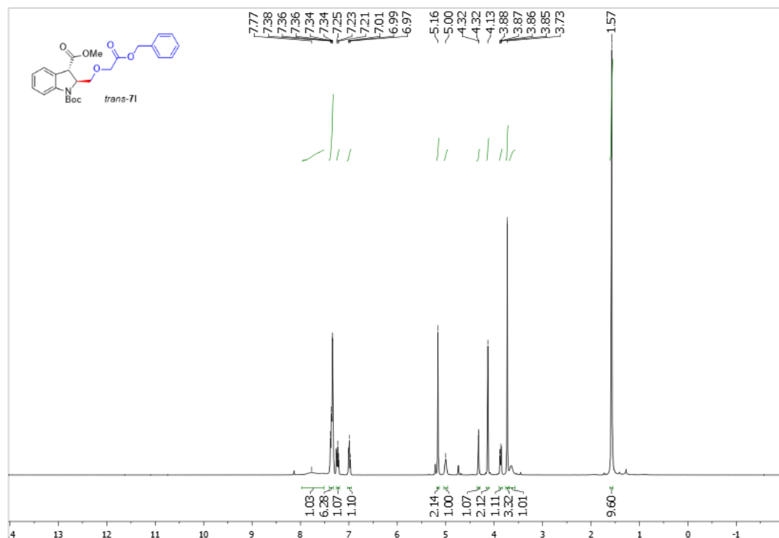
Supplementary Figure 168. 1 H NMR spectra of trans -71
