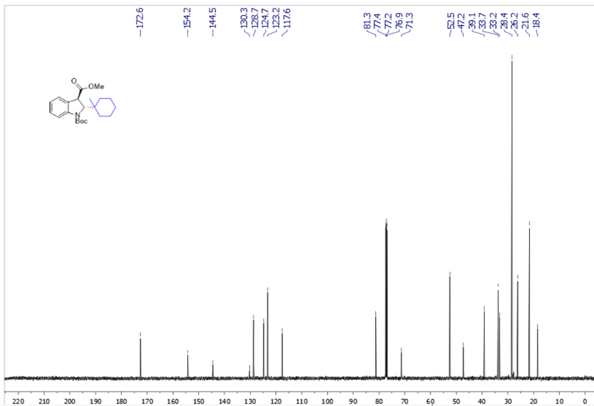
Supplementary Figure 124. ^{13}\text{C} NMR spectra of trans -3am
