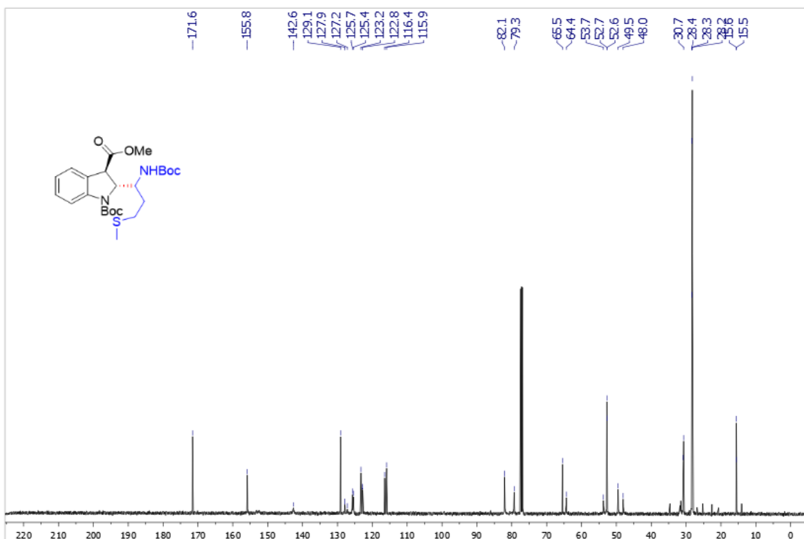
Supplementary Figure 102. 13 C NMR spectra of trans -3ab
