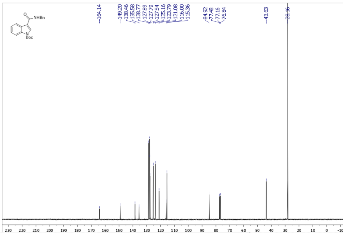
Supplementary Figure 3. ^1\text{H} NMR spectra of 1c
