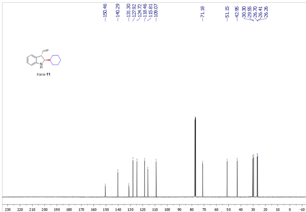
Supplementary Figure 192. 13 C NMR spectra of trans -11
