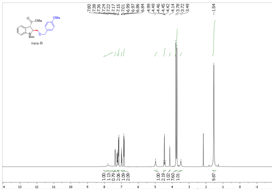
Supplementary Figure 162. 1 H NMR spectra of trans -7i
