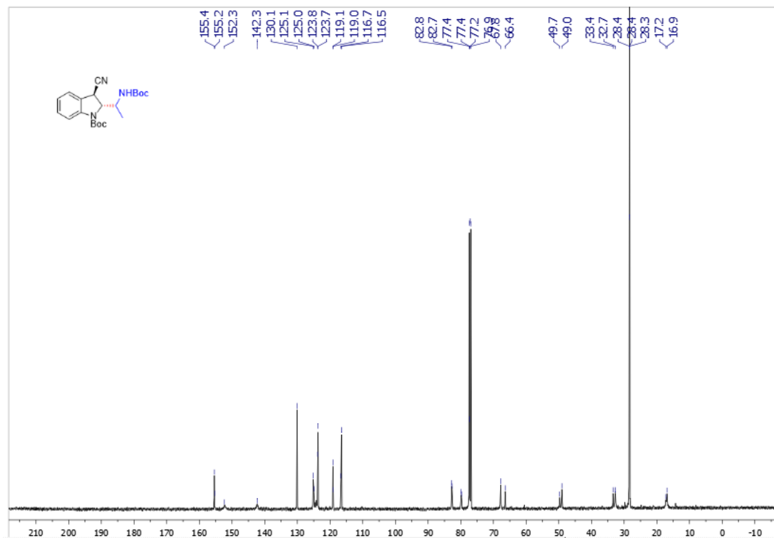
Supplementary Figure 55. ^1\text{H} NMR spectra of trans -3f
