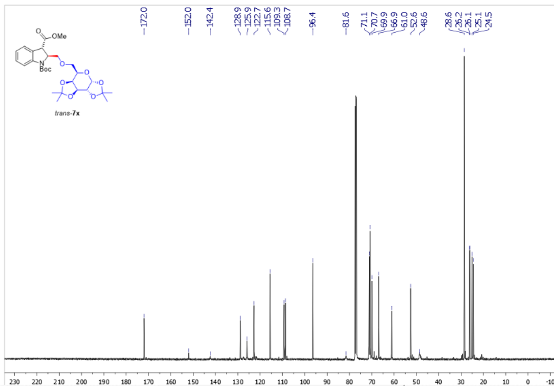
Supplementary Figure 177. 13 C NMR spectra of trans-7x
