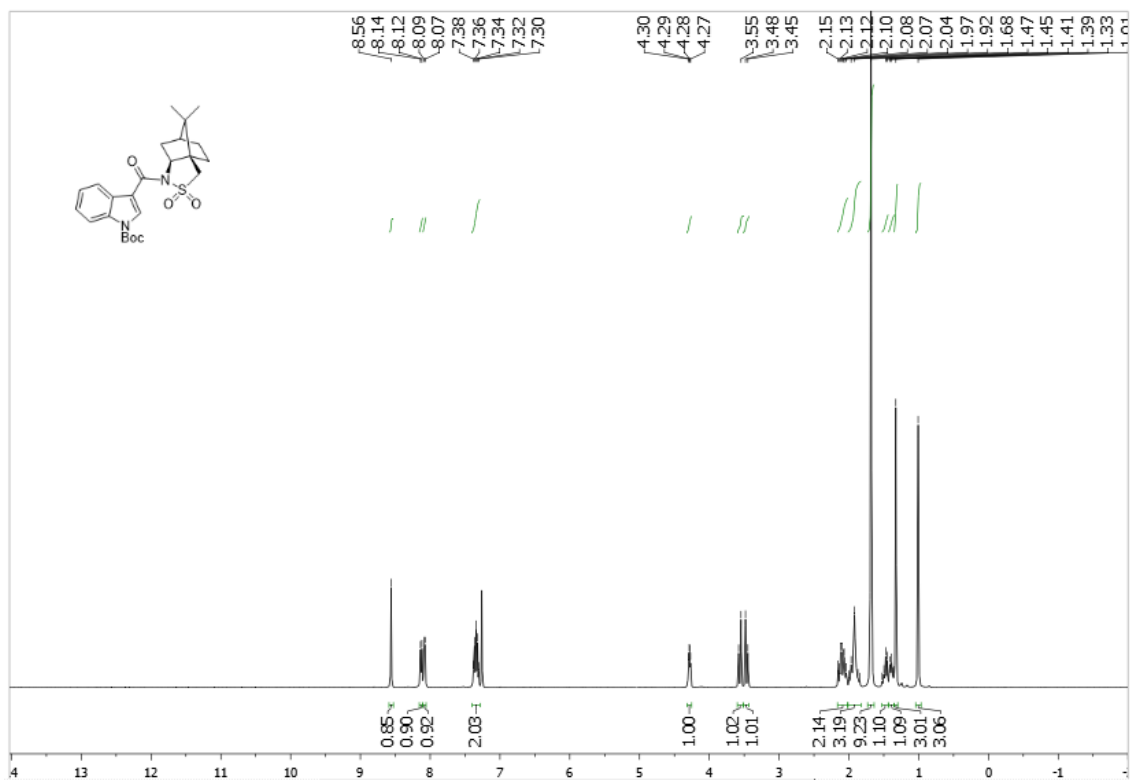
Supplementary Figure 37. ^1\text{H} NMR spectra of 5b
