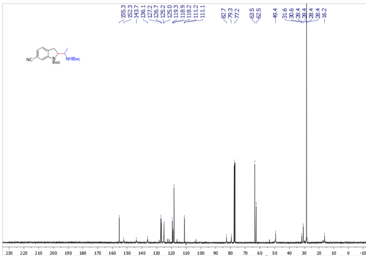
Supplementary Figure 74. ^{13}\text{C} NMR spectra of 30
