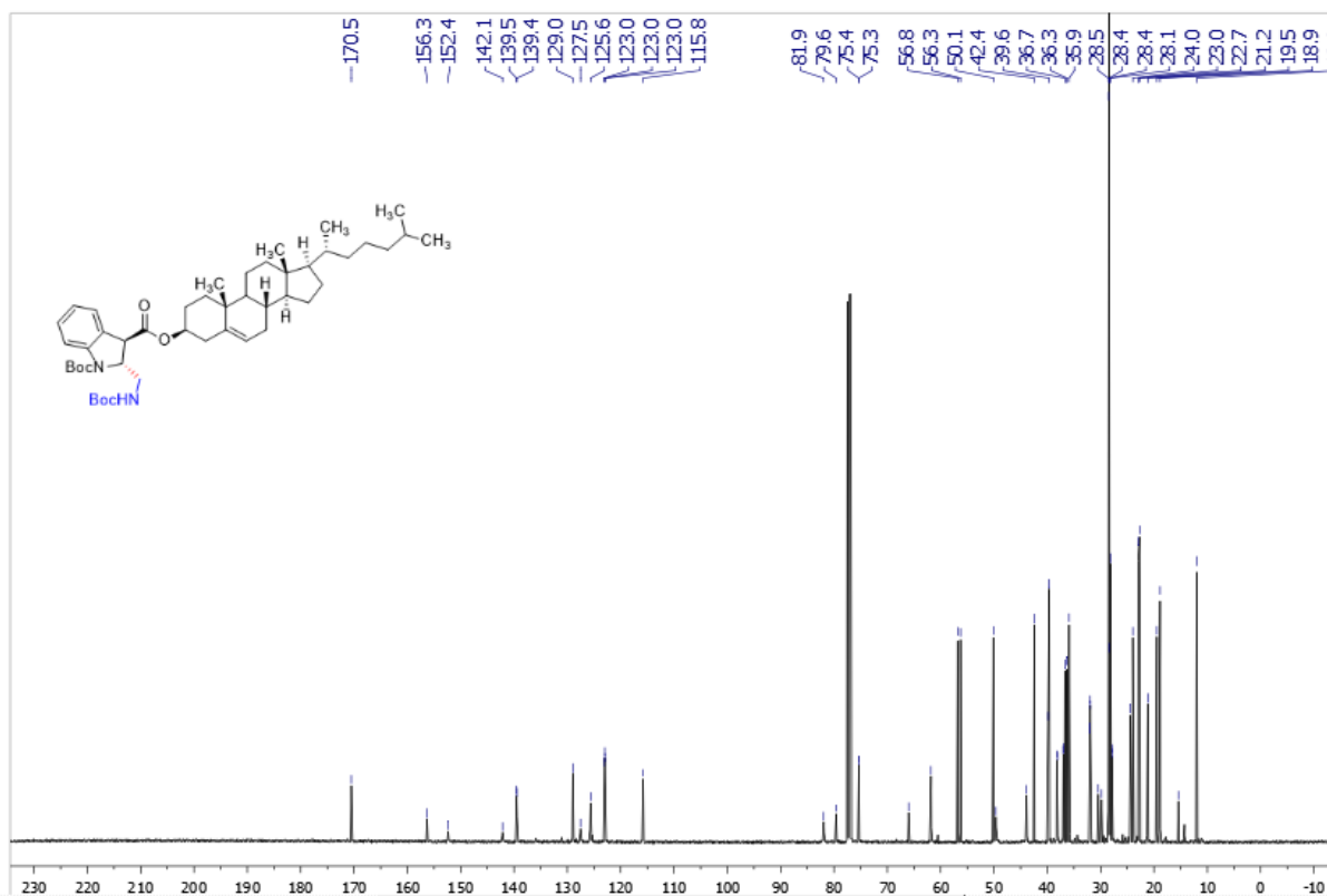
Supplementary Figure 144. 13 C NMR spectra of trans -3aw
