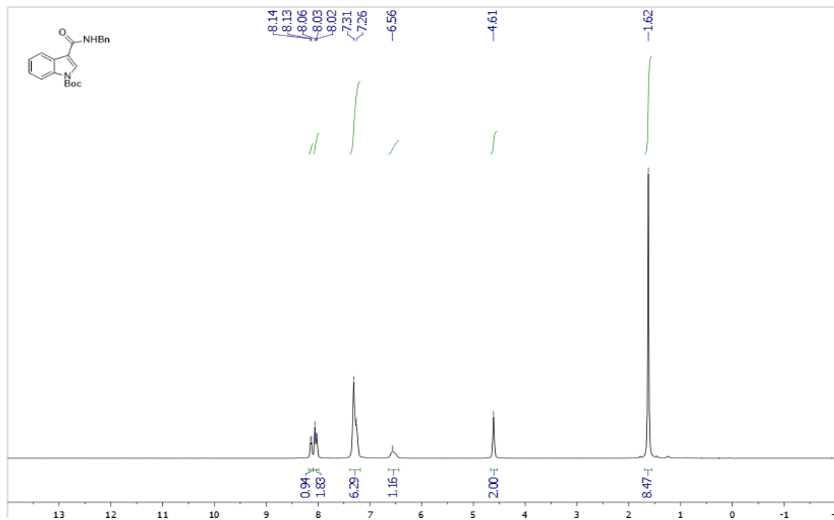
Supplementary Figure 3. ^1\text{H} NMR spectra of 1c
