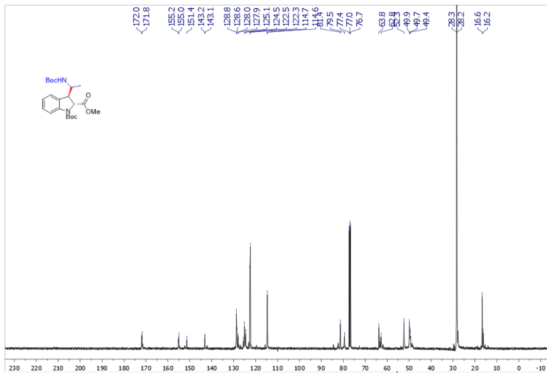
Supplementary Figure 80. ^{13}\text{C} NMR spectra of trans -3q
