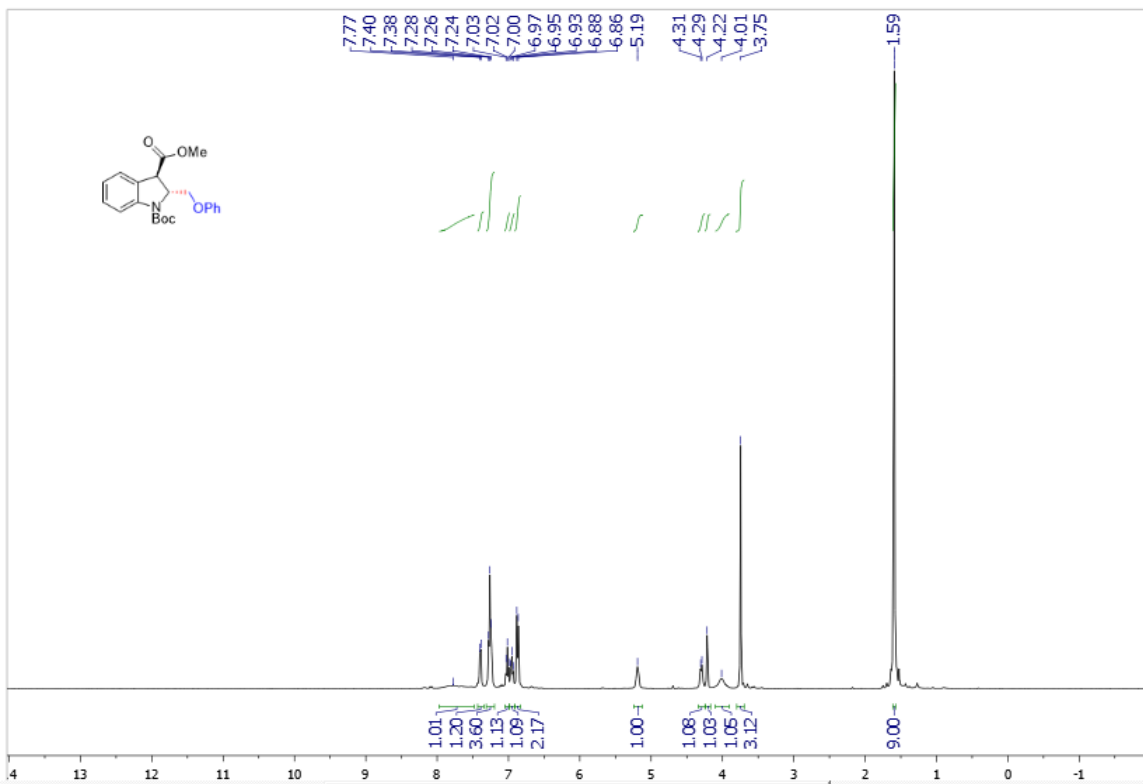
Supplementary Figure 113. ^1\text{H} NMR spectra of trans -3ah
