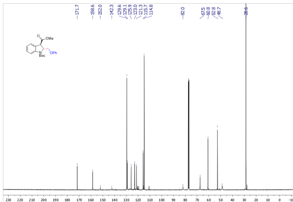
Supplementary Figure 114. ^{13}\text{C} NMR spectra of trans -3ah
