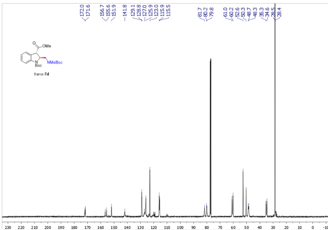
Supplementary Figure 157. ^{13}\text{C} NMR spectra of trans -7d
