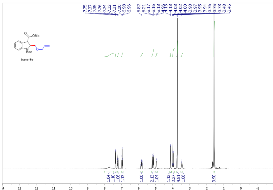
Supplementary Figure 158. 1 H NMR spectra of trans-7e
