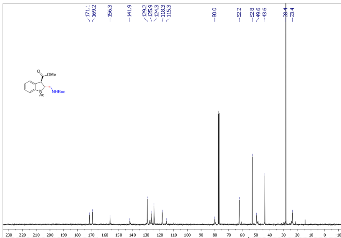
Supplementary Figure 64. ^{13}\text{C} NMR spectra of trans -3j
