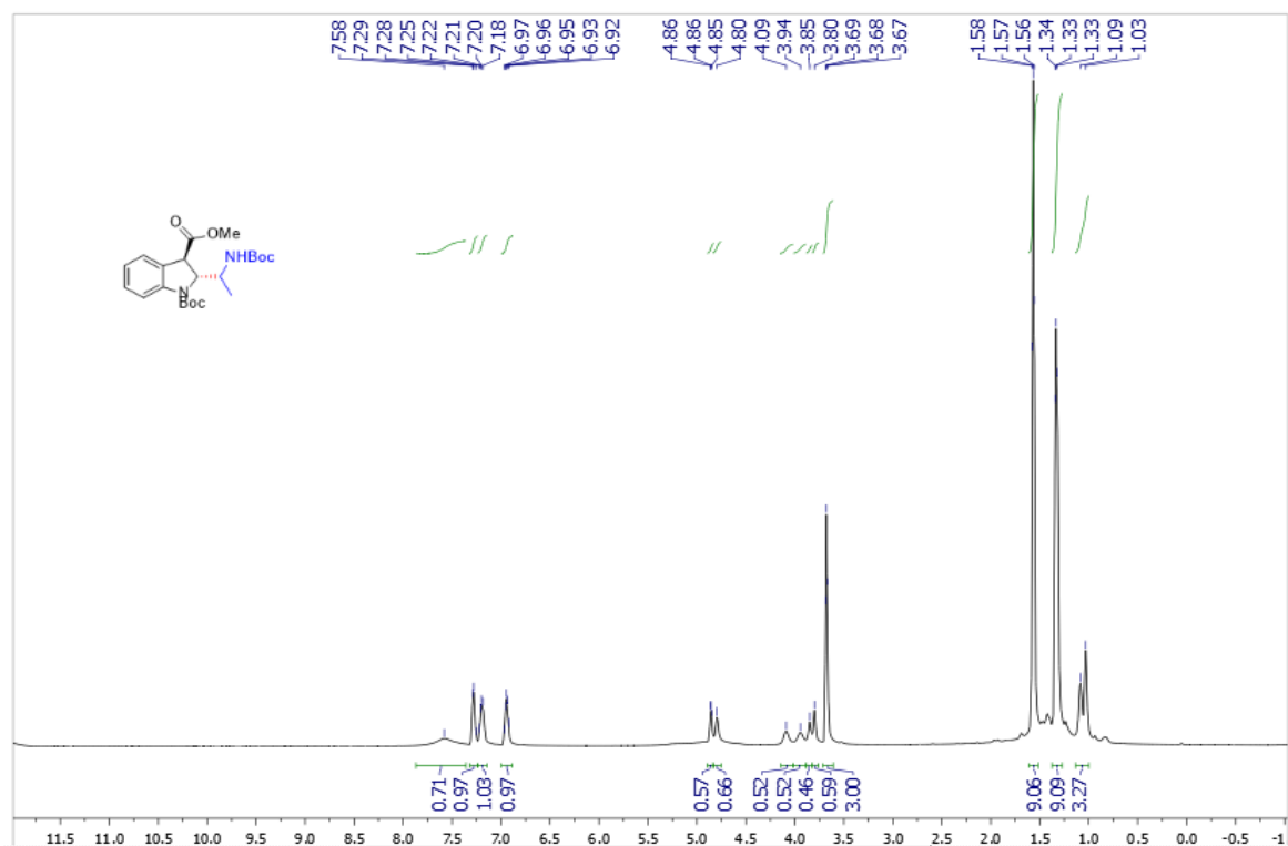
Supplementary Figure 39. ^1\text{H} NMR spectra of trans - 3a
