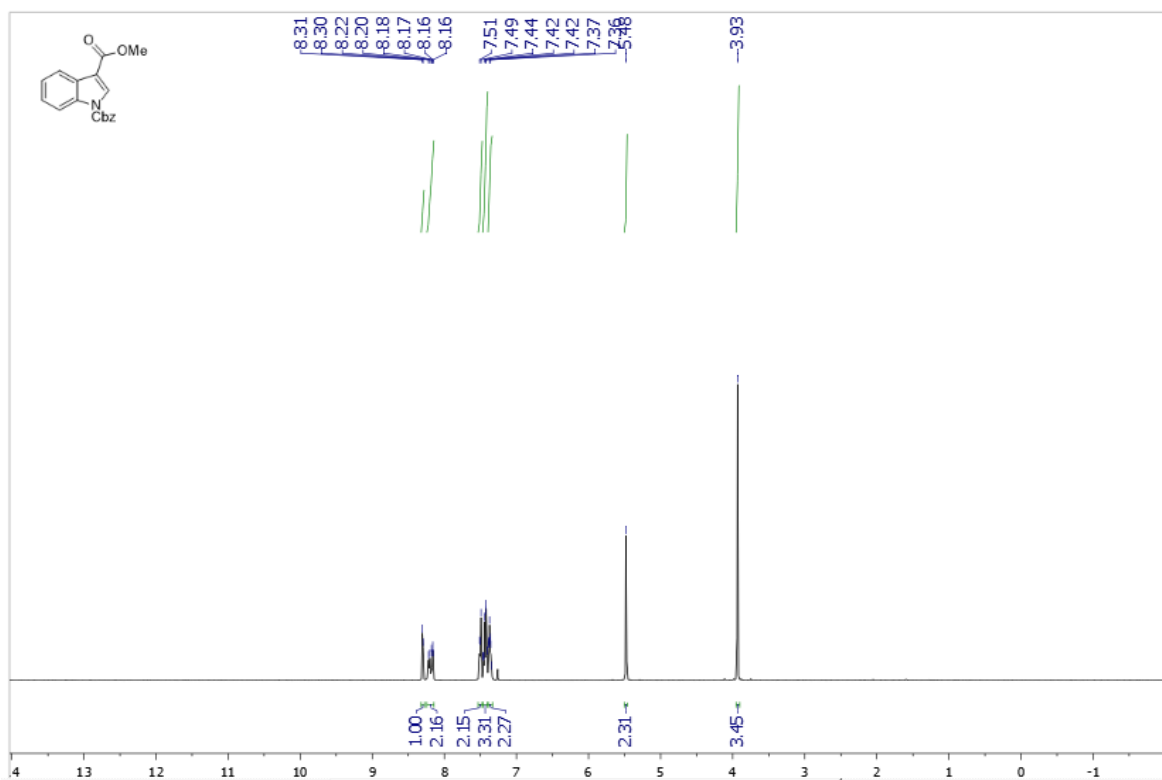
Supplementary Figure 13. ^1\text{H} NMR spectra of 1k
