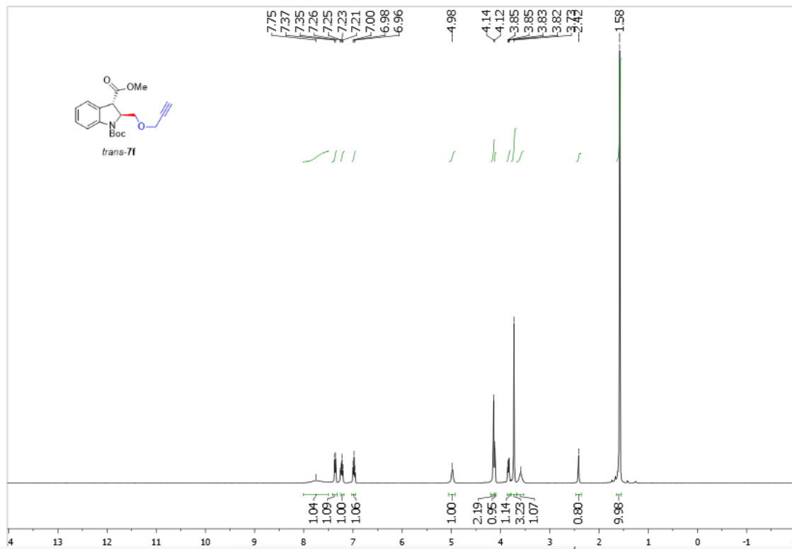
Supplementary Figure 160. ^1\text{H} NMR spectra of trans -7f
