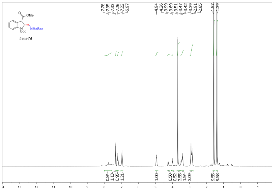
Supplementary Figure 156. ^1\text{H} NMR spectra of trans -7d
