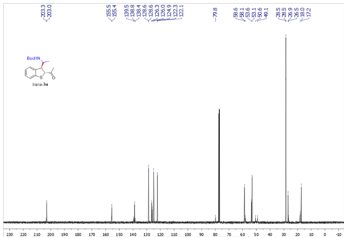
Supplementary Figure 88. ^{13}\text{C} NMR spectra of trans -3u
