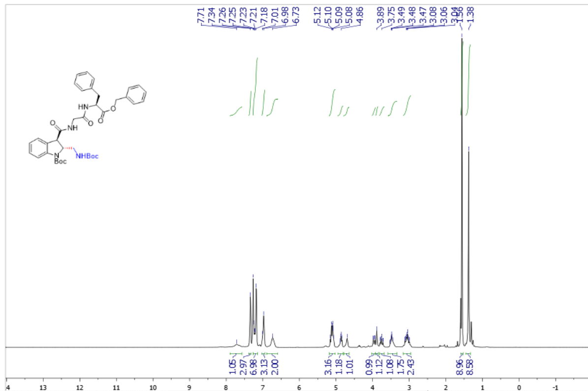
Supplementary Figure 141. 1 H NMR spectra of trans -3av
