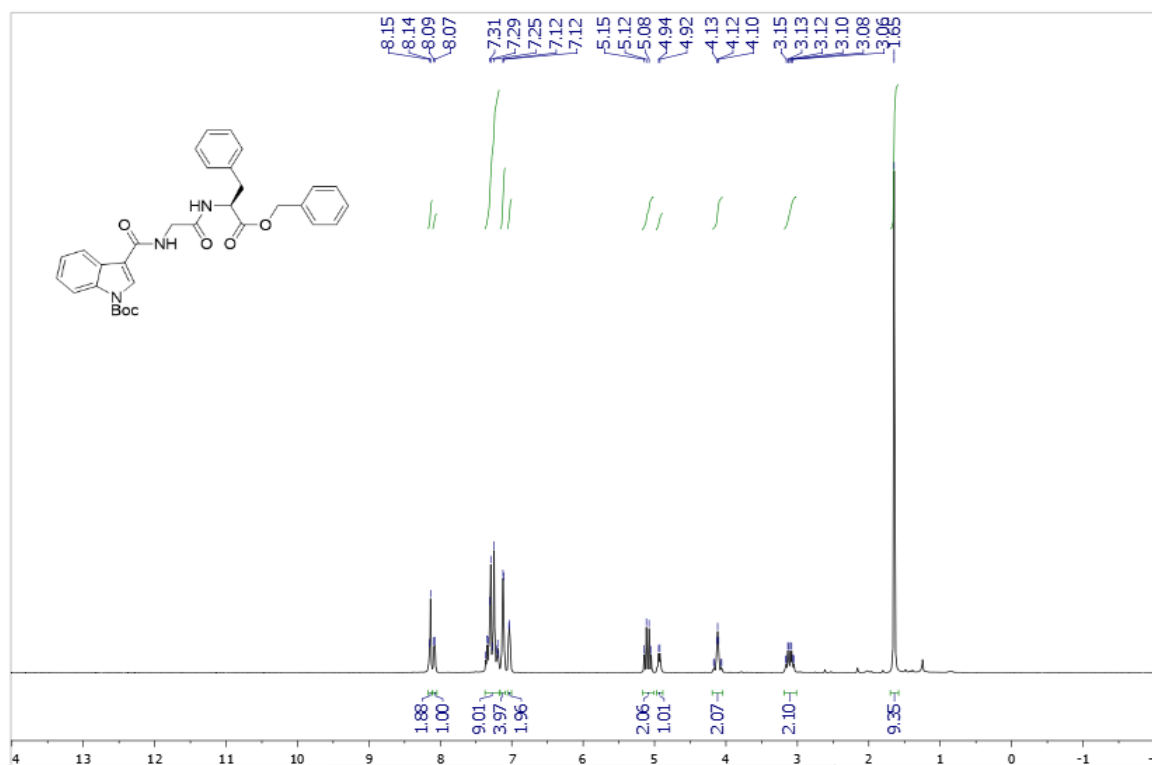
Supplementary Figure 31. ^1\text{H} NMR spectra of 1av
