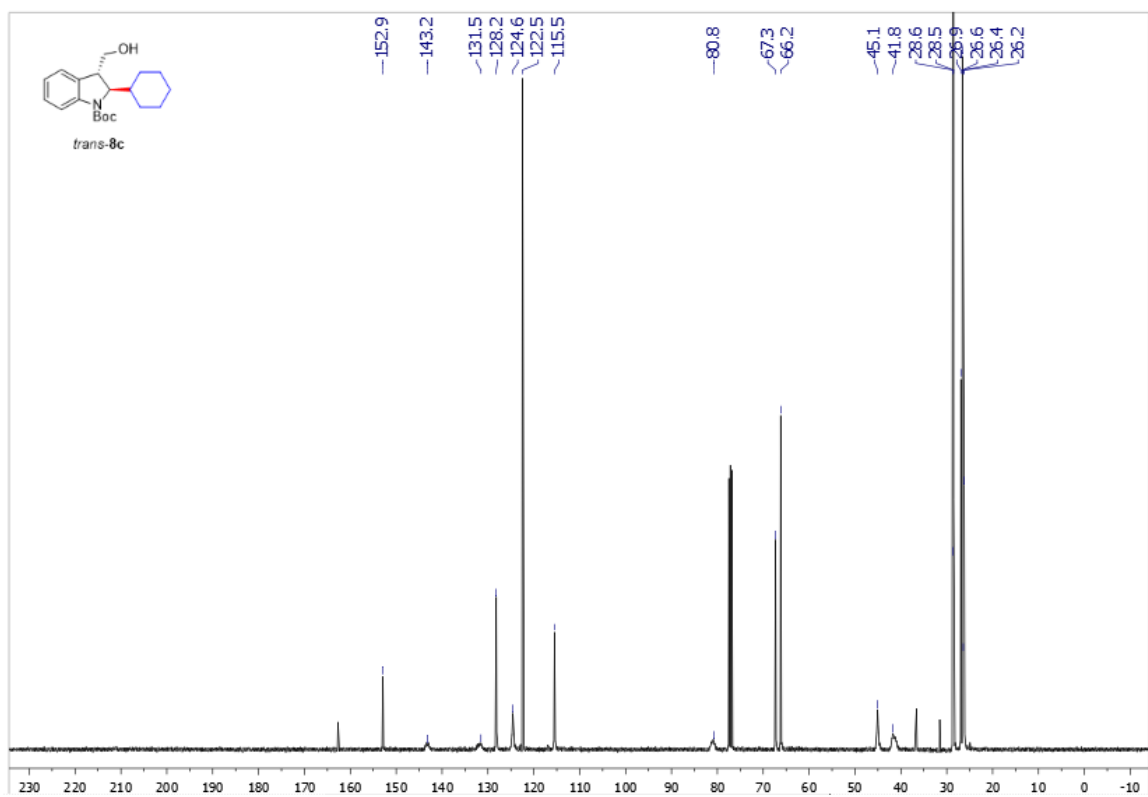
Supplementary Figure 186. 13 C NMR spectra of trans-8c
