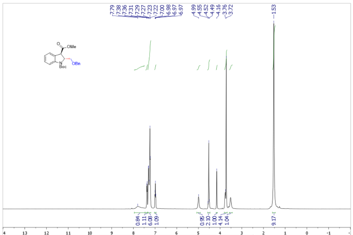
Supplementary Figure 111. ^1\text{H} NMR spectra of trans -3ag
