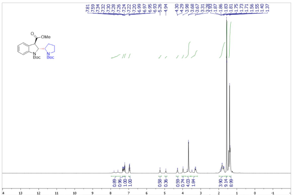
Supplementary Figure 103. ^1\text{H} NMR spectra of trans -3ac
