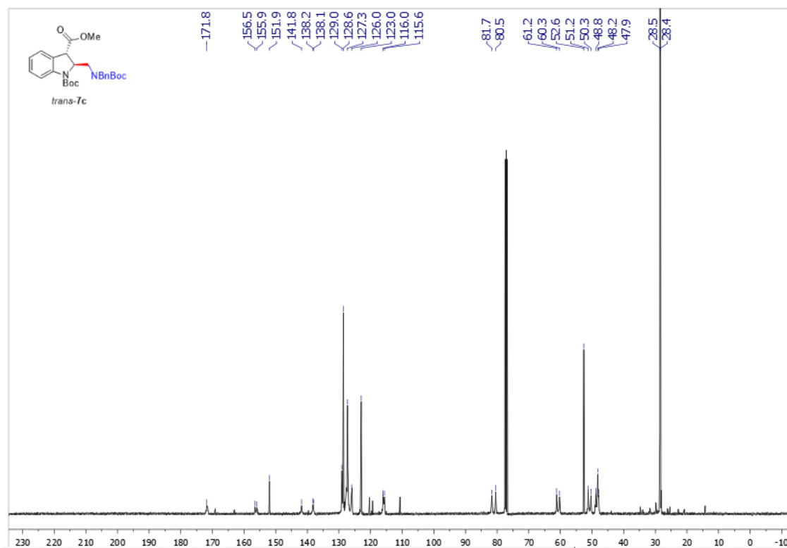
Supplementary Figure 155. 13 C NMR spectra of trans -7c
