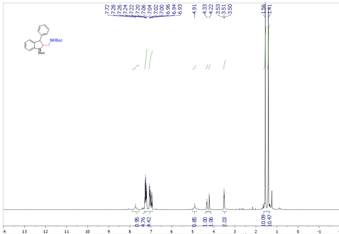
Supplementary Figure 77. ^1\text{H} NMR spectra of 3p-isomer-b
