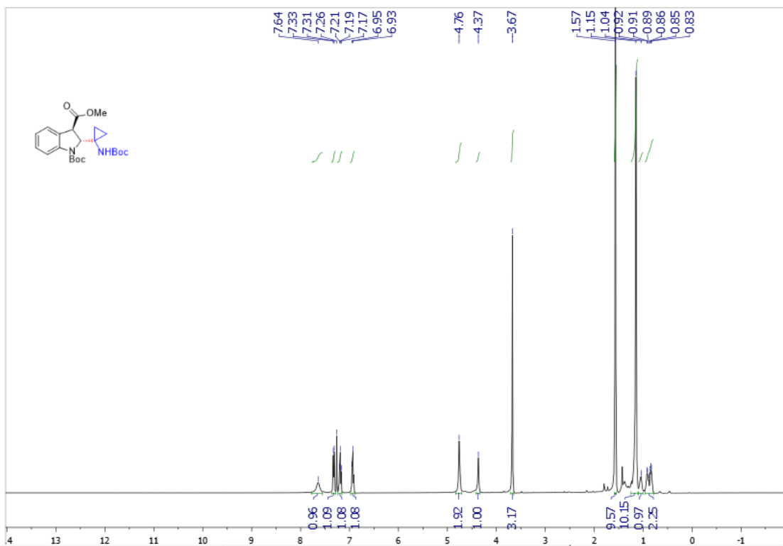
Supplementary Figure 107. ^1\text{H} NMR spectra of trans -3ae
