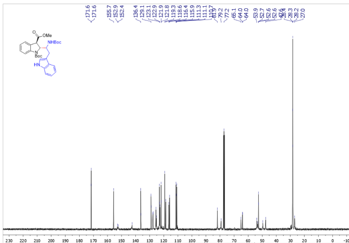
Supplementary Figure 94. ^{13}\text{C} NMR spectra of trans -3x
