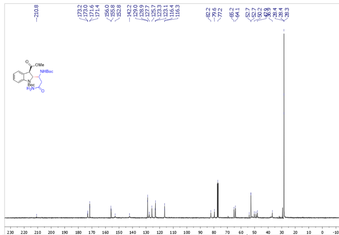
Supplementary Figure 100. 13 C NMR spectra of trans -3aa
