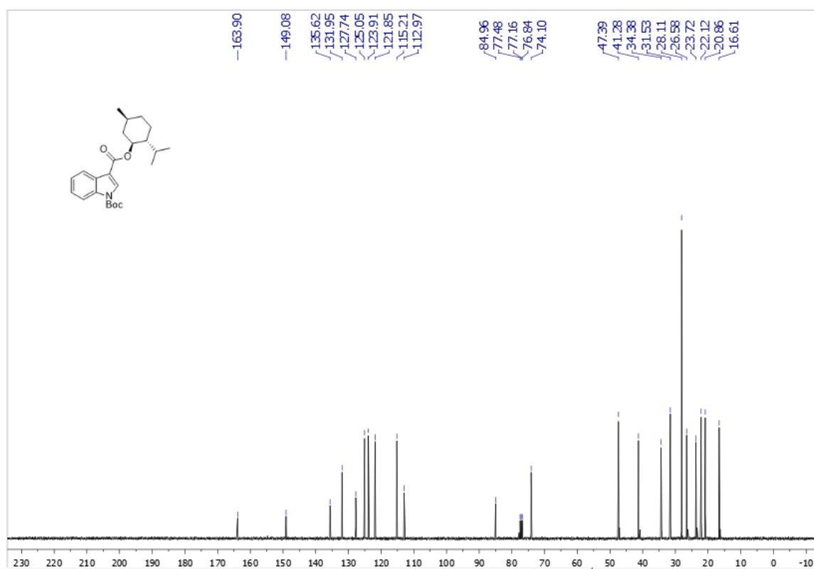
Supplementary Figure 25. ^1\text{H} NMR spectra of 1s
