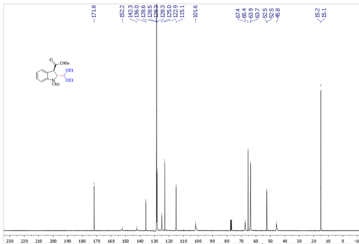
Supplementary Figure 116. ^{13}\text{C} NMR spectra of trans -3ai
