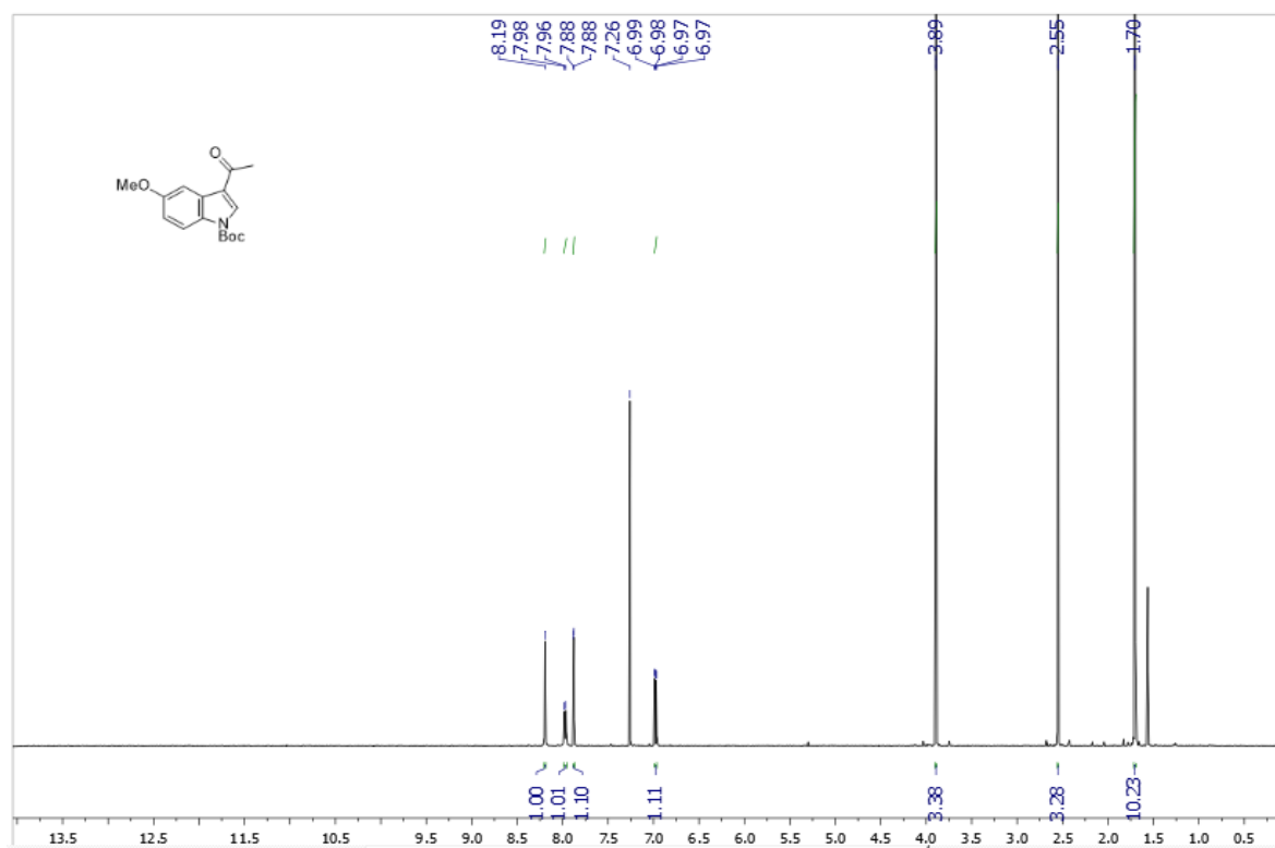
Supplementary Figure 19. ^1\text{H} NMR spectra of 1n
