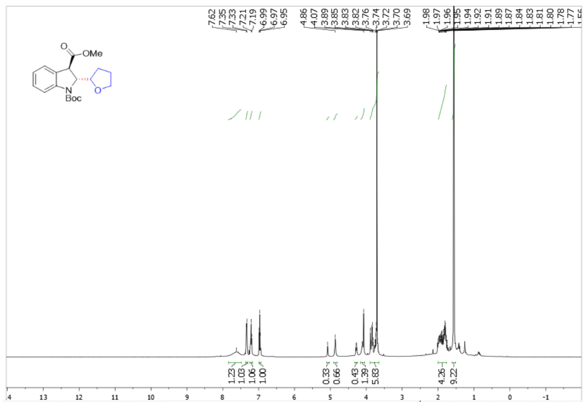
Supplementary Figure 109. ^1\text{H} NMR spectra of trans -3af
