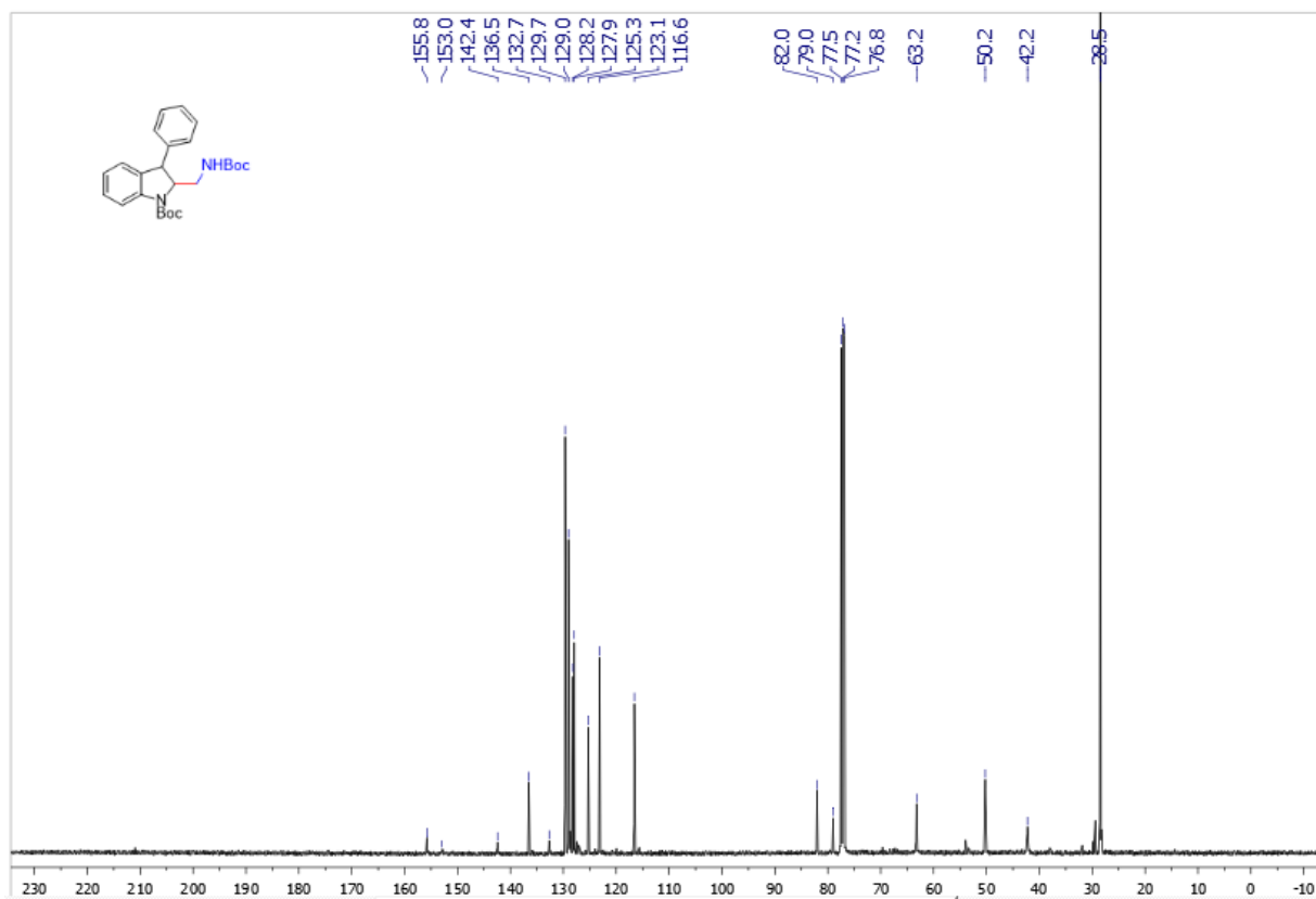
Supplementary Figure 76. 13 C NMR spectra of 3p-isomer-a
