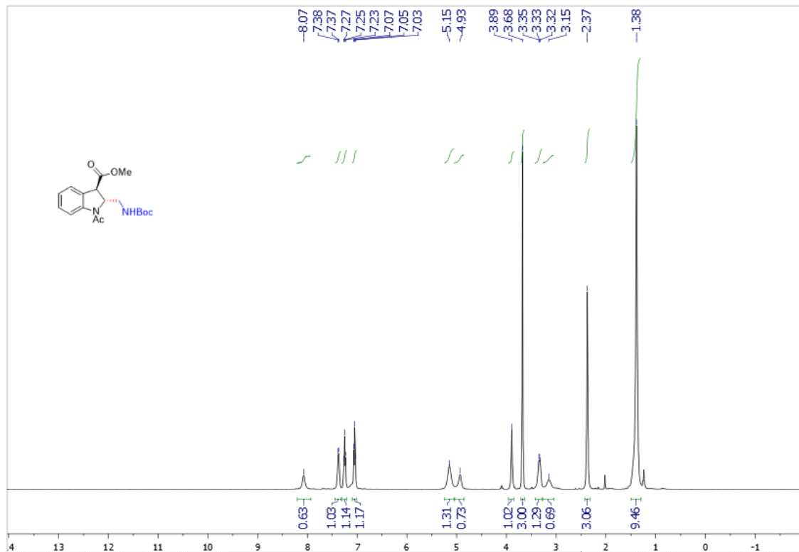
Supplementary Figure 63. ^1\text{H} NMR spectra of trans -3j
