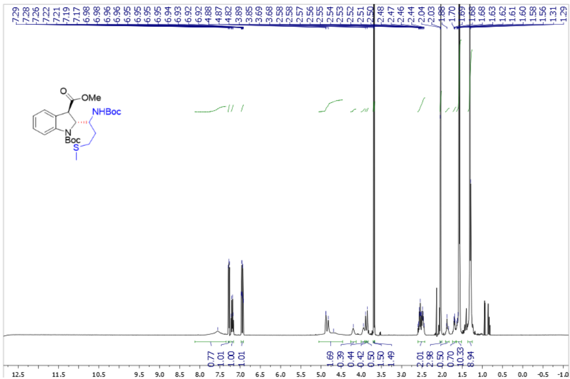
Supplementary Figure 101. 1 H NMR spectra of trans -3ab
