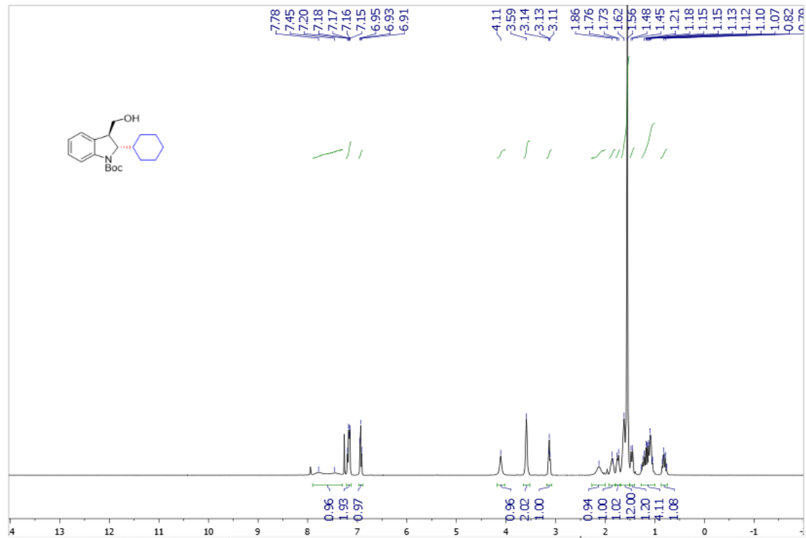
Supplementary Figure 150. ^1\text{H} NMR spectra of trans -4aj
