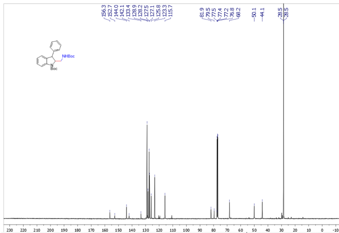
Supplementary Figure 78. ^{13}\text{C} NMR spectra of 3p-isomer-b
