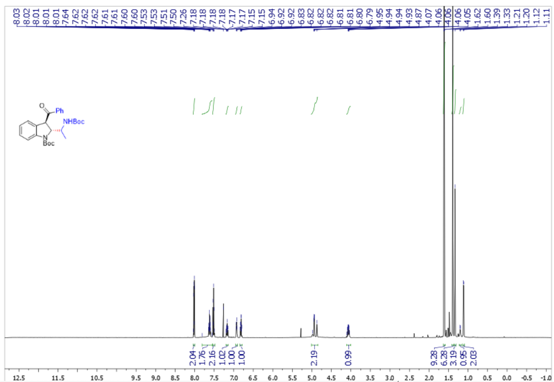
Supplementary Figure 53. ^1\text{H} NMR spectra of trans -3e
