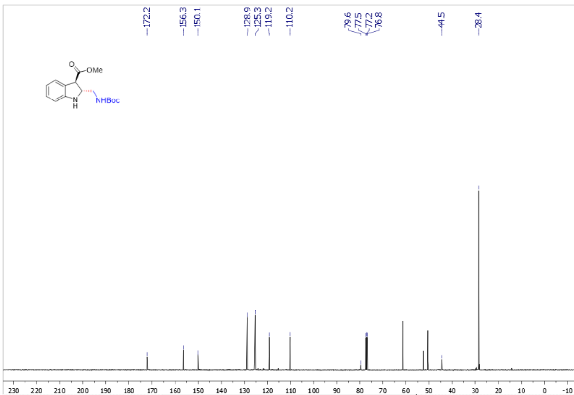
Supplementary Figure 149. ^{13}\text{C} NMR spectra of trans -4k
