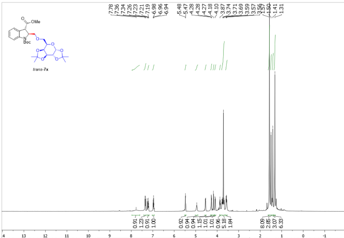
Supplementary Figure 176. 1 H NMR spectra of trans-7x
