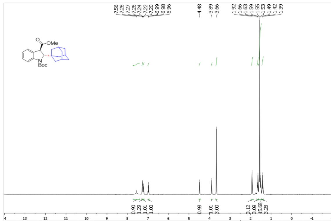
Supplementary Figure 129. 1 H NMR spectra of trans -3ap
