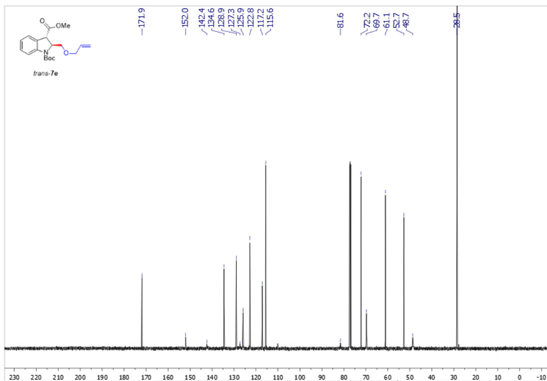
Supplementary Figure 159. 13 C NMR spectra of trans-7e
