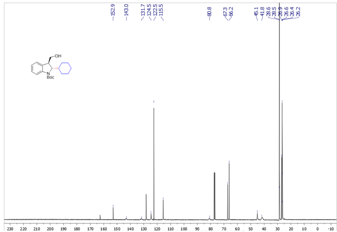
Supplementary Figure 151. ^{13}\text{C} NMR spectra of trans -4aj
