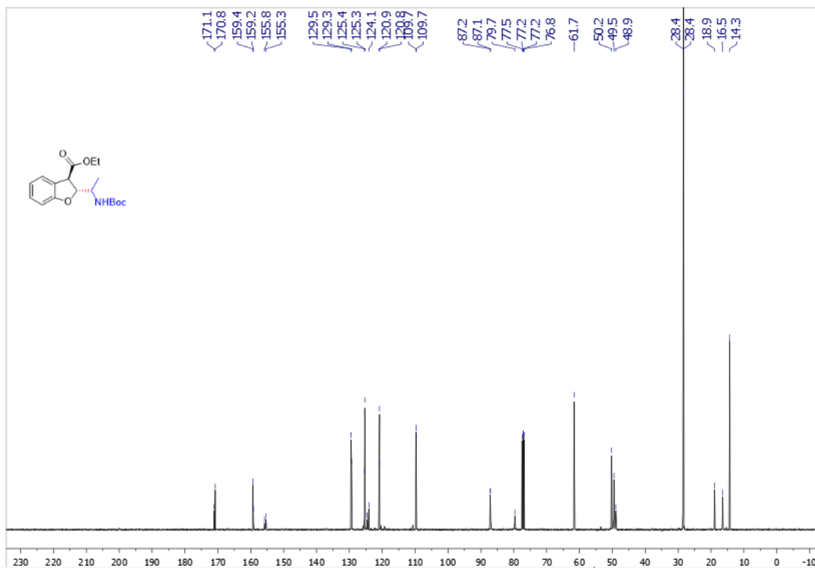
Supplementary Figure 86. ^{13}\text{C} NMR spectra of trans -3t
