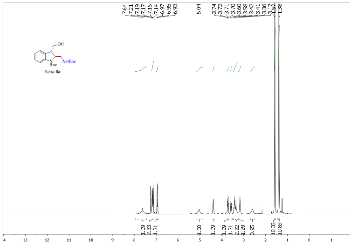
Supplementary Figure 181. 1 H NMR spectra of trans -8a
