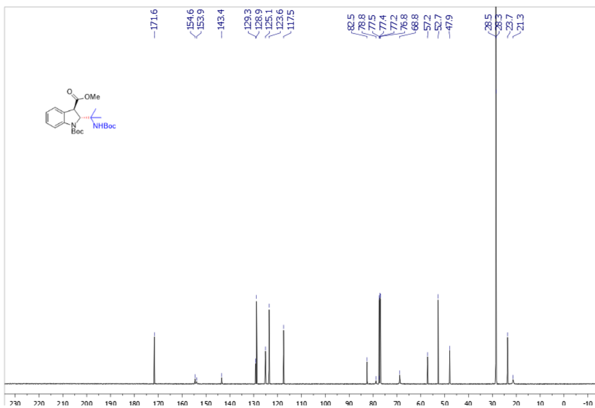
Supplementary Figure 106. ^{13}\text{C} NMR spectra of trans -3ad
