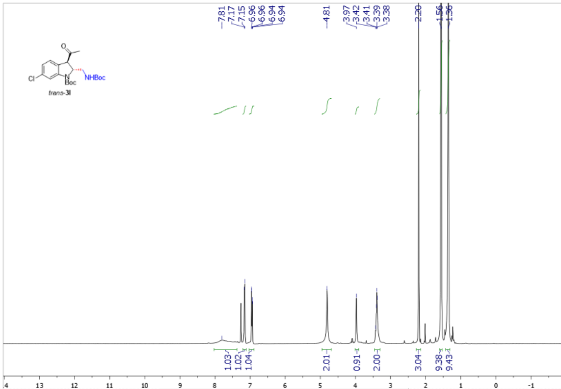
Supplementary Figure 67. 1 H NMR spectra of trans -31
