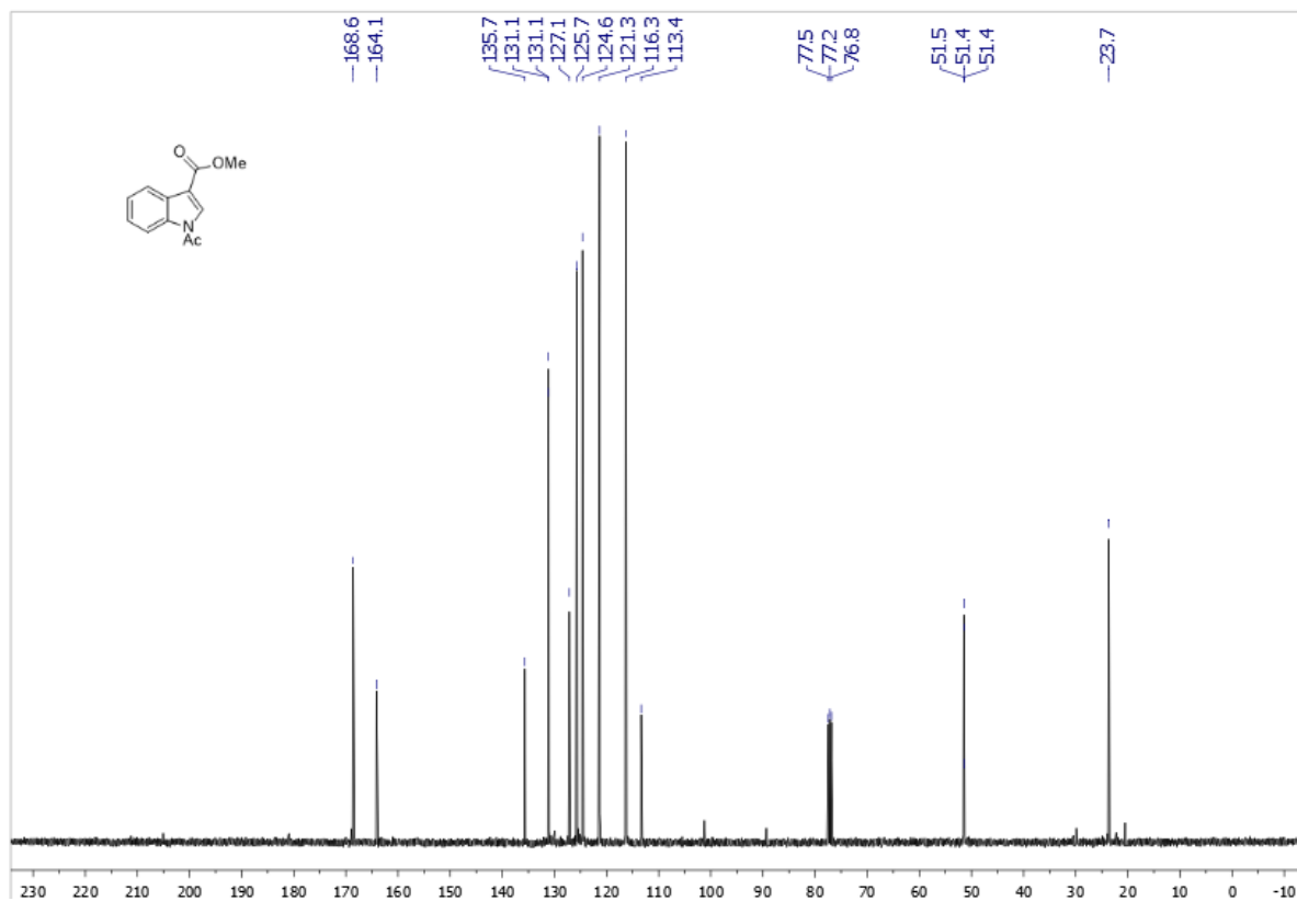
Supplementary Figure 11. ^1\text{H} NMR spectra of 1j
