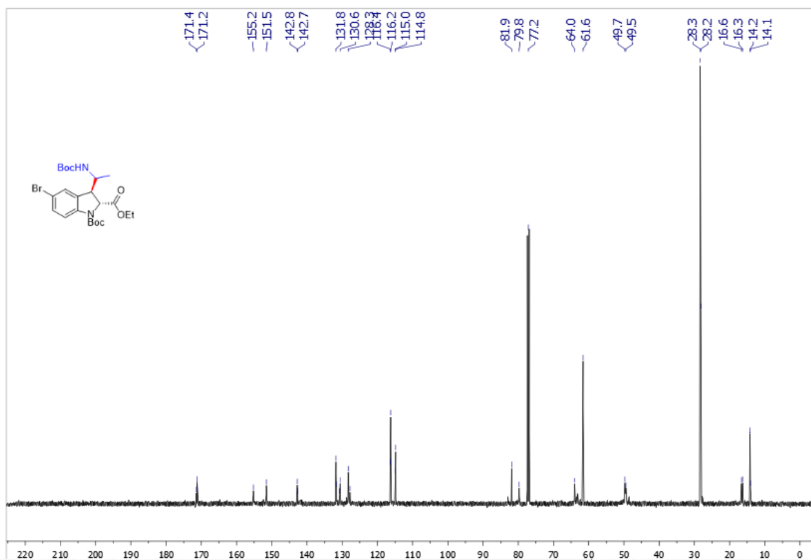
Supplementary Figure 82. 13 C NMR spectra of trans -3r
