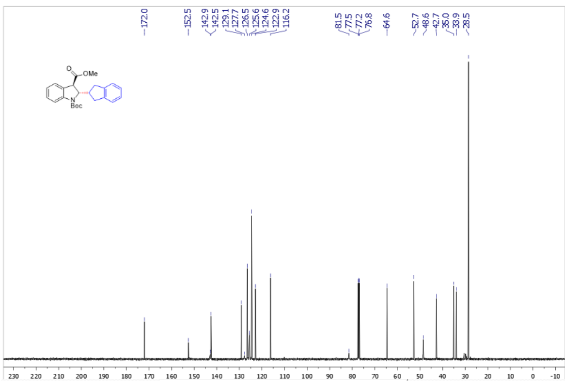
Supplementary Figure 120. ^{13}\text{C} NMR spectra of trans -3ak
