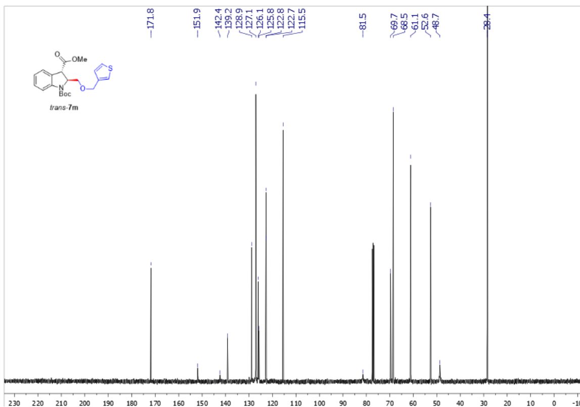
Supplementary Figure 171. 13 C NMR spectra of trans -7m
