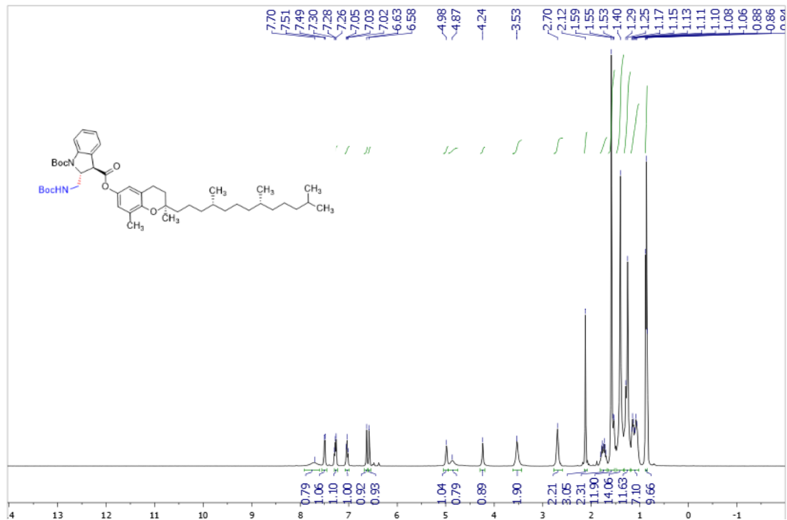
Supplementary Figure 145. 1 H NMR spectra of trans -3ax
