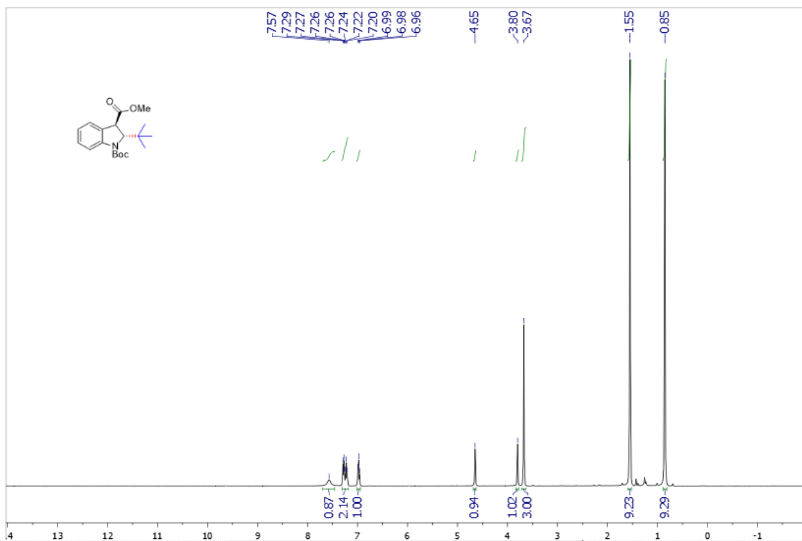
Supplementary Figure 121. ^1\text{H} NMR spectra of trans -3al
