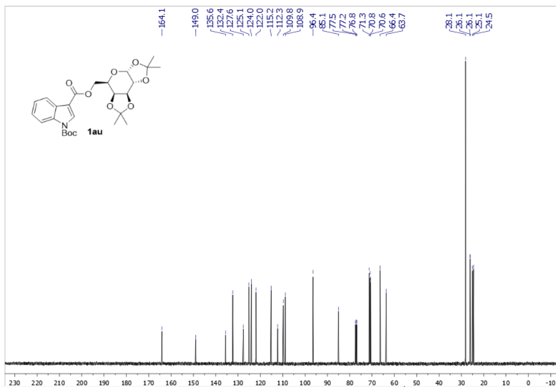
Supplementary Figure 29. ^1\text{H} NMR spectra of 1au
