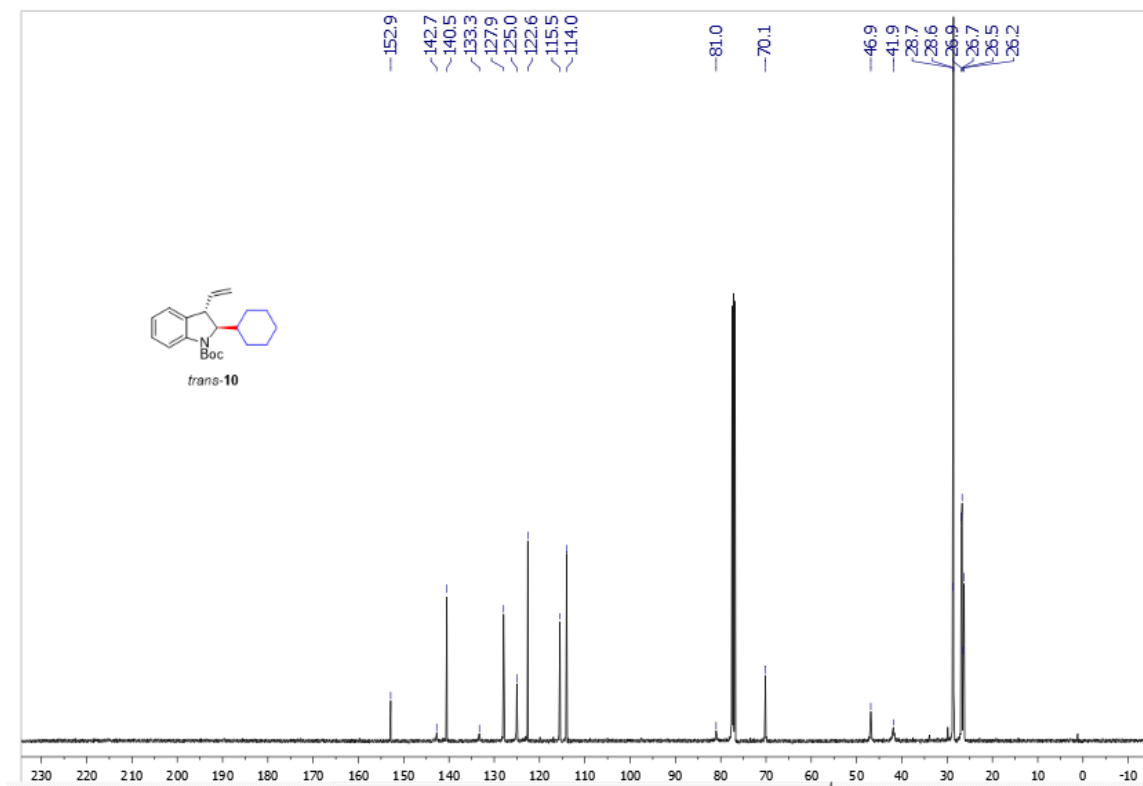
Supplementary Figure 190. ^{13}\text{C} NMR spectra of trans -10
