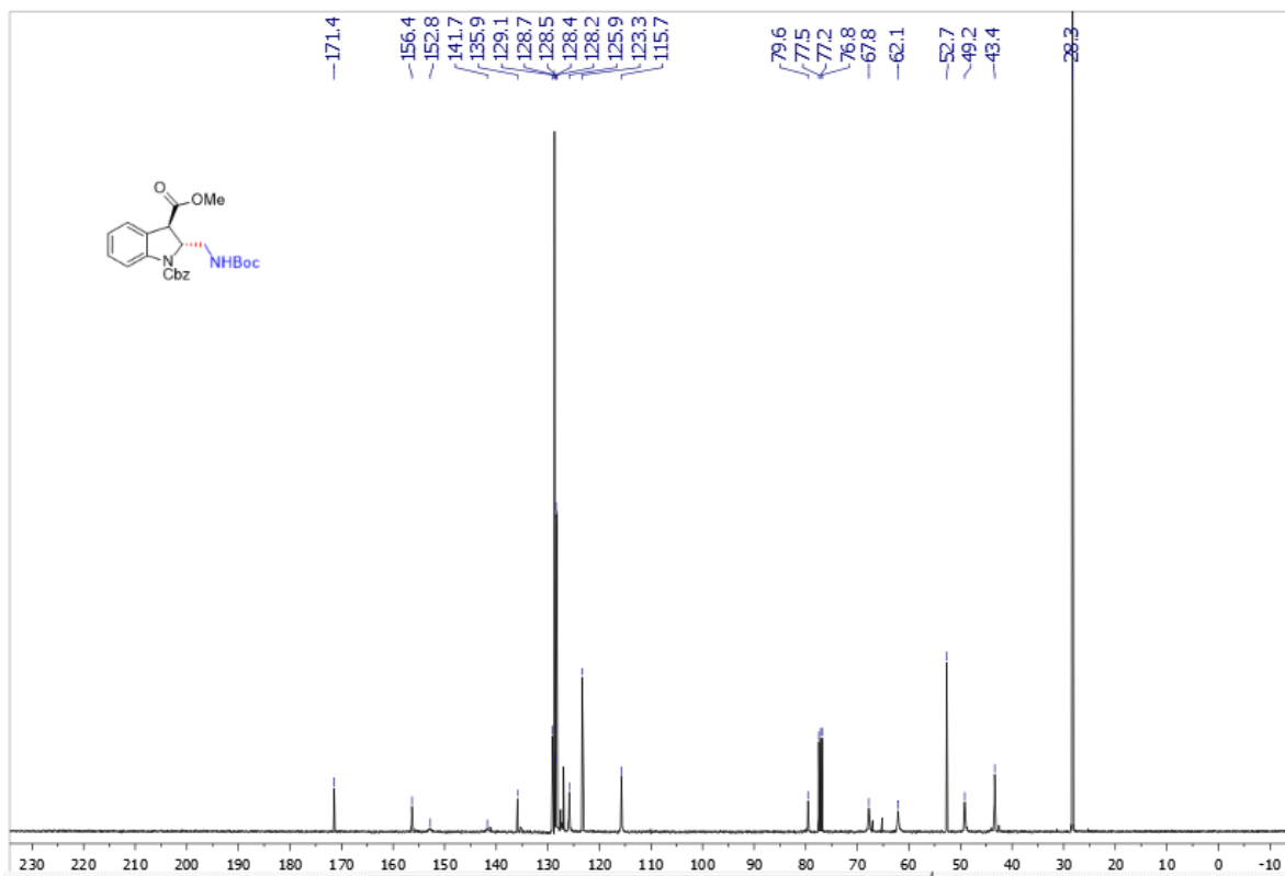
Supplementary Figure 66. ^{13}\text{C} NMR spectra of trans -3k
