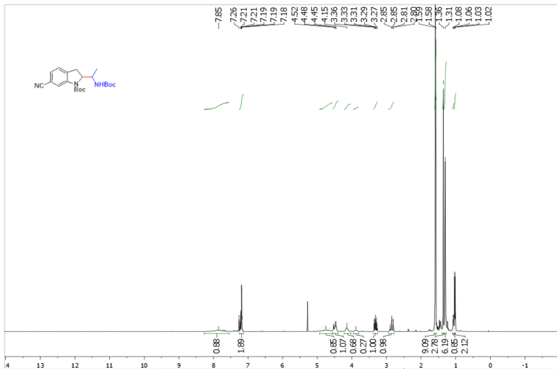
Supplementary Figure 73. ^1\text{H} NMR spectra of 30
