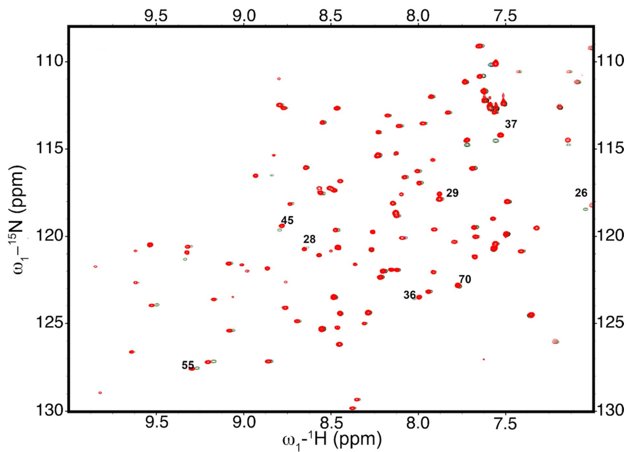
Figure S1 ^{15}\text{N} -HSQC of protein \pm Fe.
