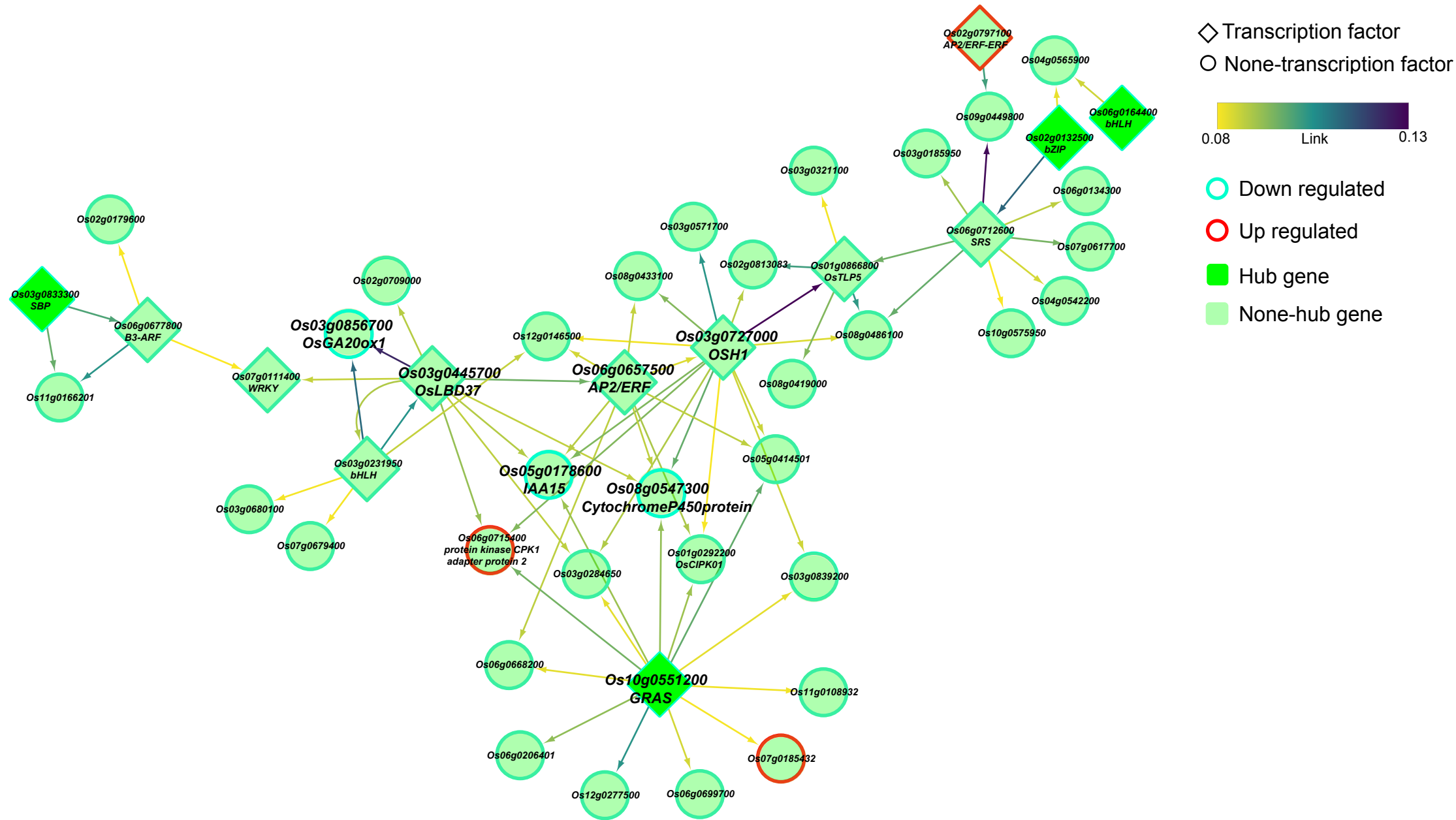
Fig. S13. The regulatory network in the green module. Transcription factors are annotated with symbols or family names; descriptions of target genes regulated by more than two transcription factors are annotated.
