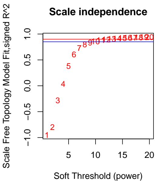
Fig. S3. R^2 and mean connectivity calculation of soft threshold.
