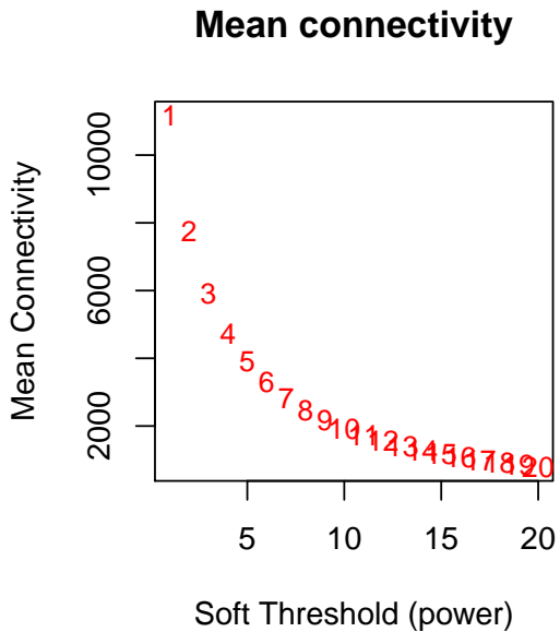
Fig. S3. R^2 and mean connectivity calculation of soft threshold.
