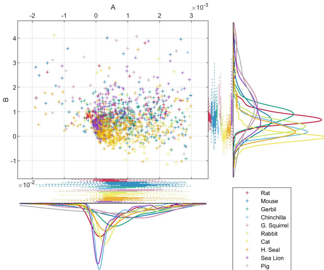
S9 Fig. Individual variation in the linear Cesàro model. The optimized coefficients A and B in the linear Cesàro equation \kappa(s)=As+B , are presented in a 2D scatter plot. Plotting conventions are identical to S7 Fig.
