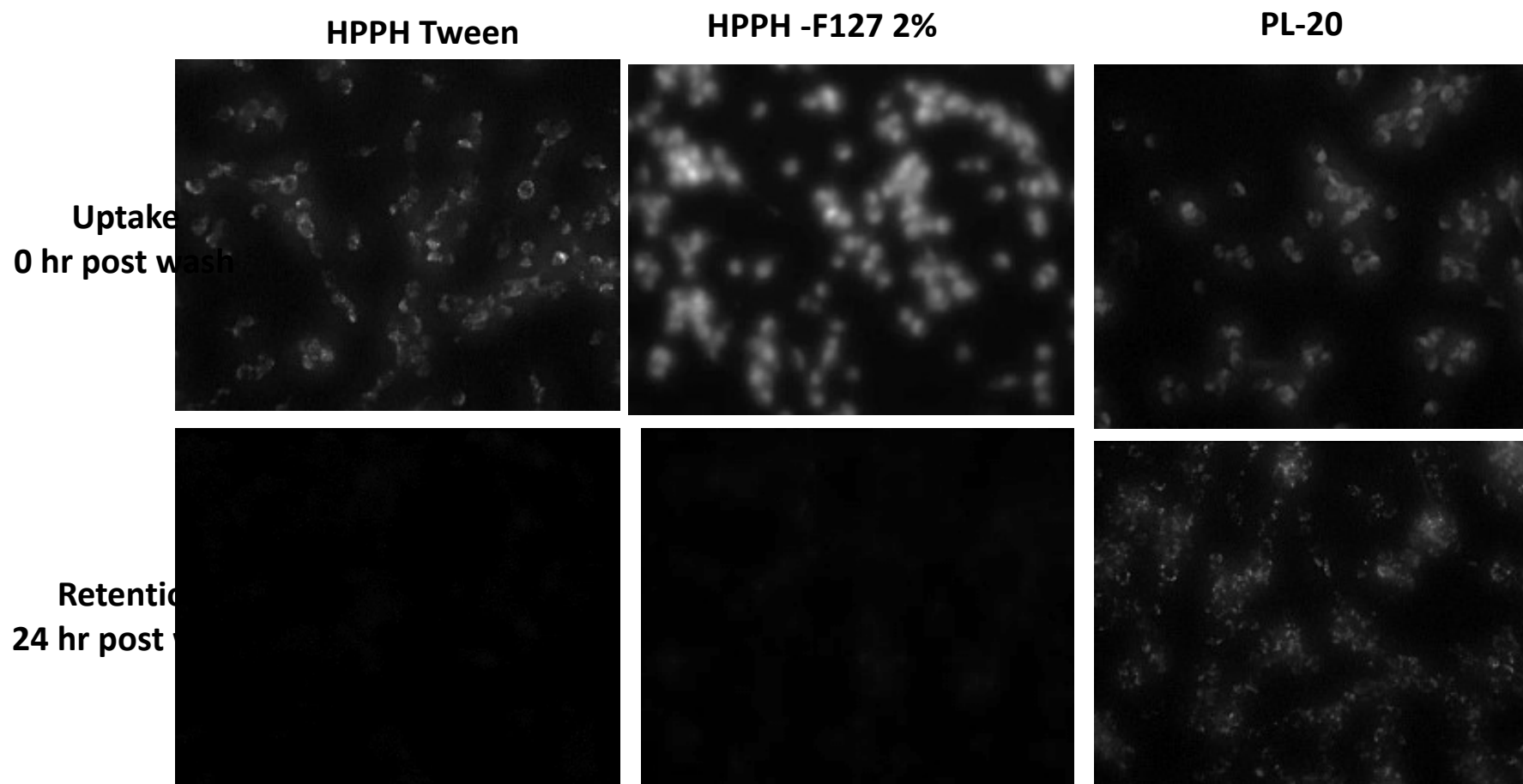
Figure S1: Tumor-uptake and retention of HPPH formulated in various delivery vehicles
