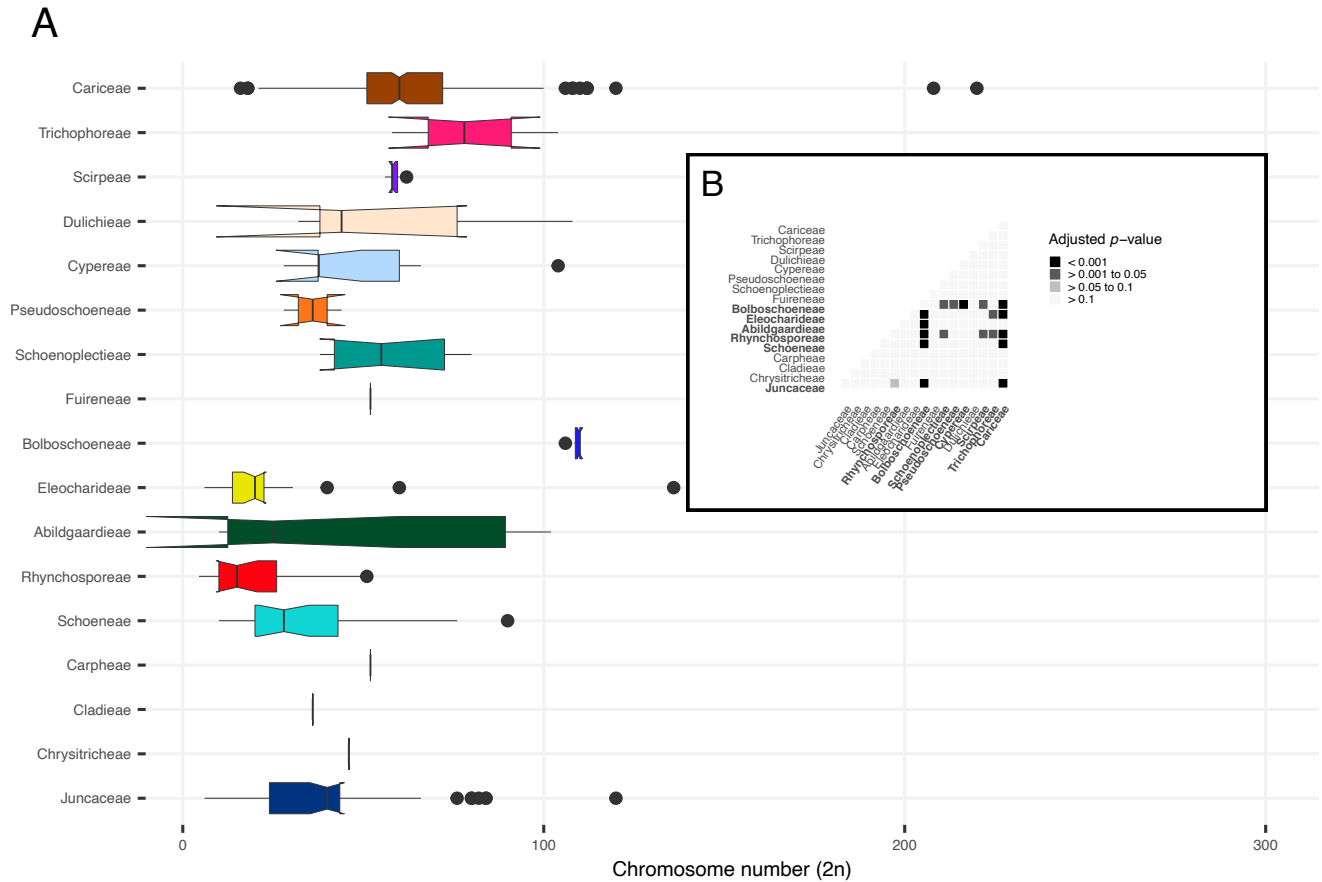
FIG. S4. Chromosome number (2n) across cyperids divided into 16 tribes of Cyperaceae, as well as the Juncaceae family (A). Major clades are represented by the same colours as in Fig. S1 and are presented in the same order as in the phylogeny shown in Fig. S2. Solid lines represent median values for the clades, outlying data are indicated by circles and lower and upper hinges correspond to the first and third quartiles, respectively.
