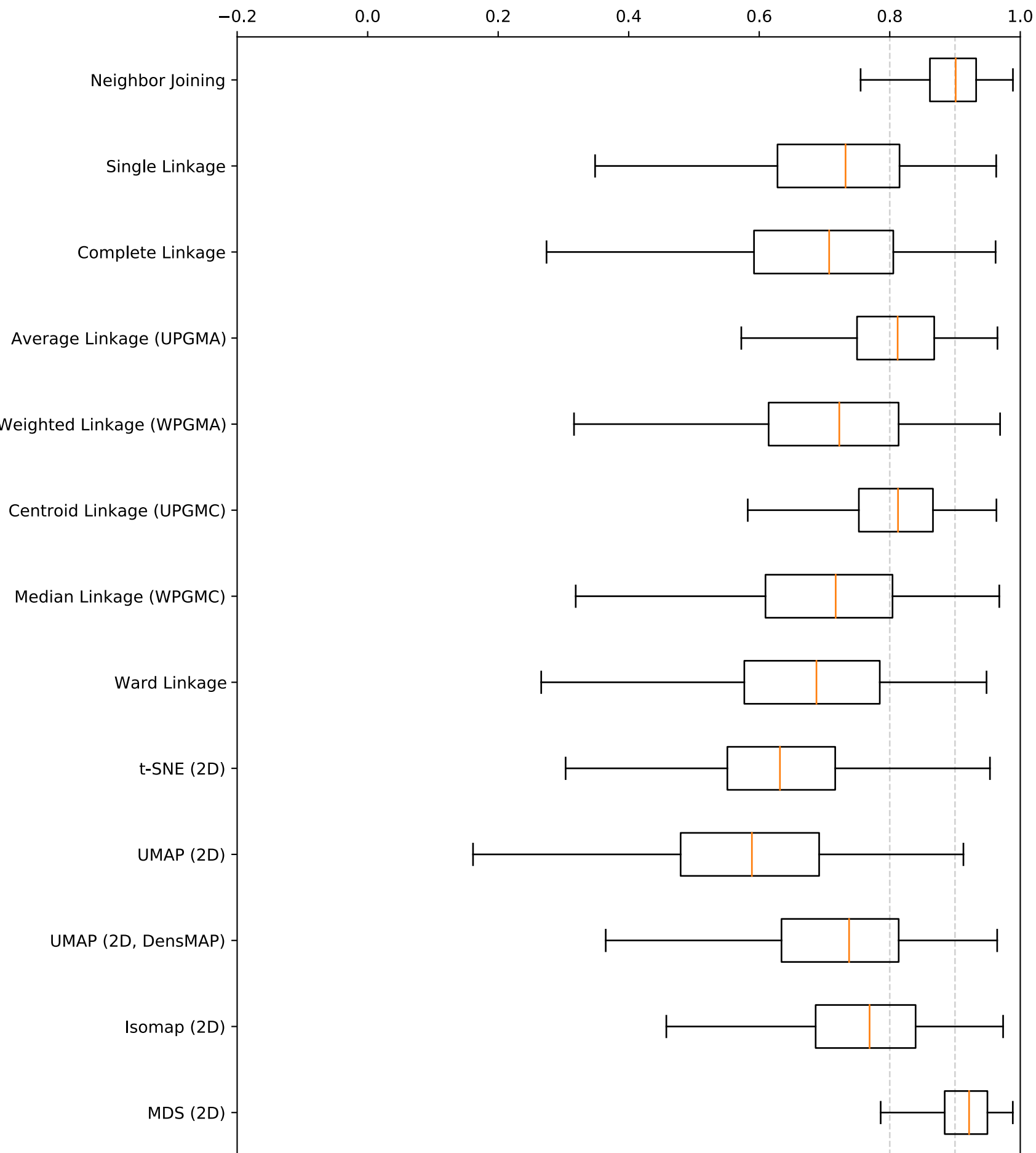
Spearman
