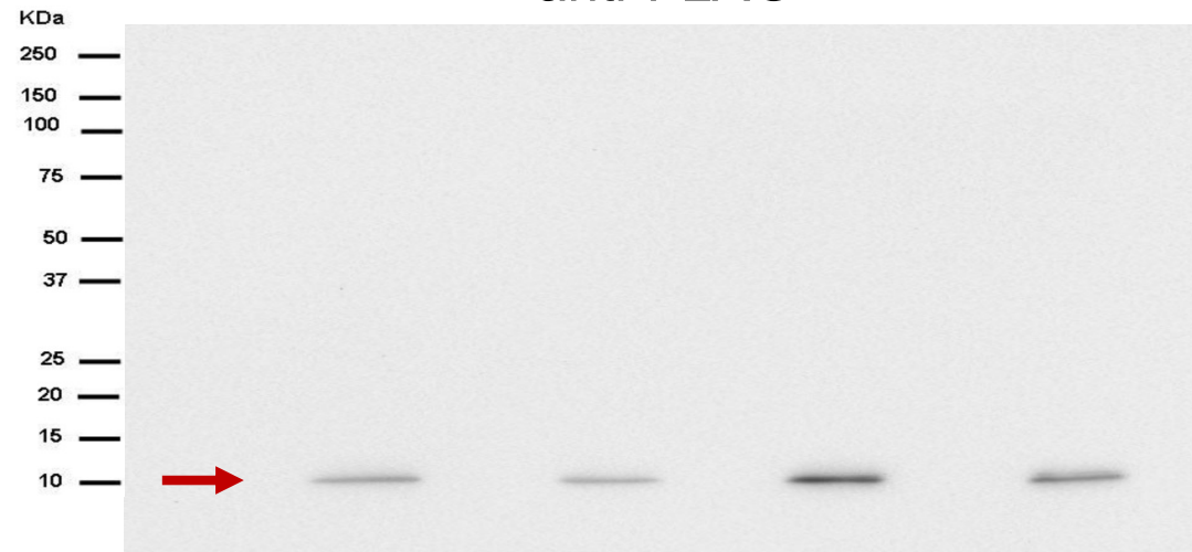
anti-FLAG
