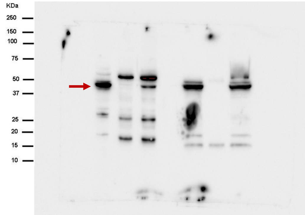
anti-FLAG
