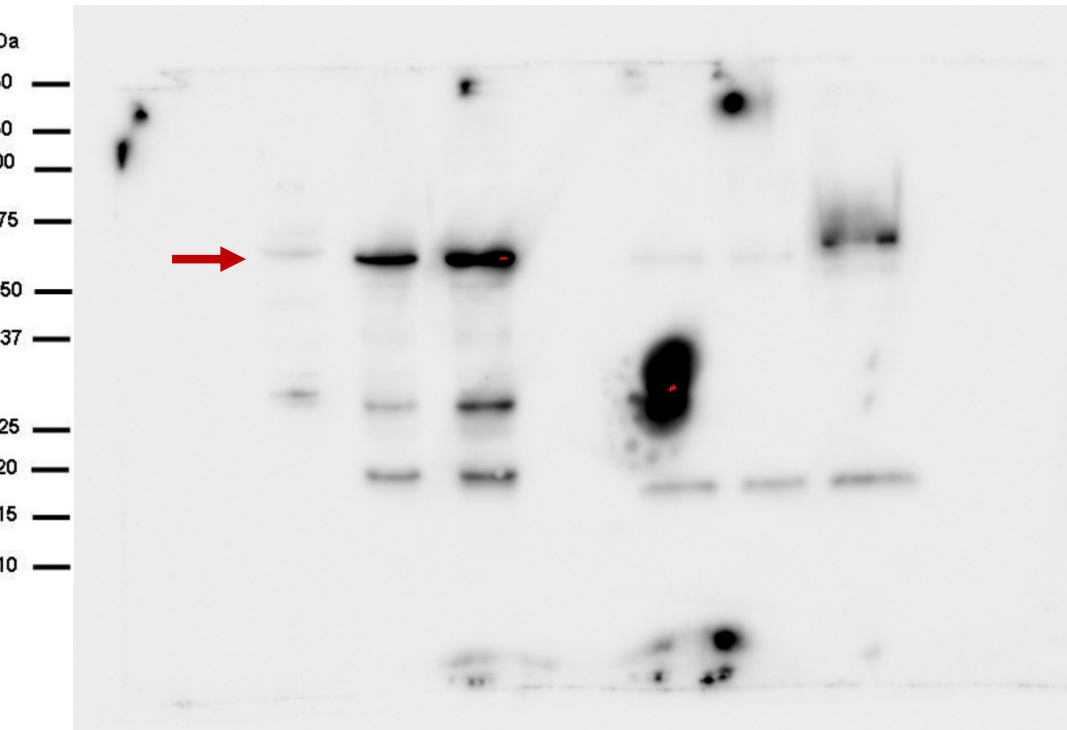
anti-GFP
