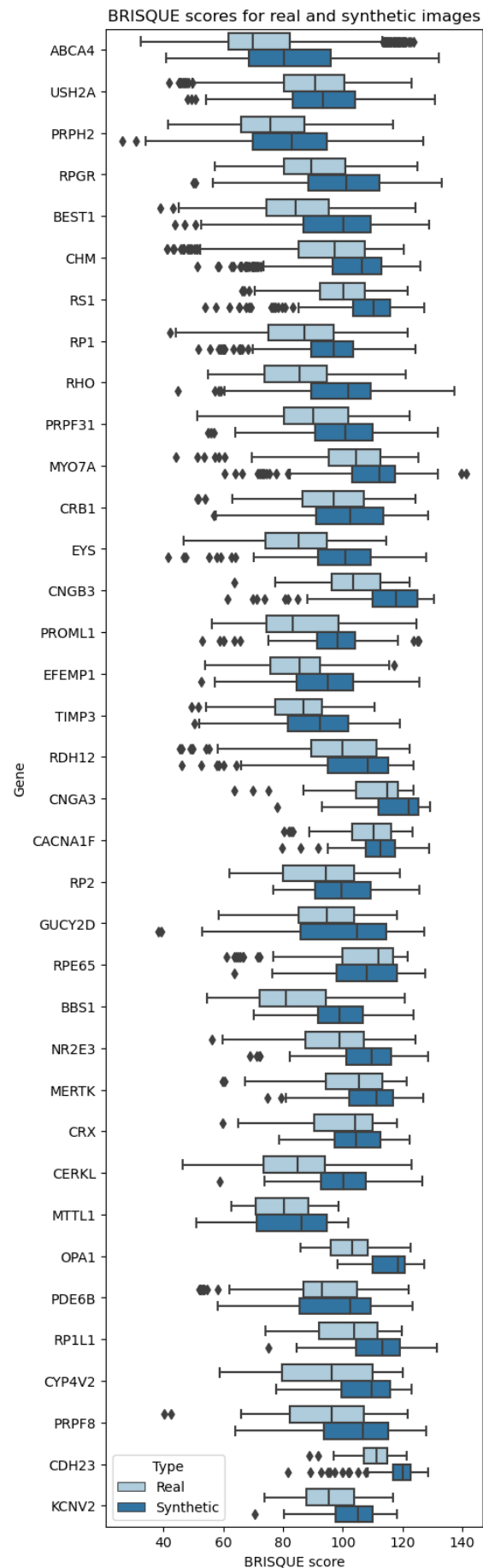
Supplementary Figure 18: Blind Referenceless Image Spatial Quality Estimator (BRISQUE) scores for synthetic and real images of all 36 classes. For all classes, we find a significantly higher ( p < 0.05 ) BRISQUE score for synthetic images relative to real images, suggesting poorer overall image quality.
