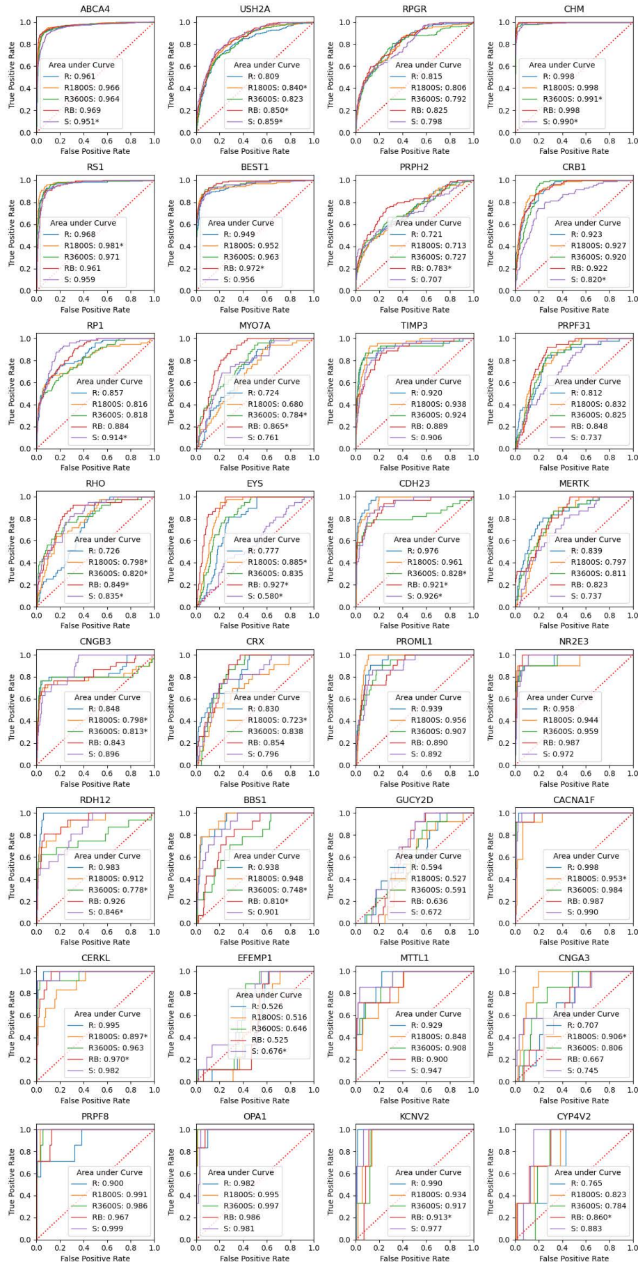
Supplementary Figure 20: Receiver operating characteristic (ROC) curves evaluating the IRD classifier performance per class. The ROC curves in each subplot represent five models from Regime 1 and 1.5, which are defined in Table 1. The figure legend contains the area under the ROC curve which describes the diagnostic ability of the model between 0 (poor classifier) to 1 (optimal classifier). * indicates significant difference between the area under ROC (AUROC) of the model and the baseline R model in that plot ( p < 0.05 , Delong's test).
