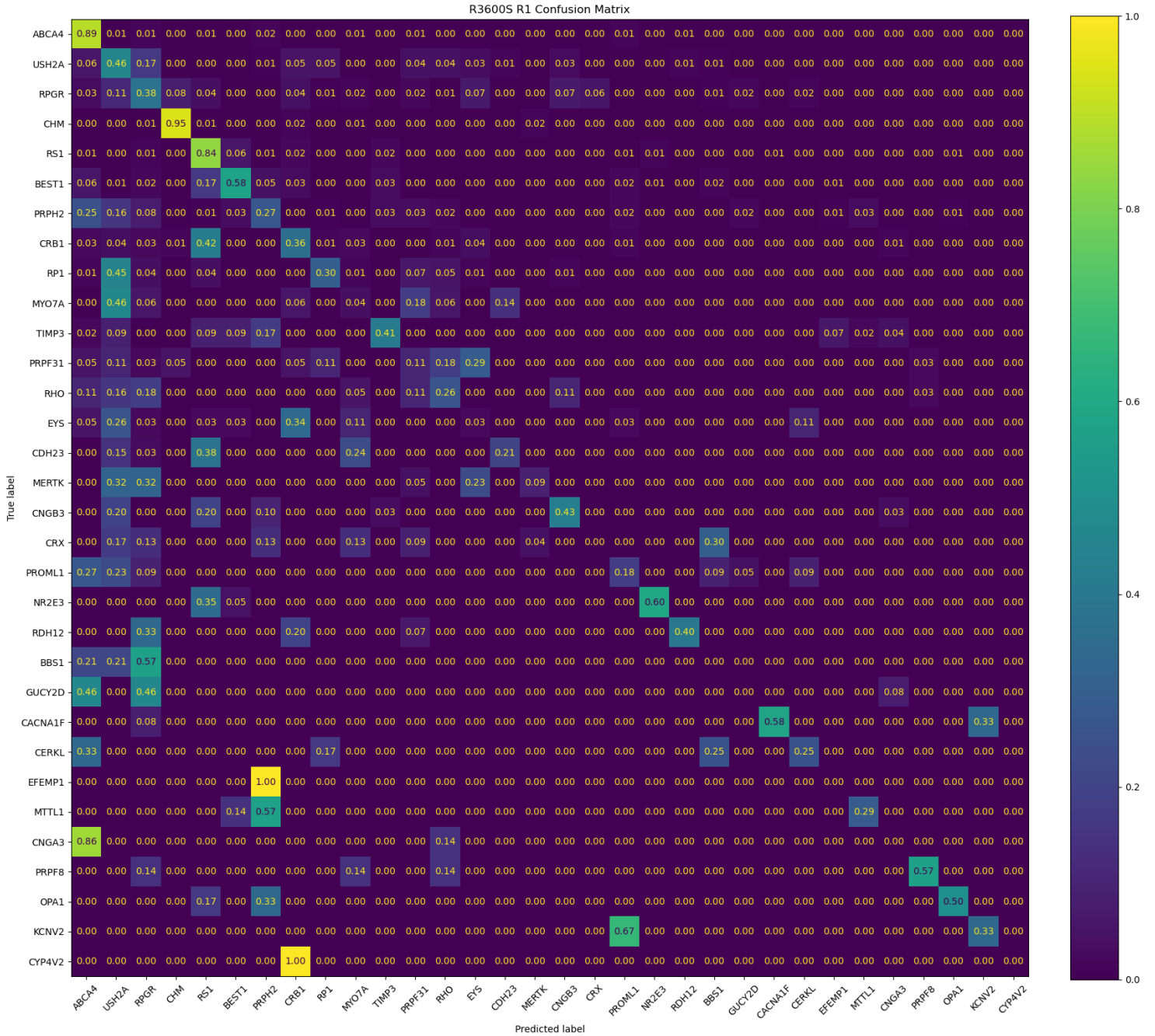
Supplementary Figure 26: Confusion Matrix for the IRD classifier model trained on the entire real IRD training dataset plus 3600 synthetic images (100 images augmented per class) (R3600S – Regime 1). Values are normalized over the true predictions (rows), thus each value represents the proportion of true examples classified by the model as the predict class indicated by the column.
