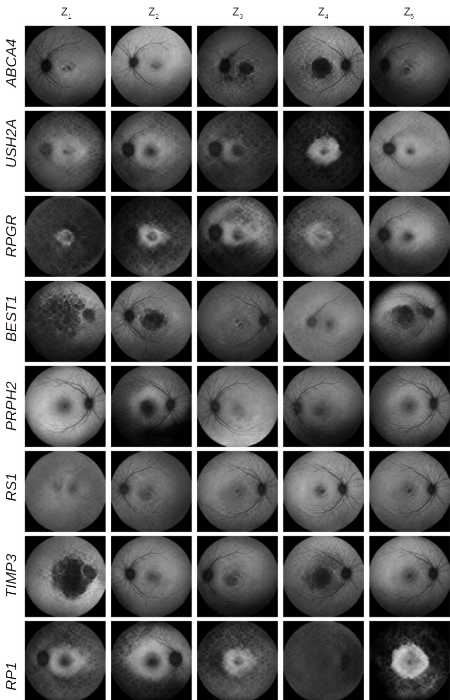
Supplementary Figure 5: Examples of synthetic images created from our initial experiments with multi-scale gradients Generative Adversarial Network (GAN). Rows represent the class and columns represent different noise vectors used to generate the image. While the images were of reasonable quality, the GAN was not able to reproduce the diversity of the training set.
