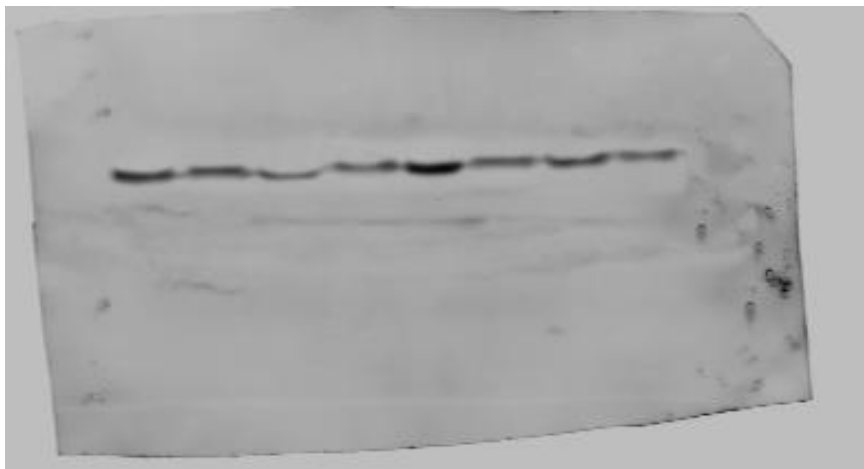
85 kD p-PI3k
