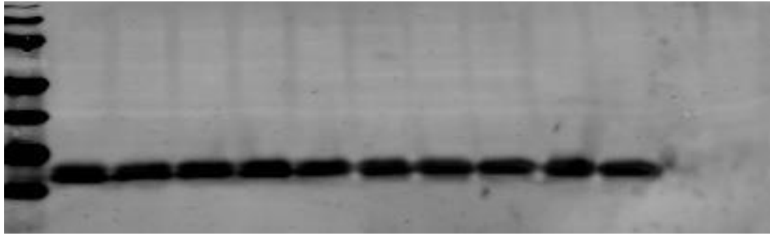
36 kD GAPDH
