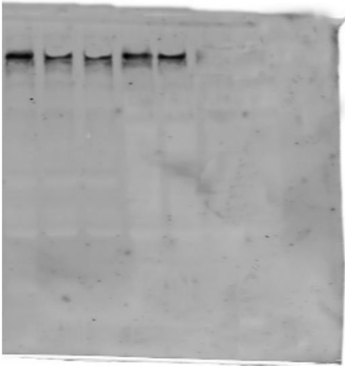
65-80 kD ABCG2
