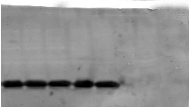
36 kD GAPDH
