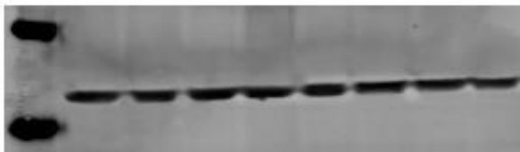
110 kD PI3k
