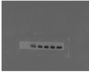
Figure 1A. IGF-1R
