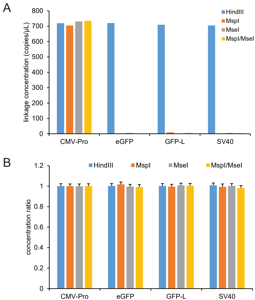
Figure S28. Milepost analysis of pAV-CMV-GFP. The (A) linkage concentration and (B) concentration ratio is shown for a milepost experiment using CMV-Enh FAM and the indicated HEX assay with either HindIII, MspI, MseI, or a double digest with MspI and MseI. The error bars represent the 95% confidence interval.
