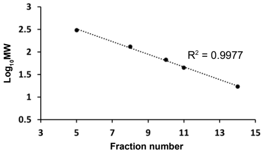
A Regression curve of standard proteins in SEC1
