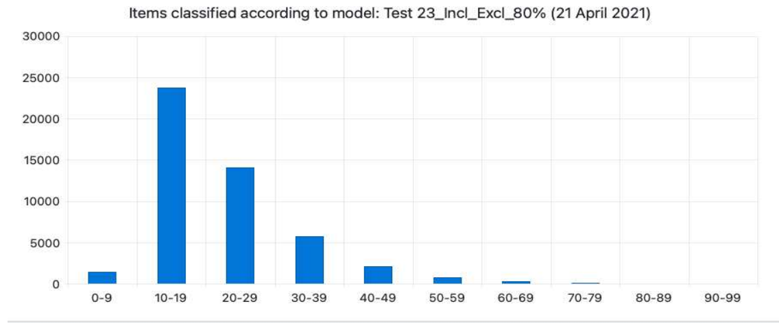
Figure S2: Distribution of all records across 10 classes (decile bands) representing probability of relevance from 0 to 99%, modelled with supervised machine learning (bespoke classifiers)
