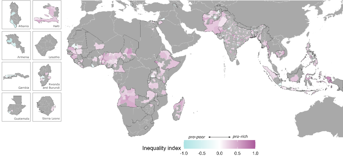
Fig S3. Subnational estimates of Wagstaff's (a) and Erreygers' (b) indices of inequality statistically significant at 95 percent level. Spatial boundaries were retrieved from Natural Earth ( https://www.naturalearthdata.com/ ) using "rnaturalearth" package ( https://github.com/ropenscilabs/rnaturalearth ).
