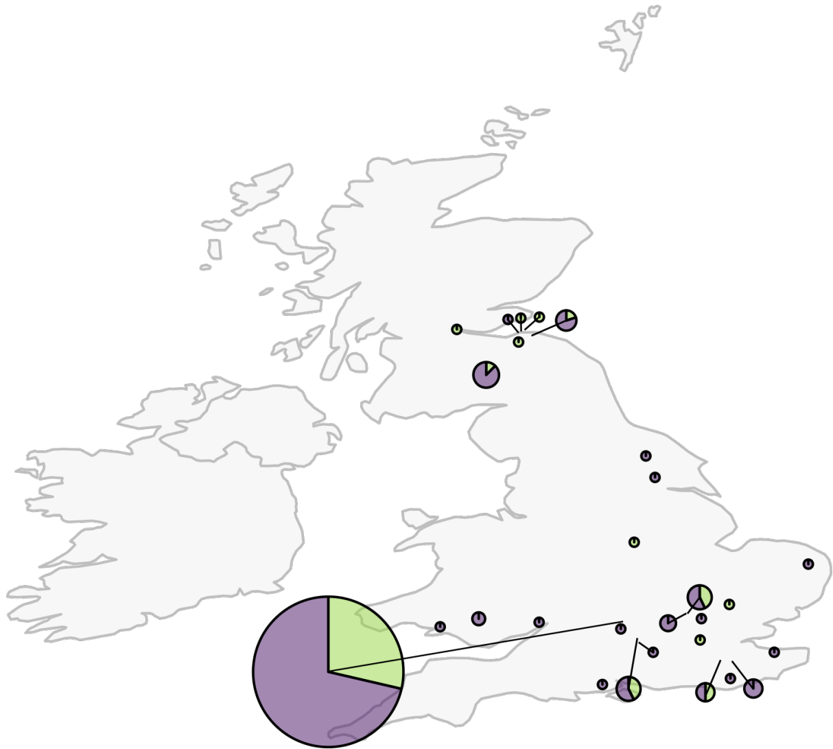
S2 Fig. Sampling locations and incidence of Wolbachia presence (green) and absence (purple) of DTOL samples from Britain and Ireland. The map was drawn using the maps library (version 3.4.0) in R, which imports data from the public domain (Natural Earth project) ( https://www.naturalearthdata.com/downloads/50m-physical-vectors/ ). The size of the pie charts reflects the number of collected samples per location. Most samples came from Wytham Woods Genomic Observatory near Oxford. The data underlying this Figure can be found in S1 Data.
