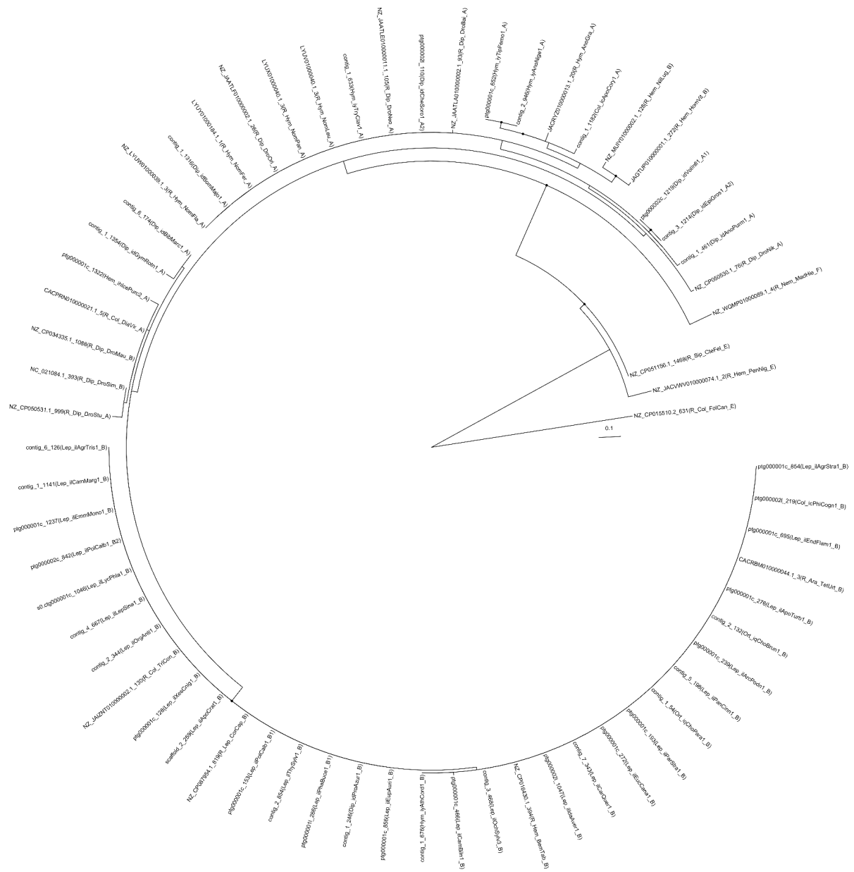
S13 Fig. Phylogeny of ParD toxin genes, highlighting nodes with a bootstrap value higher than 80 with a circle.
