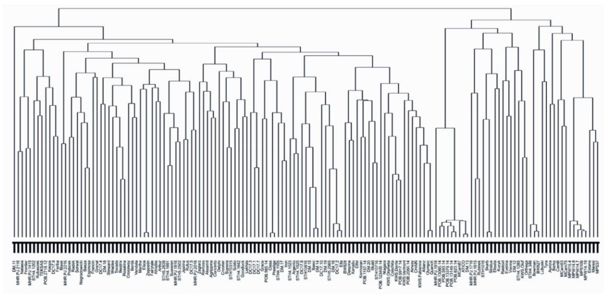
Supplementary Figure 1. Dendrogram of all 149 accessions constructed by hierarchical clustering using the average linkage method based on kinship matrix.
