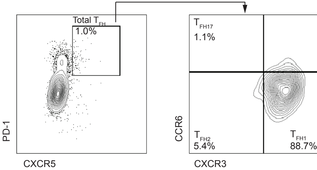
Supplemental Figure 3. Gating strategy for Total T FH and T FH subsets. Parent gate of Total T FH is CD4 T cells.
