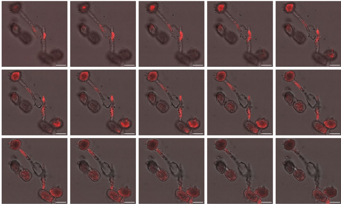
Figure S2 Selected Cy3 dsRNA_1 Z stack confocal images. The complete Z stack consisted of 33 images across a depth of 10.65 \mu\text{m} . Images were taken on a Leica Microsystems SP8 system, scale bars correspond to 20 \mu\text{m} .
