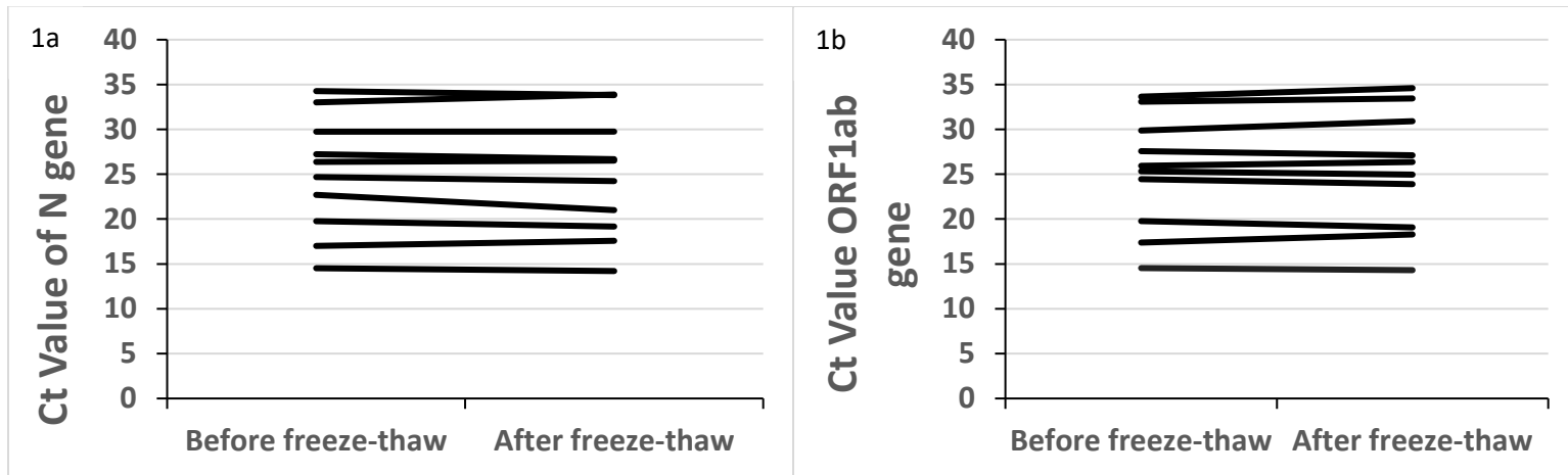
Supplemental Figure 1. Ct values of N gene (1a) and ORF1ab (1b) of 10 COVID-19 positive samples before and after one cycle of freeze-thaw.
