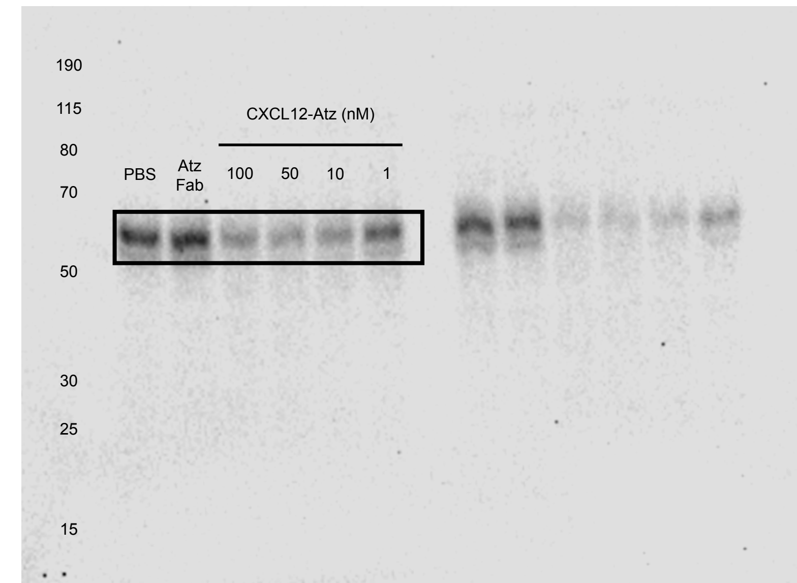
e. Mouse PD-L1 blot
