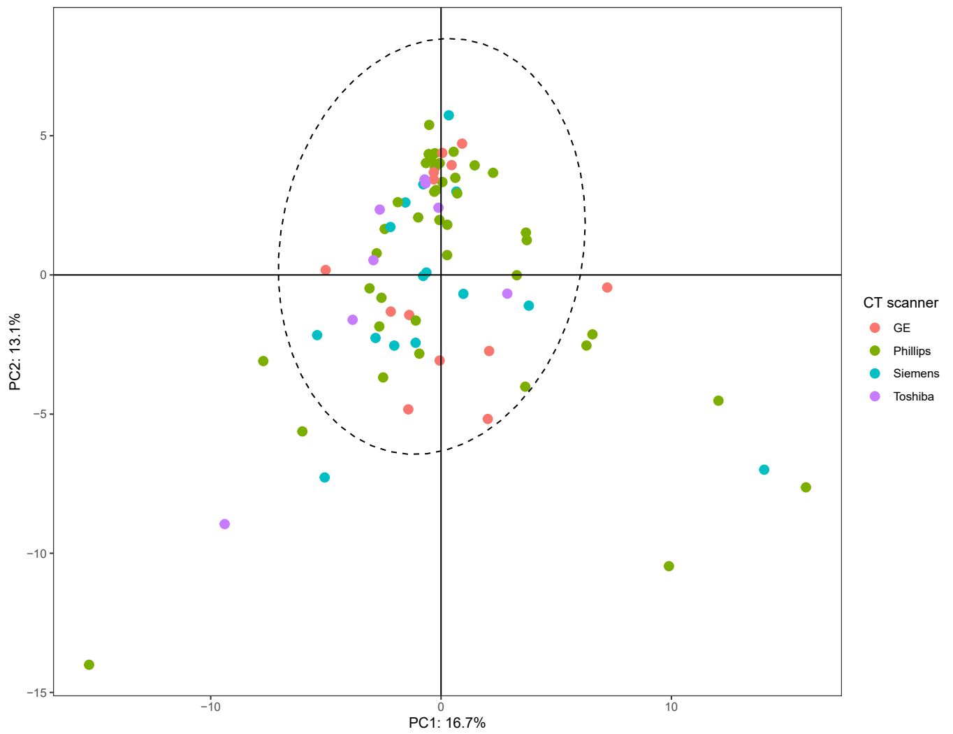
Figure S3. PCA for RCR features.
