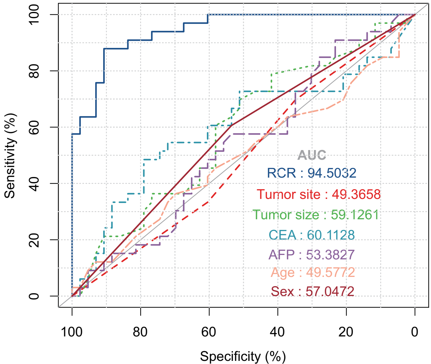
Figure S1. ROC curves for RCR features using scores established by LDA and other clinical predictors.
