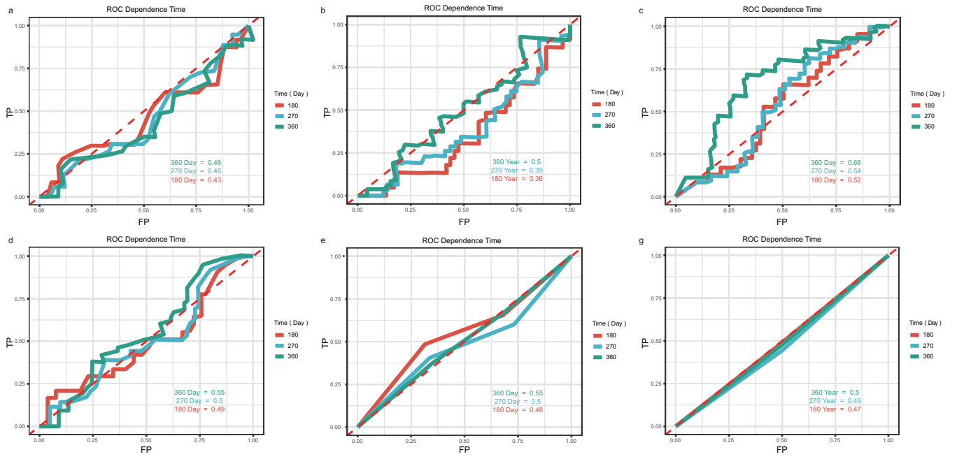
Figure S2. Time-dependent ROC curves for Age (a), AFP (b), CEA (c), Tumor size (d), Tumor site (e) and Sex (g).
