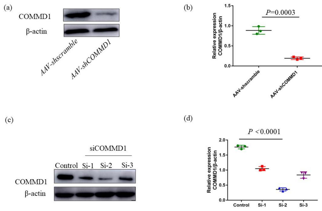
Figure S1. (a-b) The infection efficiency of COMMD1 knockdown. (c-d) siRNA knockdown efficiency for siCOMMD1
