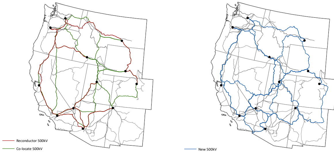
Fig. S8. Least cost path model results showing 500 kV transmission lines. Left: recondored and co-located 500 kV lines only. Right: new 500 kV lines only. )
