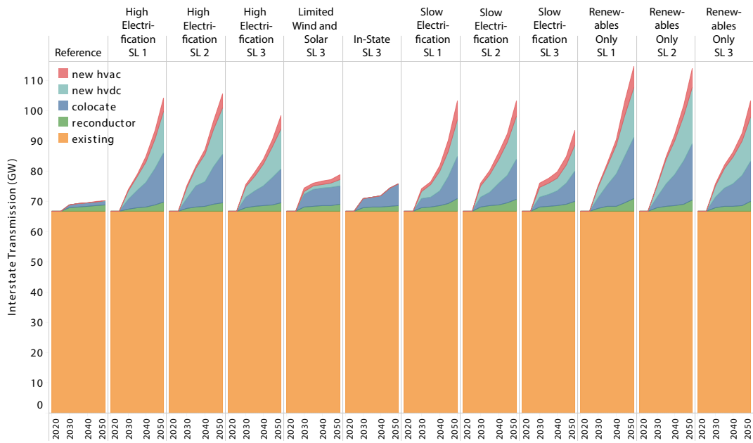
Fig. S22. Existing and new transmission capacity for the reference scenario and all decarbonization scenarios.
