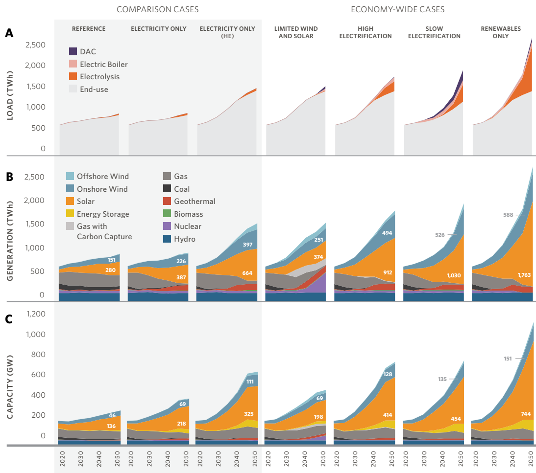
Fig. S14. Electricity demand (Load) (A), generation (B), and installed capacity (C) across the western U.S. for scenarios that achieve different decarbonization targets (reference, electricity only, and economy-wide net zero cases) or with different decarbonization pathways (High Electrification, Slow Electrification, Renewables Only). This figure is the same as Figure 2 in the main paper, except that it includes the sensitivity energy cases, In-State, Limited Biomass, the Limited Wind and Solar. See Figure 2 for the complete caption.
