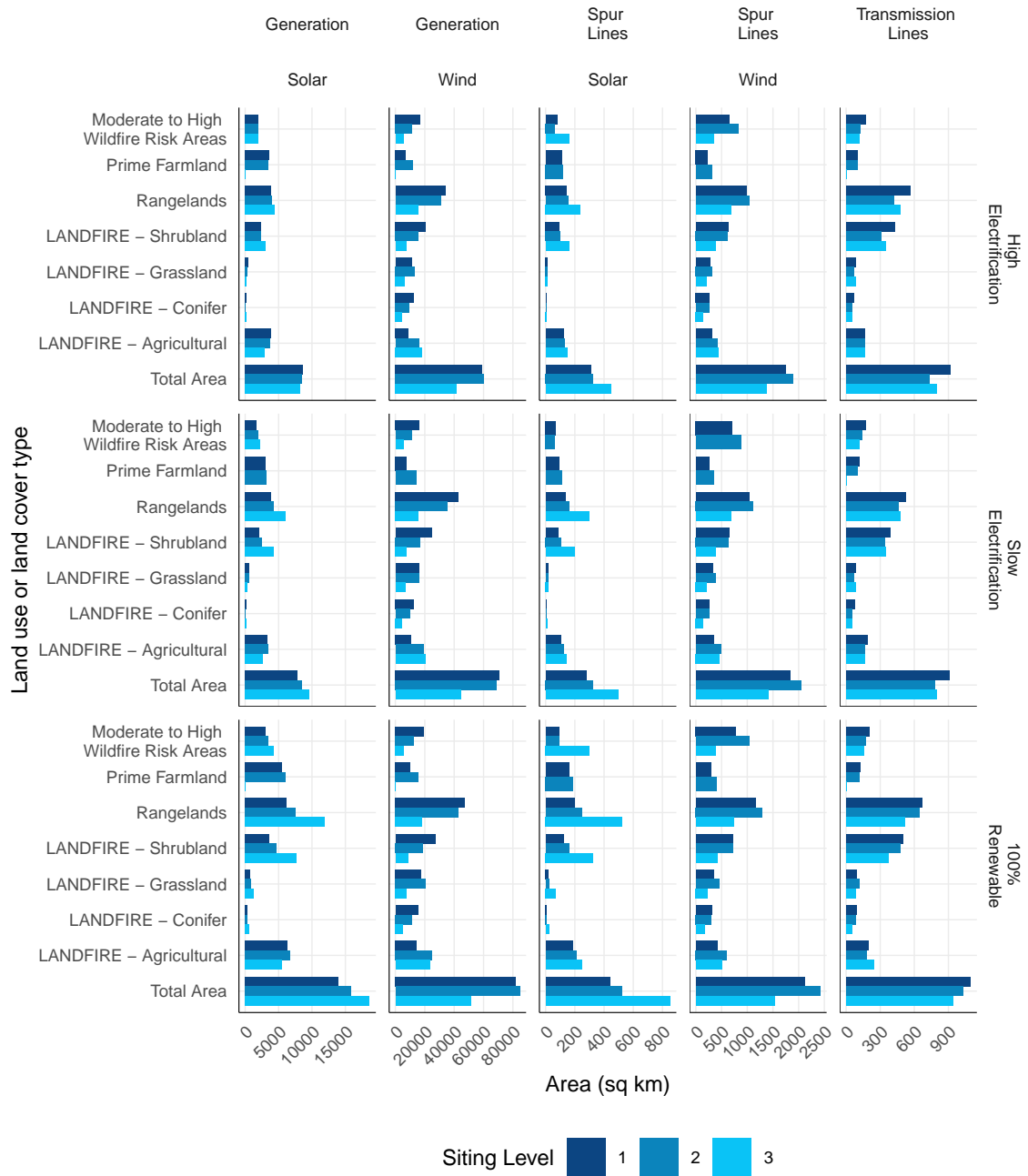
Fig. S27. Land use and land cover impacts for generation, transmission, and spur lines for the three core economy-wide cases at all Siting Levels.
