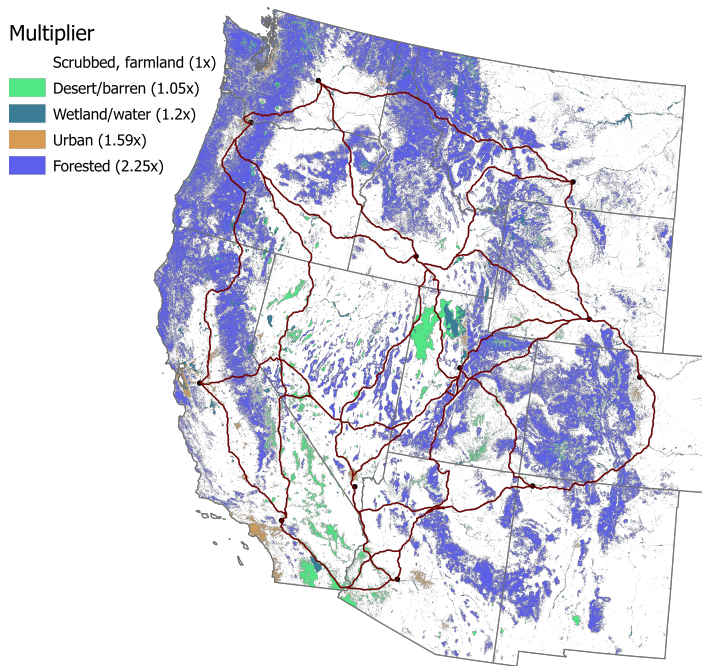
Fig. S7. Least cost path model results showing selected cost surface multipliers and new 500 kV transmission lines.
