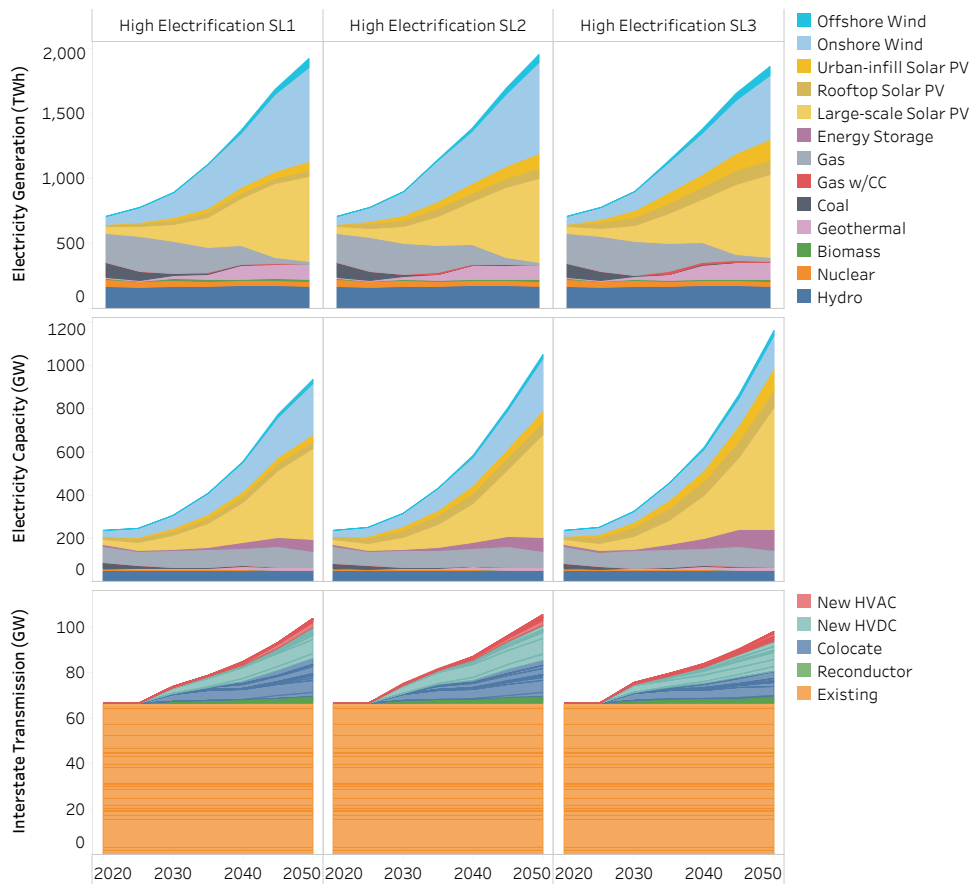
Fig. S21. Generation, capacity, and transmission for High Electrification Siting Levels 1-3.
