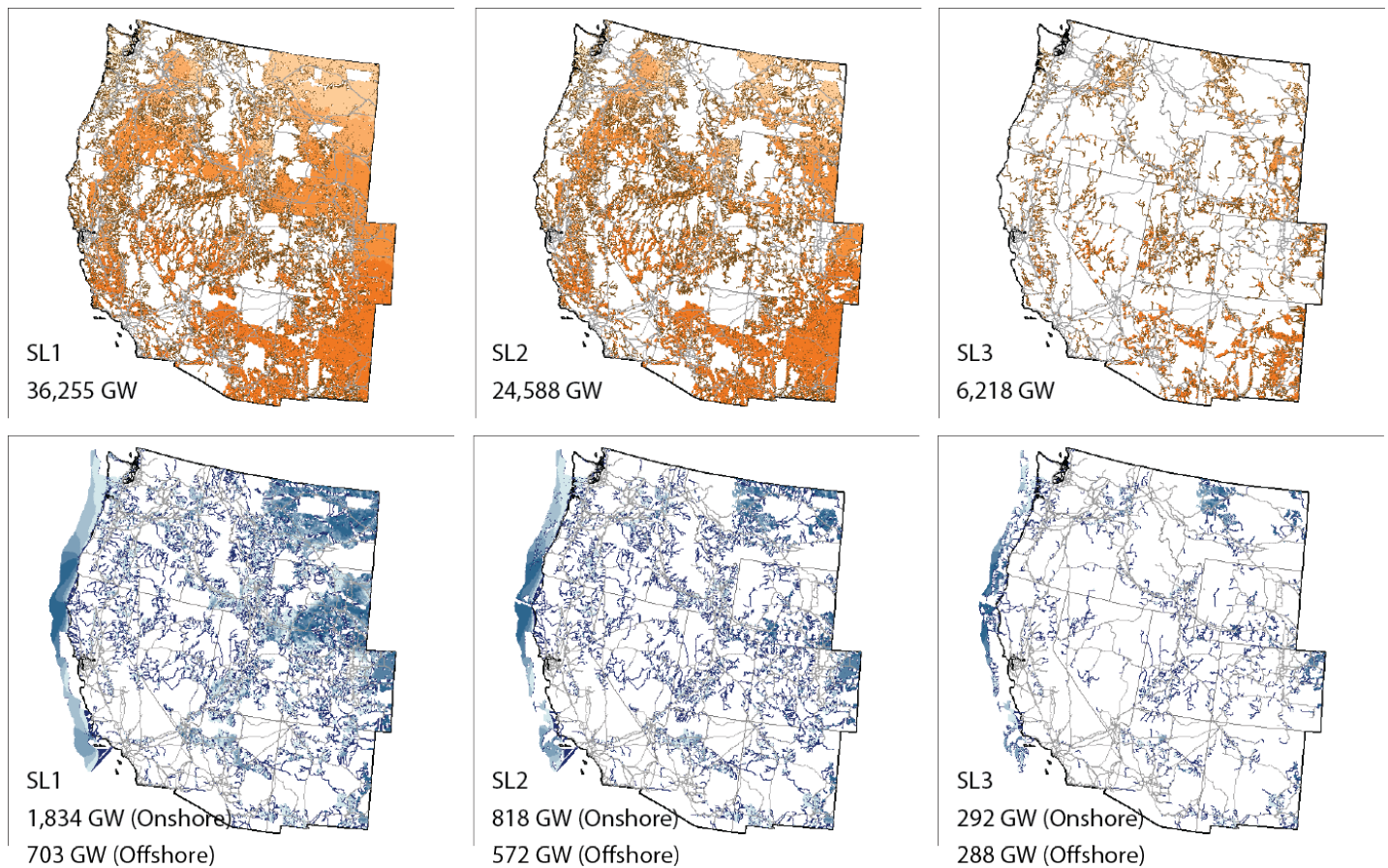
Fig. S3. Utility-scale Wind and solar Candidate Project Areas and spur lines
