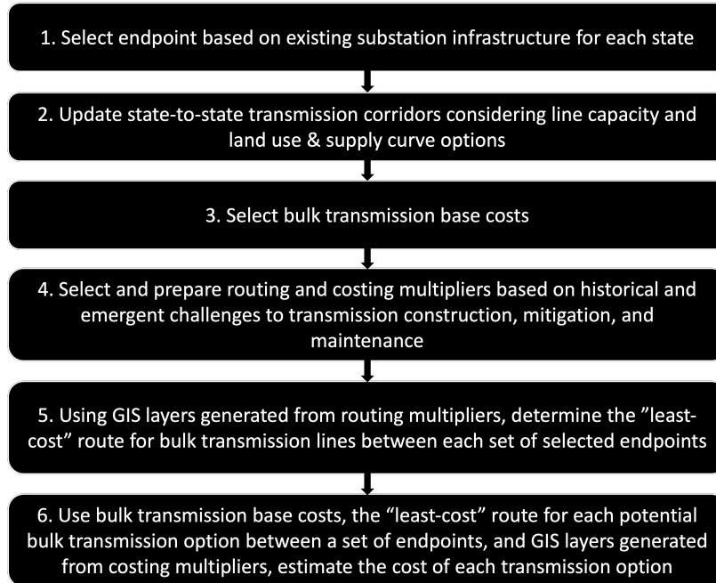
Fig. S5. Transmission modelling flow
