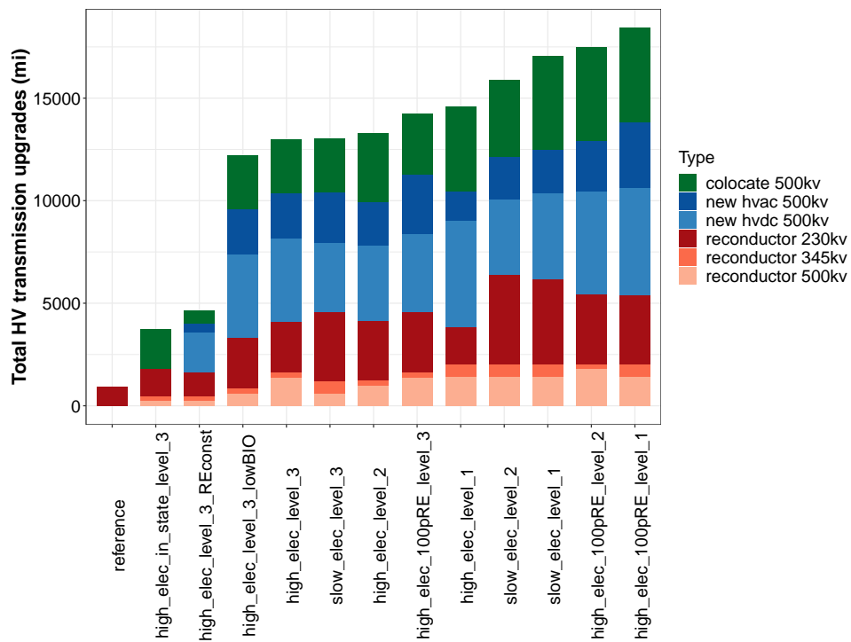
Fig. S25. Spatial downscaling results showing total transmission upgrades in each scenario
