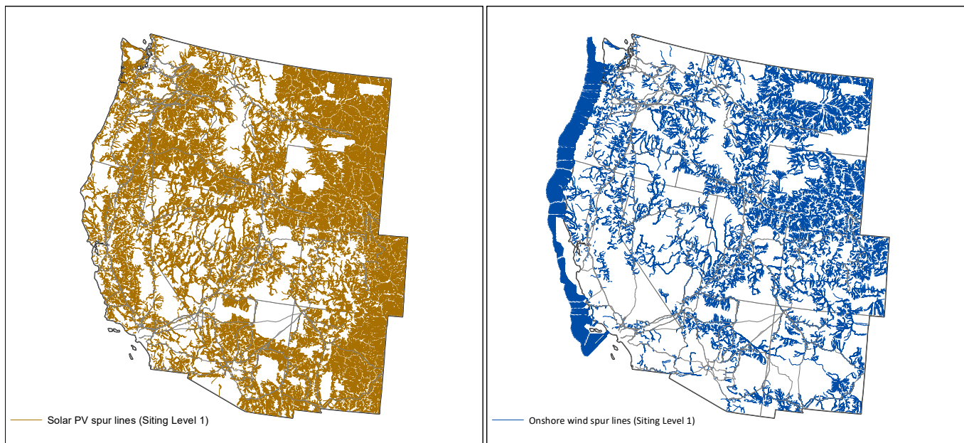
Fig. S11. Least cost path model results showing wind and solar interconnection spur lines. )
