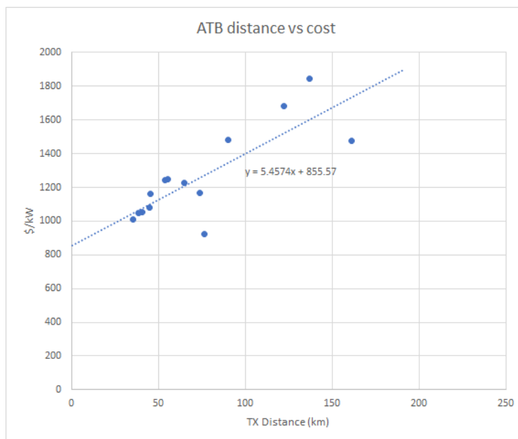
Fig. S10. Linear regression on plot of the ATB2020’s offshore wind transmission costs per kW against the ATB2020’s corresponding average transmission distance
