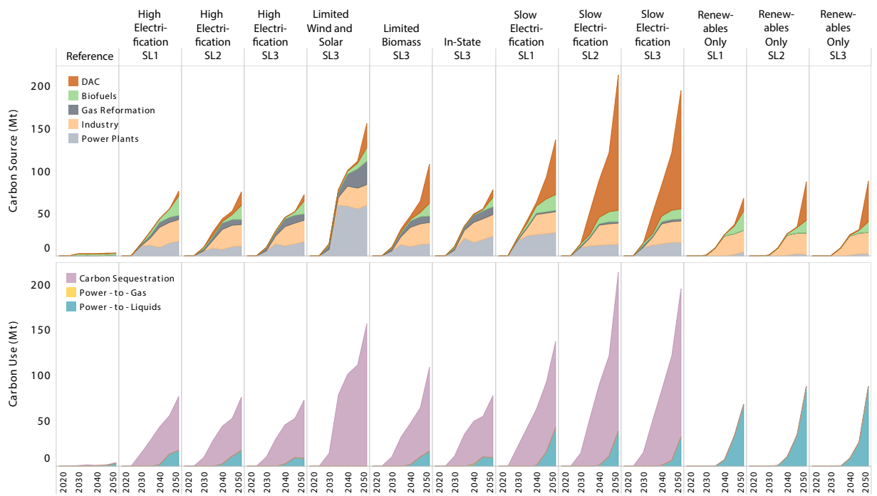
Fig. S17. Carbon emissions, storage, and use
