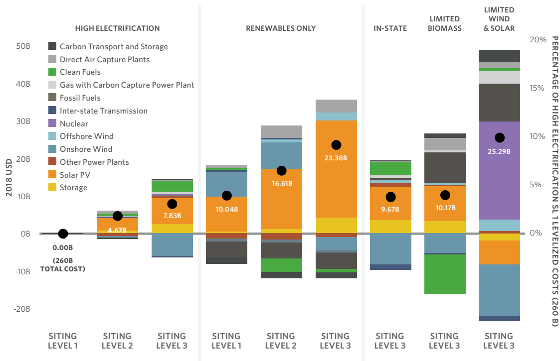
Fig. S15. Net annual levelized supply-side cost in 2050 for scenarios are shown relative to the High Electrification Siting Level 1 scenario. Bars above the x-axis represent and increase in costs while bars below represent a decrease in relative cost. This figure is the same as Figure 4 in the main paper, except that it includes the sensitivity energy cases, In-State, Limited Biomass, the Limited Wind and Solar. See Figure 4 for the complete caption.
