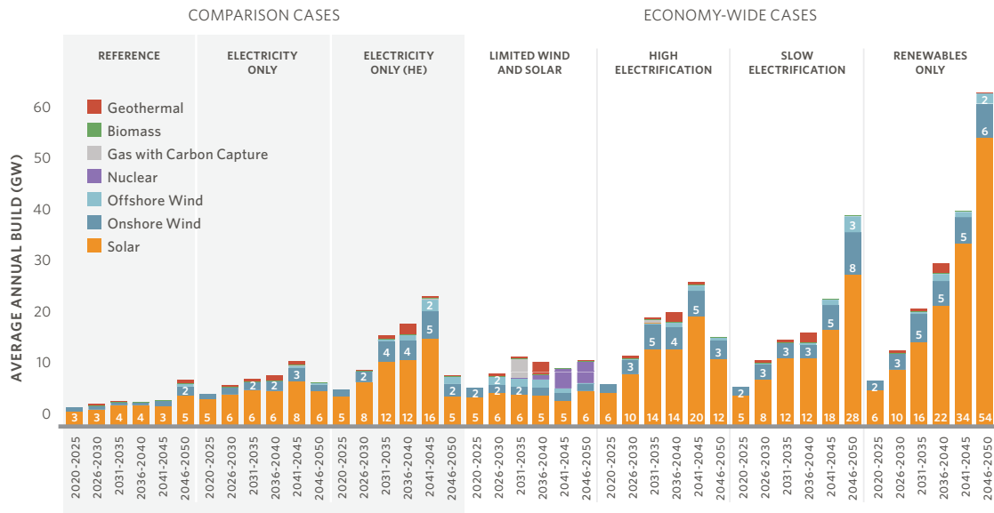
Fig. S16. Average annual generation capacity build rates by 5-year period for the reference case contrasted against different decarbonization cases using Siting Level 3 (SL3) protections
