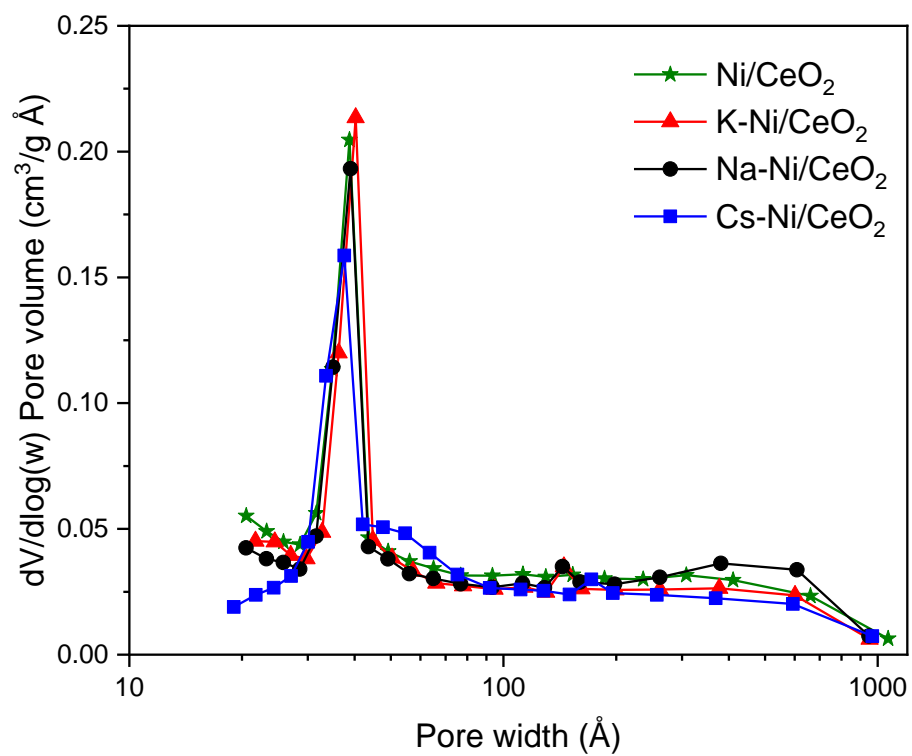
Figure S1. Pore size distribution of the catalyst calculated on the desorption branch using the BJH model.
