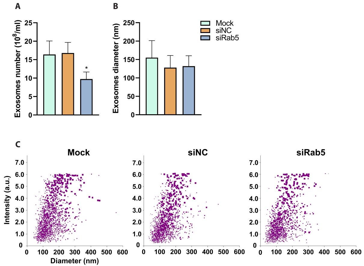
Supplementary Fig. 1. The characteristics of the exosomes isolated from MDA-MB-231 cells. The number (A) and diameter (B), and size distribution (C) of exosomes isolated from MDA-MB-231 cells without transfection or with transfection with siNC and siRab5; n = 3 . Data was represented as mean \pm SD. * p < 0.05 .
