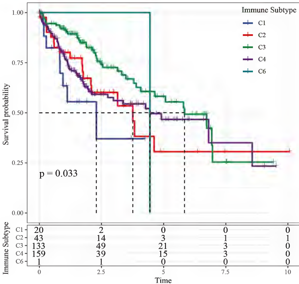
S7_Fig.1. There were significant differences in the pancancer immunotypes
