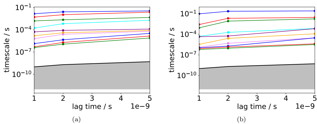
Figure S1: Plot of first 10 implied timescales for unbiased state versus MSM lag time for TRAM models constructed using (a) 50 clusters and (b) 100 clusters.
