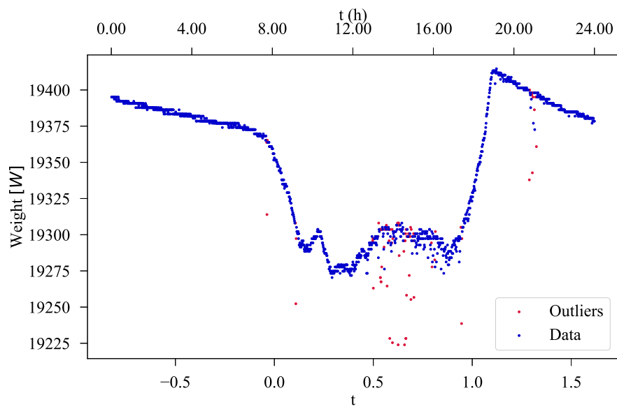
S 2 Fig. Example of outlier detection for the Hive 10 on 2018-4-7. The outliers detected are in red color and were removed before the data analysis.
