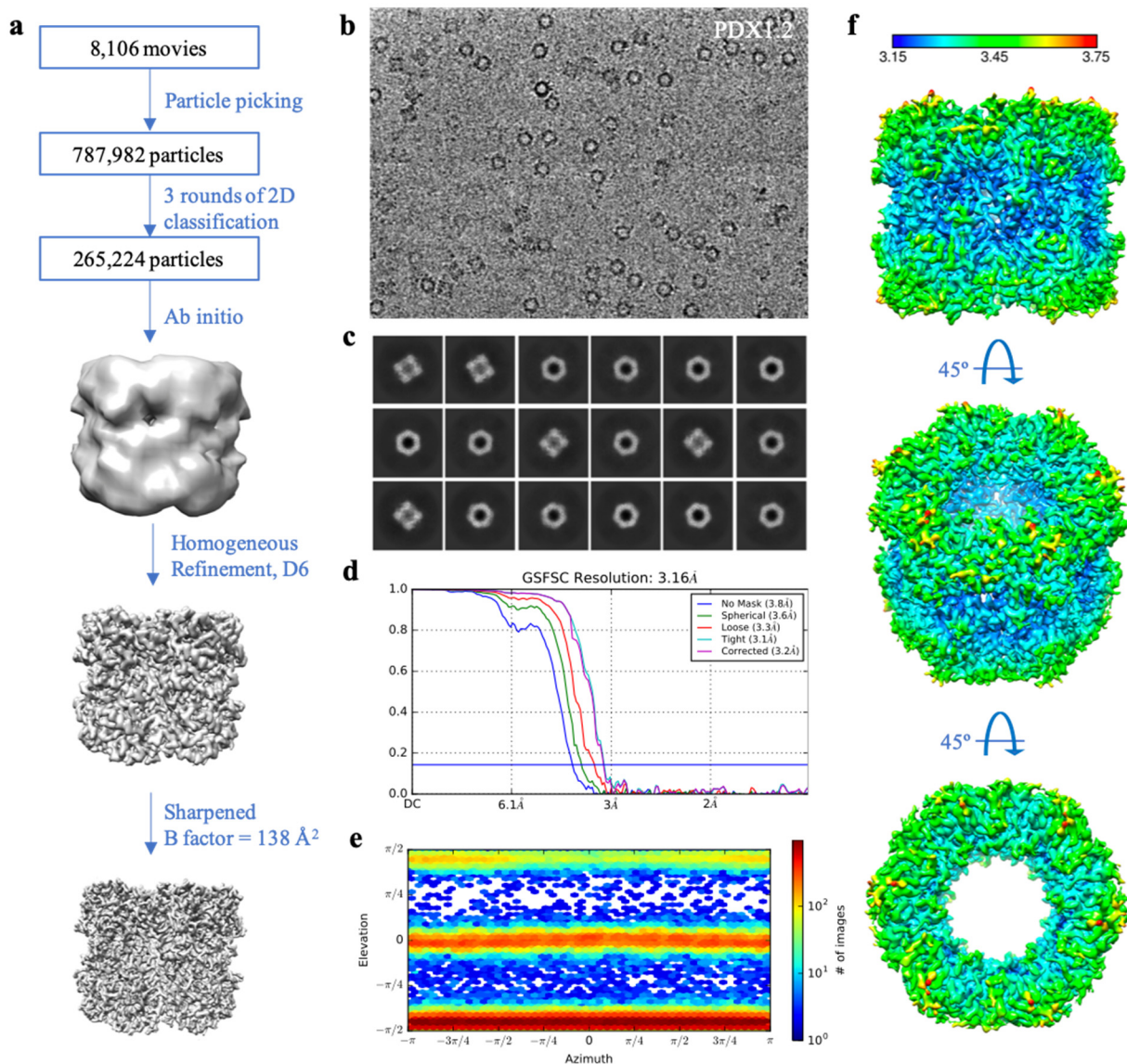
Supplementary Figure 9. Cryo-EM single particle analysis workflow for PDX1.2 homocomplex. a) All processing was performed in cryoSPARC v2. Movies were first corrected for beam motion, and CTF parameters were determined. The positions of particles were identified using a template-based autopicking algorithm and corrected for local motion. The final pool of 787,982 particles was subjected to three rounds of reference-free 2D classification (with 150 classes each round). The curated pool of 265,224 particles was then used for ab initio model generation, which was further used for homogenous refinement. The final structure shows a 3.2 Å resolution. b) A representative image of the PDX1.2 complexes in vitreous ice. c) Representative 2D classes. d) The Fourier shell correlation (FSC) curve and (e) Euler angle distribution of refined map. f) PDX1.2 reconstructed map sharpened and colored according to local resolution in Angstroms.
