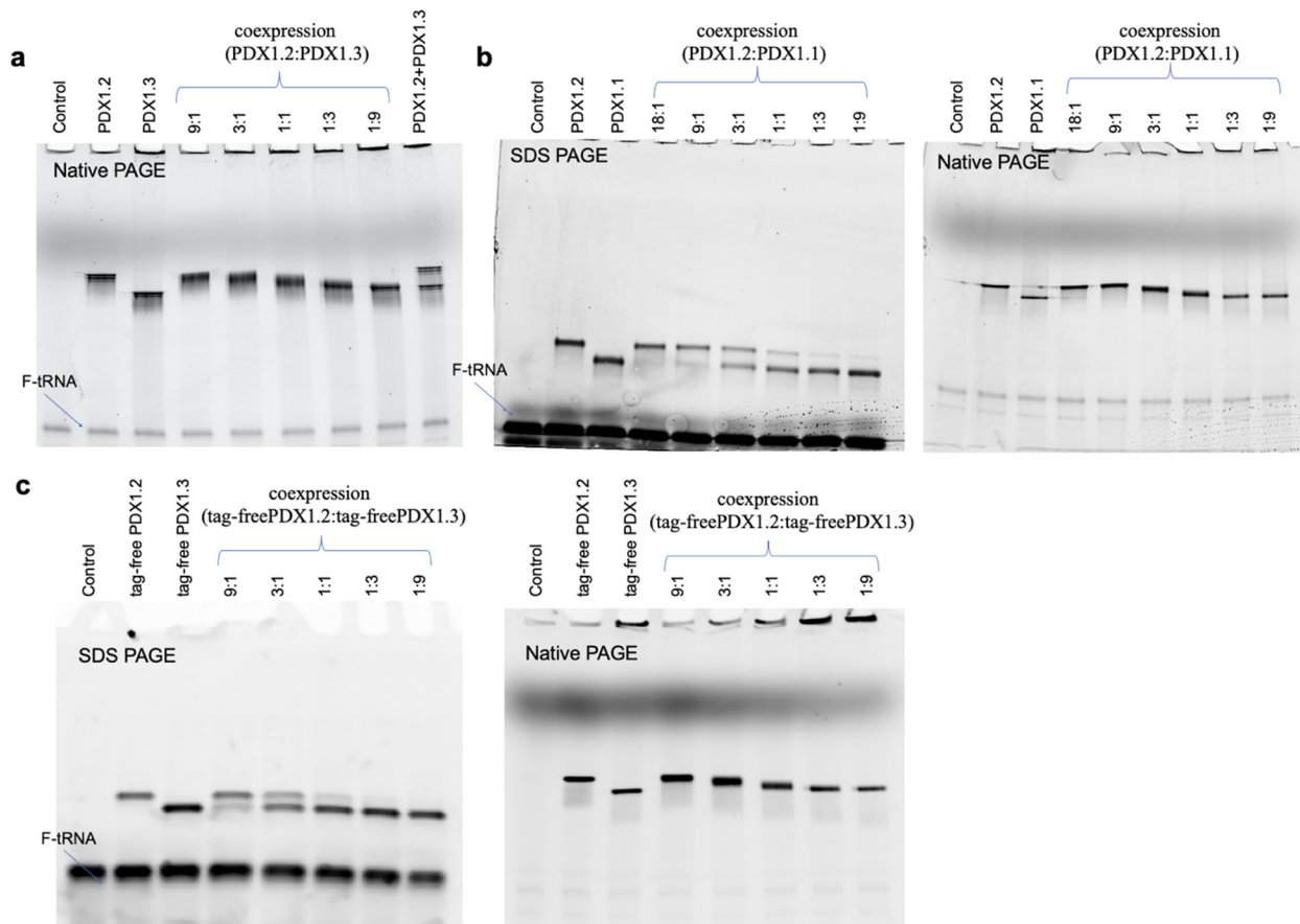
Supplementary Figure 2. Additional gel electrophoresis data for PDX1.2—PDX1.3 and PDX1.2—PDX1.1 pseudoenzyme—enzyme complexes. The fluorescent bands were detected by Typhoon FLA 9500 from GE Healthcare, set for Alexa488 dye excitation and emission settings. a) Native PAGE conducted on the same samples as in Figure 1, panel c but after 48 hours incubation at 4°C. No observable degradation of complexes was detected compared to Figure 1. The last lane shows the individually expressed homomeric PDX1.2 and PDX1.3 proteins mixed post-translationally and incubated for 48 hours. The PDX1.2 and PDX1.3 remained homomeric in the mixture and no formation of intermixed complexes were observed as shown by distinct bands matching to the two individual proteins. b) PAGE data on the coexpression of PDX1.2 and PDX1.1 proteins in the crude wheat germ mixture. Coexpressed conditions are denoted as 18:1, 9:1, 3:1, 1:1, 1:3 and 1:9, where these numbers correspond to DNA template ratio of PDX1.2 to PDX1.1. PAGE data include a denaturing SDS-PAGE gel on the left and Native PAGE on the right. F-tRNA stands for fluorophore-labeled lysine-charged tRNA. Note that a similar trend in complexation is seen for PDX1.2-PDX1.3 pair, as shown in panel (a) and Figure 1, panel c. c) PAGE data on the coexpression of tag-free PDX1.2 and PDX1.3 proteins. Their assembly and mobility behavior on the gels appear identical to the tagged PDX1.2 and PDX1.3 proteins (Figure 1, panel c).
