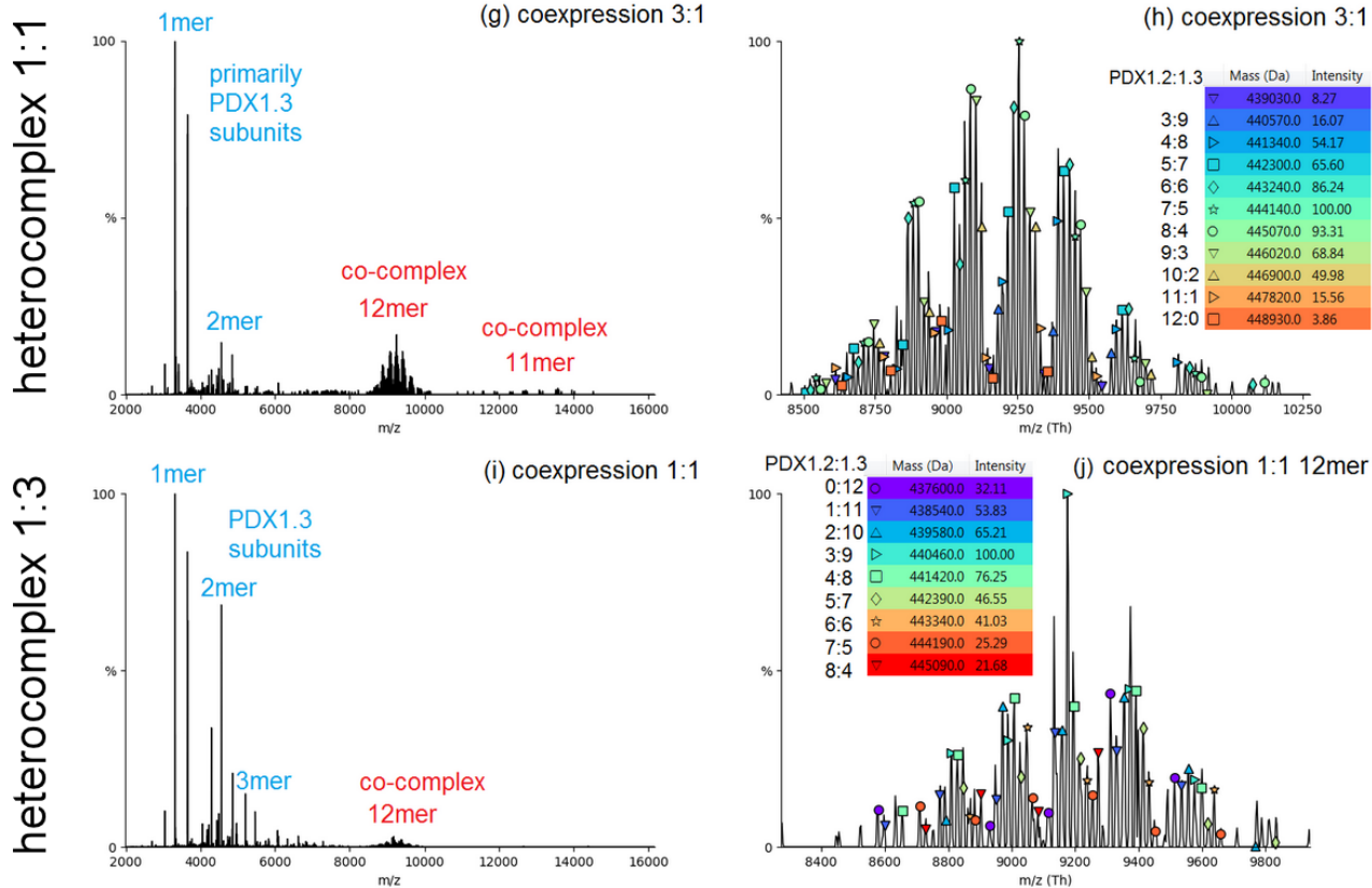
Supplementary Figure 7. (a, c, e, g, i) Full range and (b, d, f, h, j) zoomed native mass spectra of PDX1.2, PDX1.3 and heterocomplexes 3:1, 1:1 and 1:3. Spectra were generated using UniDec ( https://github.com/michaelmarty/UniDec ).
