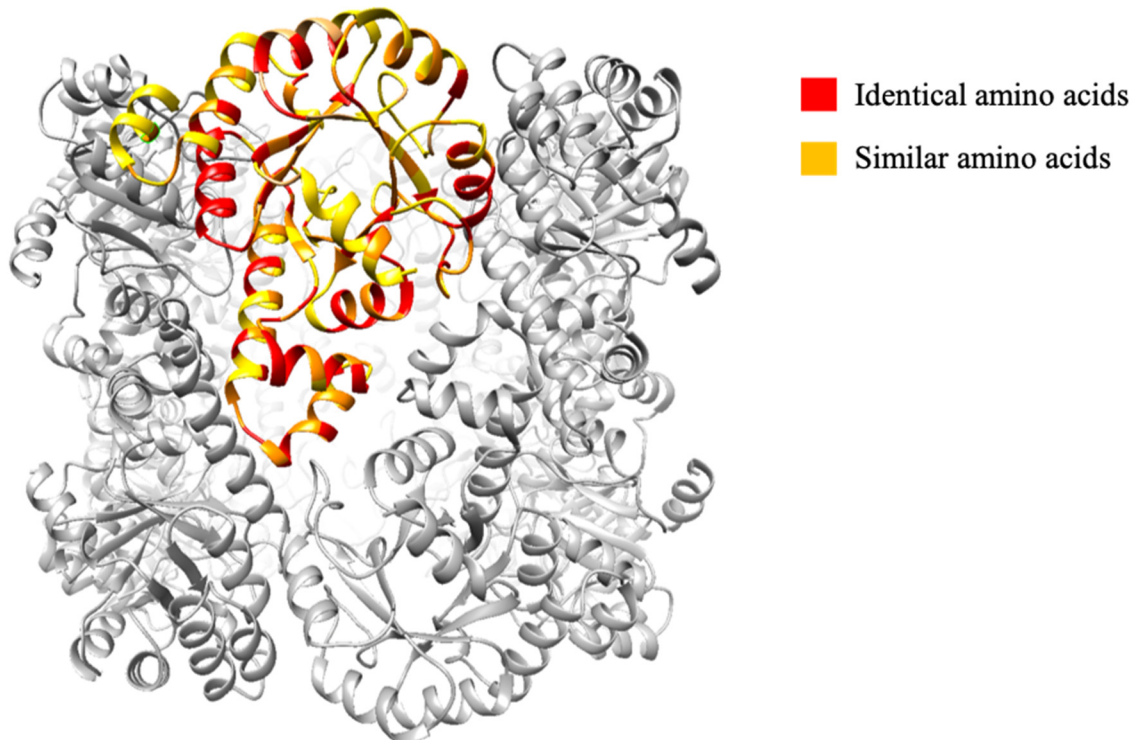
Supplementary Figure 17. Alignment of PDX1.2 sequences across plants and mapping of conserved amino acids within the PDX1.2 pseudoenzyme family. The UniProtKB database was searched for proteins under the name of “pyridoxal 5'-phosphate synthase-like subunit”. Sequences were retrieved and aligned using Clustal Omega. The most conserved residues (in red and orange) were mapped on the cryo-EM structure of PDX1.2 monomer. The amino acids residues in yellow are the least conserved.
