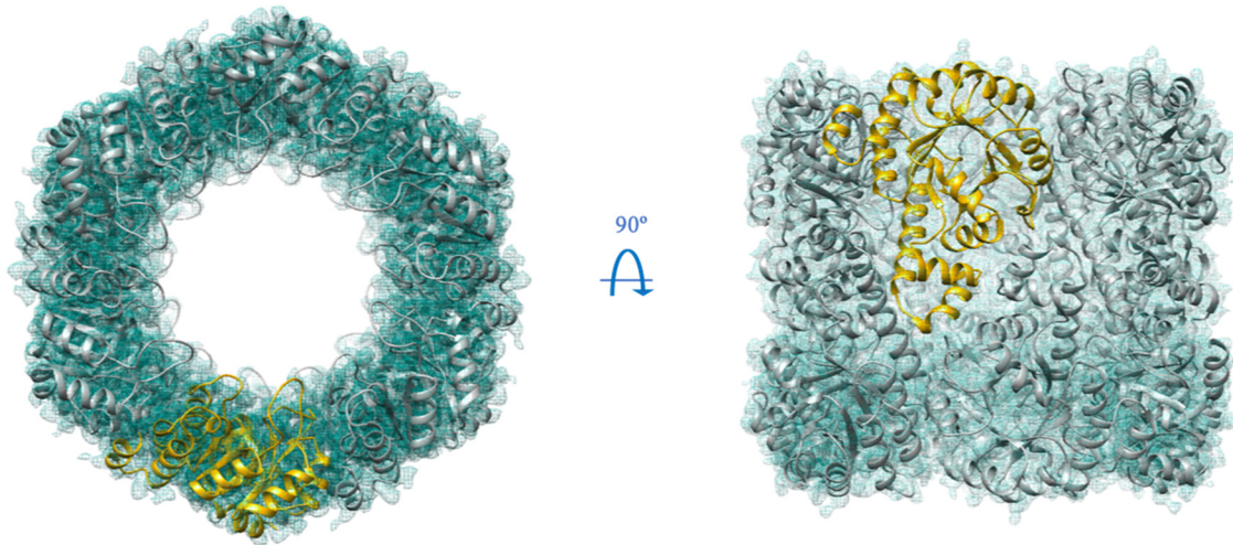
Supplementary Figure 10. Atomic model of PDX1.2 dodecamer fitted in the sharpened cryo-EM map (green mesh). An asymmetric unit (representing a single PDX1.2 subunit) is shown in yellow.
