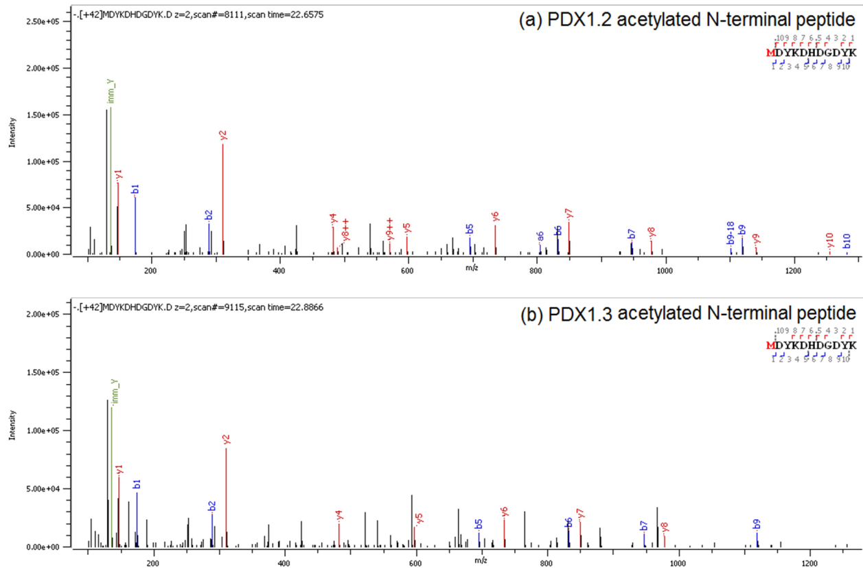
Supplementary Figure 6. Annotated MS 2 spectra of acetylated N-terminal peptide for (a) PDX1.2 and (b) PDX1.3. Fragmentation spectra suggest that acetylations are localized at the N termini of the proteins. In the previous study (Mocand, C. et al. The pseudoenzyme PDX1.2 boosts vitamin B6 biosynthesis under heat and oxidative stress in Arabidopsis . J Biol Chem 289, 8203-8216, doi: 10.1074/jbc.M113.540526 (2014)), E. coli expressed PDX1.2 was found to carry an acetyl group on the alanine (A5). Such modification was not detected in the wheat germ cell-free produced PDX1.2 and PDX1.3 shown here. N-terminal acetyl groups were detected and located on the first methionine residue, preceding the exogenous protein tag.
