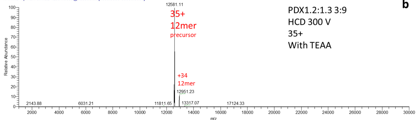
Supplementary Figure 14. HCD spectra of a select 12mer with the stoichiometry of 3:9 (PDX1.2:PDX1.3) (a) without and (b) with TEAA. Without TEAA, the 12mer dissociated into 1mer+11mer, which is the typical 1mer stripping behavior for gas phase protein dissociation upon neutral gas collision. Such behavior is generally believed to be correlated with charge directed protein unfolding in the gas phase. With TEAA, protein unfolding can be suppressed, but dissociation was also remarkably suppressed as shown by (b). Even at the maximum collision voltage of 300 V, HCD was not able to generate significant amounts of product for charge reduced 12mer. In contrast, SID was able to yield 6mers for the charge reduced 12mer as shown in Fig. S13.
