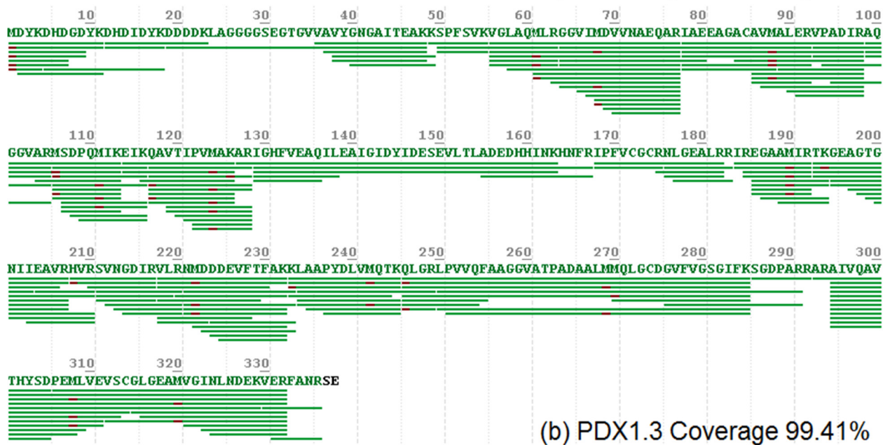
Supplementary Figure 4. Peptide mapping coverage map for cell-free expressed (a) PDX1.2 and (b) PDX1.3. Green horizontal lines along the protein sequences show the peptides detected. Protein residues colored in black are the regions where no peptides were detected (too short to be detected). Red segments along the sequences are modified residues (primarily methionine oxidation and protein N-terminal oxidation), induced by the sample preparation.
