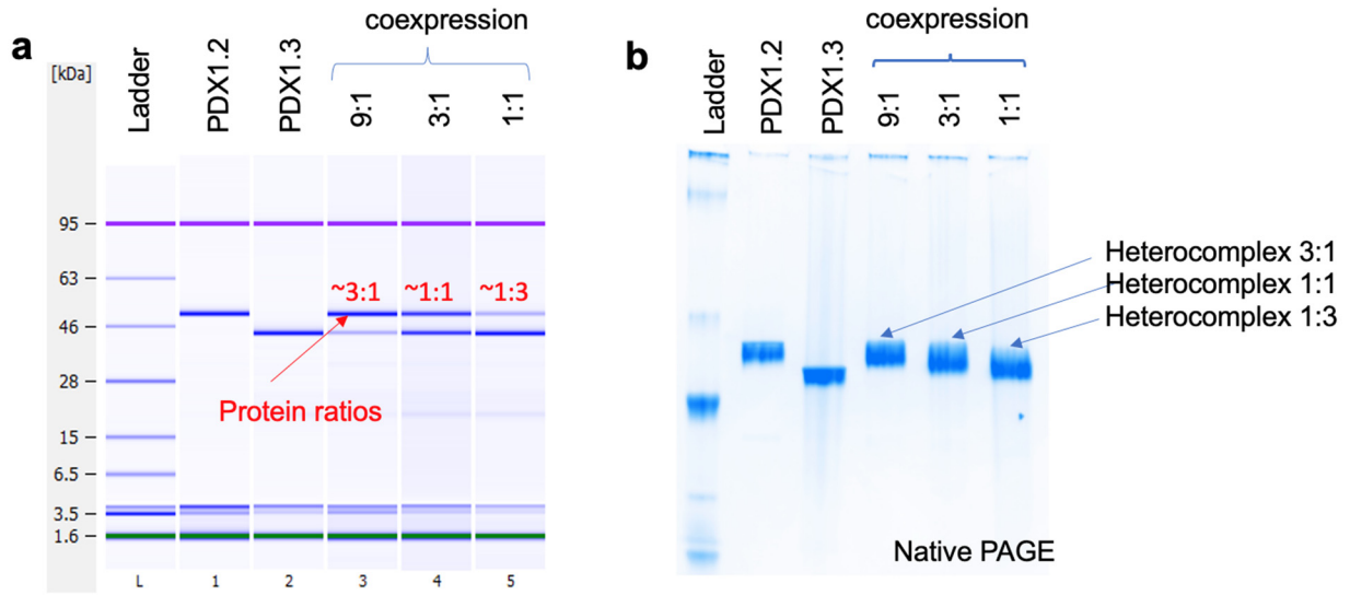
Supplementary Figure 3. Analysis of purified PDX complexes. a) Denaturing Bioanalyzer Protein 80 electropherogram of purified PDX protein samples. b) Native PAGE, stained with Bio-Safe Coomassie Stain. Ladder stands for NativeMark Protein Standard (ThermoFisher). Note that coexpressed samples have wider bands, consistent with Figure1, panel c.
