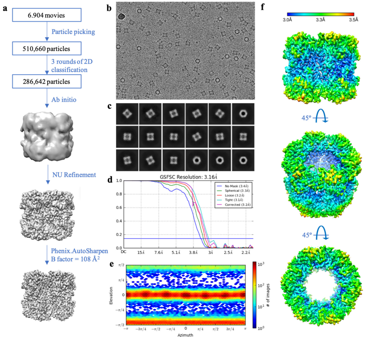
Supplementary Figure 11. Cryo-EM single particle analysis workflow for heterocomplex 3:1. a) All processing (except the sharpening) was performed in cryoSPARC v2. Movies were first corrected for beam motion, and CTF parameters were determined. The positions of particles were identified using a template-based autopicking algorithm and corrected for local motion. The final pool of 510,660 particles was subjected to three rounds of reference-free 2D classification (with 150 classes each round). The curated pool of 286,642 particles was then used in the ab initio procedure to generate an initial model, which was used for global Non-Uniform alignment. The refined structure was resolved to a 3.2 Å resolution. The sharpening of the final volume was done in PHENIX. b) A representative image of heterocomplex 3:1 in vitreous ice. c) Representative 2D classes. d) The Fourier shell correlation (FSC) curve and e) Euler angle distribution of refined map. f) Reconstructed map sharpened and colored according to local resolution in Angstroms.
