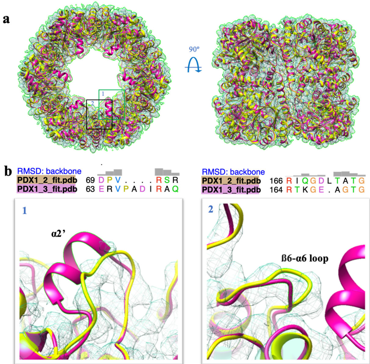
Supplementary Figure 12. Atomic modeling of PDX1.2 and PDX1.3 amino acid sequences into the cryo-EM 3D map for hetero-complex 3:1. a ) Overall dodecameric fits of PDX1.2 (yellow) and PDX1.3 (magenta) proteins in the hetero-complex cryo-EM map (green mesh). Within each subunit, PDX1.2 and PDX1.3 should differ the most in the boxed areas 1 and 2 due to insertion/deletions between the two homologs. b ) Box 1 shows the region, spanning the \alpha 2' helix for PDX1.3. Box 2 is zoomed-in area on \beta 6 - \alpha 6 loop. Major structural differences across two proteins are defined by presence/absence of \alpha 2' helix and a \beta 6 - \alpha 6 loop kink.
