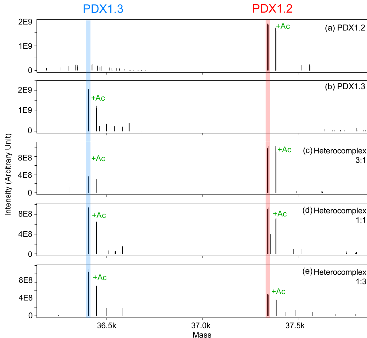
Supplementary Figure 5. Deconvoluted mass spectra of denatured intact PDX proteins for (a) PDX 1.2, (b) PDX 1.3, (c) heterocomplex 3:1, (d) heterocomplex 1:1, and (e) heterocomplex 1:3. About half of the protein show additional peak due to acetylation at the protein N-terminus. In all homomeric PDX1.2 and PDX1.3 samples and all three co-expressed samples, roughly half of the protein population was acetylated. These modifications, which are incorporated in the protein during its synthesis by ribosome-bound N-terminal acetyltransferases (NATs), are the most abundant, especially in higher eukaryotes ( Arnesen, T. Towards a functional understanding of protein. N-terminal acetylation. PLoS Biol 9, e1001074, doi:10.1371/journal.pbio.1001074 (2011) ). In general, such acetyl modifications are associated with various protein degradation and stabilization mechanisms inside the cell ( Hwang, C. S., Shemorry, A. & Varshavsky, A. N-terminal acetylation of cellular proteins creates specific degradation signals. Science 327, 973-977, doi:10.1126/science.1183147 (2010) ). Since no preferential acetylation profile was found across the samples, these modifications are likely irrelevant to PLP regulation itself.
